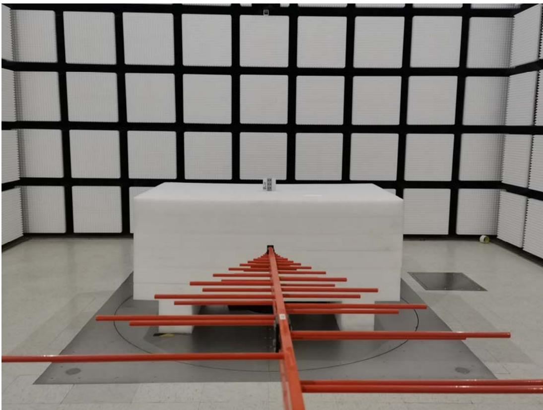
Radiated Emission Below 1GHz View- WS136-915M
