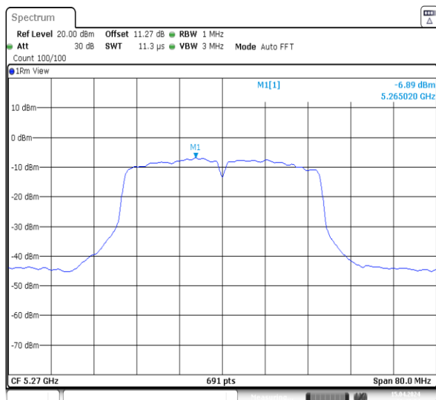
11N40MIMO-Ant1-5270-PASS
