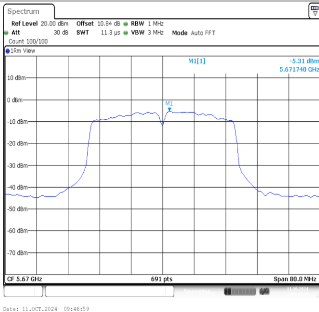
11AC40MIMO-Ant1-5670-PASS
