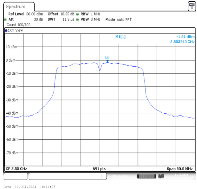
11AC40MIMO-Ant2-5550-PASS
