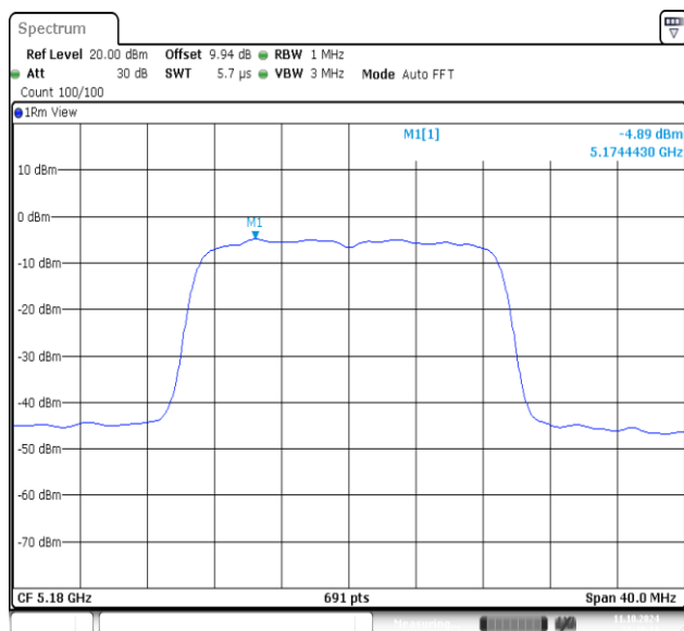
11N20MIMO-Ant1-5180-PASS
