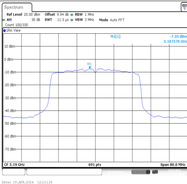
11AX40MIMO-Ant1-5190-PASS
