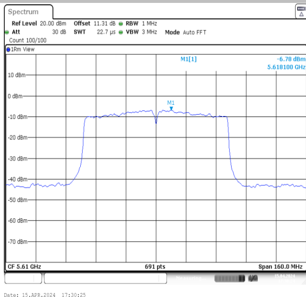
11AC80MIMO-Ant1-5610-PASS
