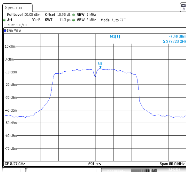
11N40MIMO-Ant2-5270-PASS
