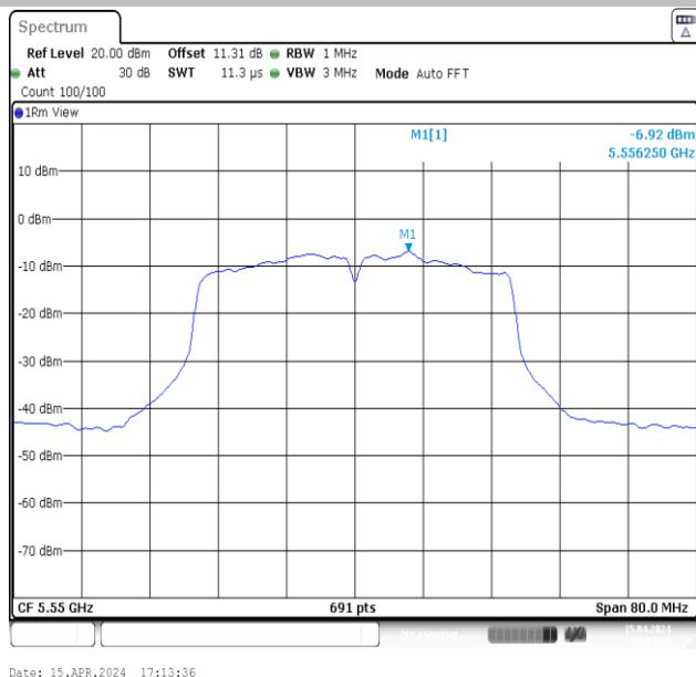
11N40MIMO-Ant1-5550-PASS
