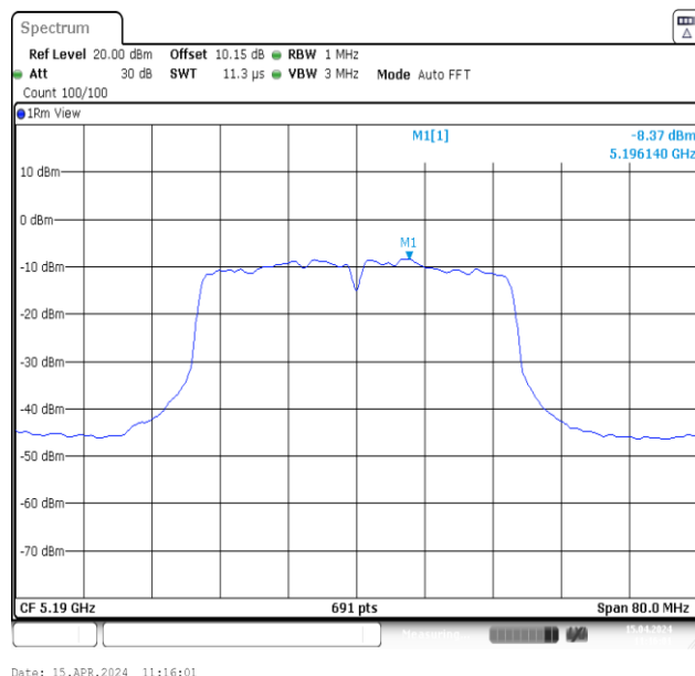
11N40MIMO-Ant2-5190-PASS
