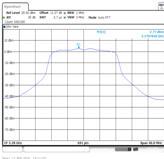
11A-Ant1-5280-PASS
