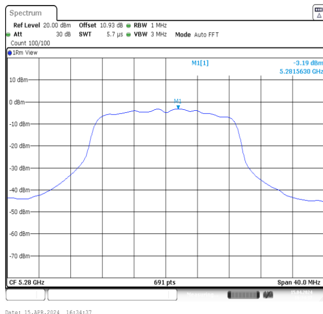
11N20MIMO-Ant2-5280-PASS
