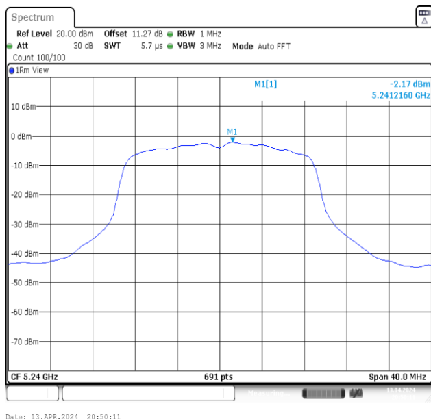
11N20MIMO-Ant1-5240-PASS
