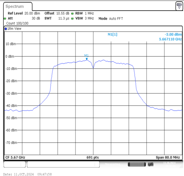
11AC40MIMO-Ant2-5670-PASS
