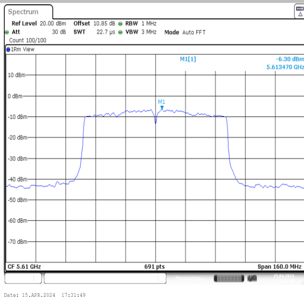
11AC80MIMO-Ant2-5610-PASS
