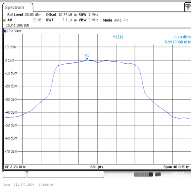
11AC20MIMO-Ant1-5240-PASS
