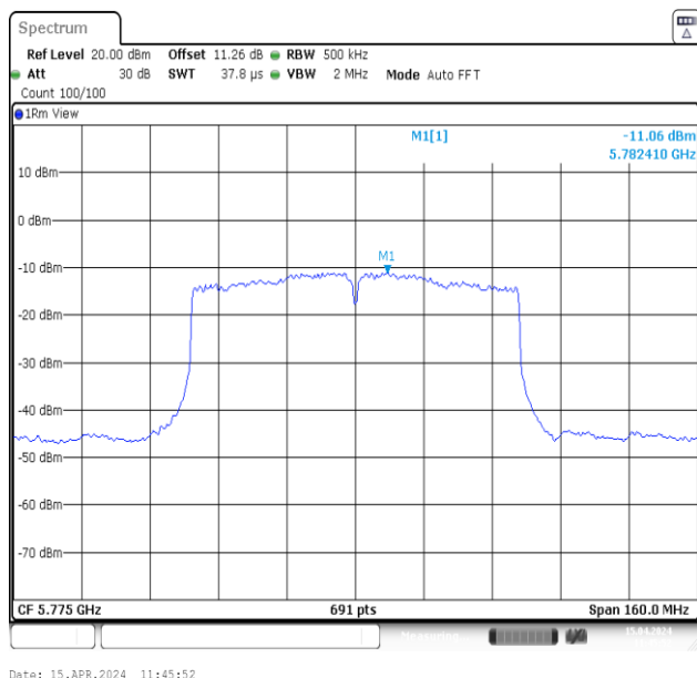
11AC80MIMO-Ant1-5775-PASS
