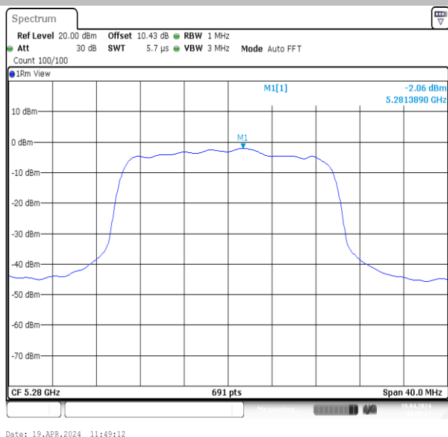
11AX20MIMO-Ant2-5280-PASS
