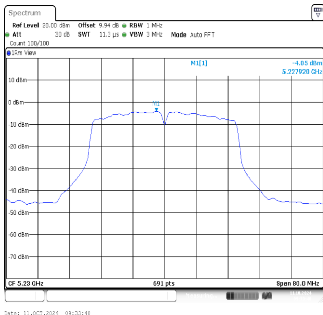
11AC40MIMO-Ant1-5230-PASS
