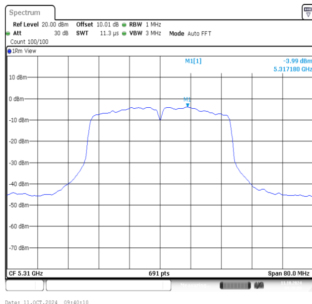
11AC40MIMO-Ant2-5310-PASS
