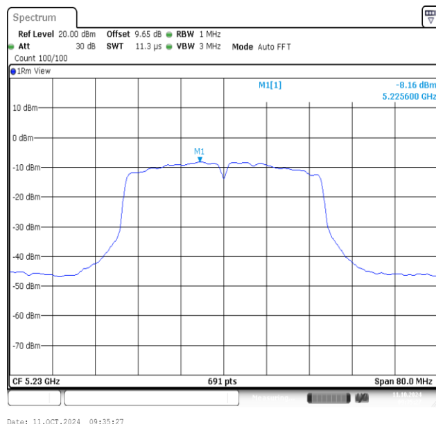
11AC40MIMO-Ant2-5230-PASS
