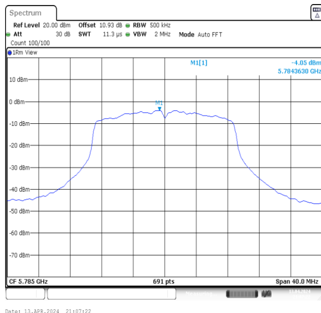
11N20MIMO-Ant2-5785-PASS
