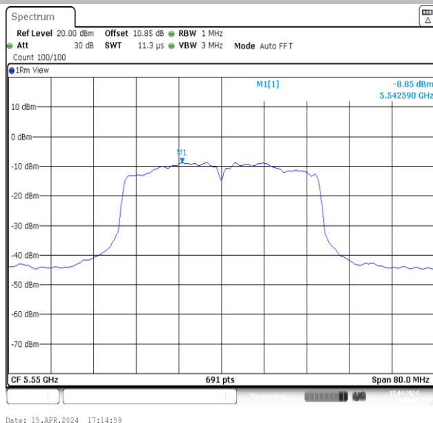
11N40MIMO-Ant2-5550-PASS
