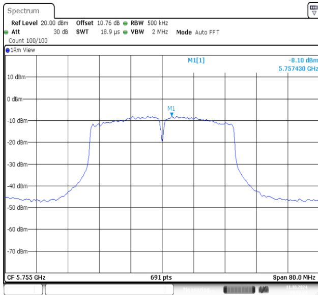
11AC40MIMO-Ant1-5755-PASS
