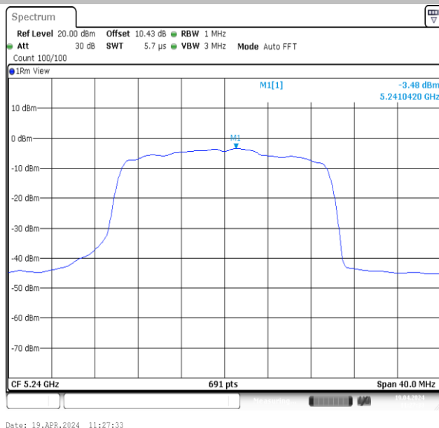
11AX20MIMO-Ant2-5240-PASS
