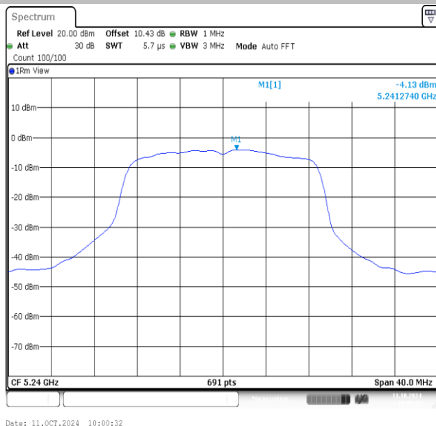
11AC20MIMO-Ant2-5240-PASS
