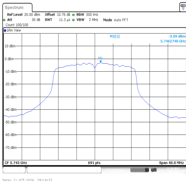
11AC20MIMO-Ant1-5745-PASS
