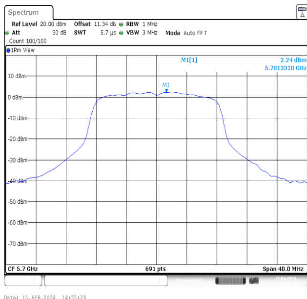
11A-Ant1-5700-PASS
