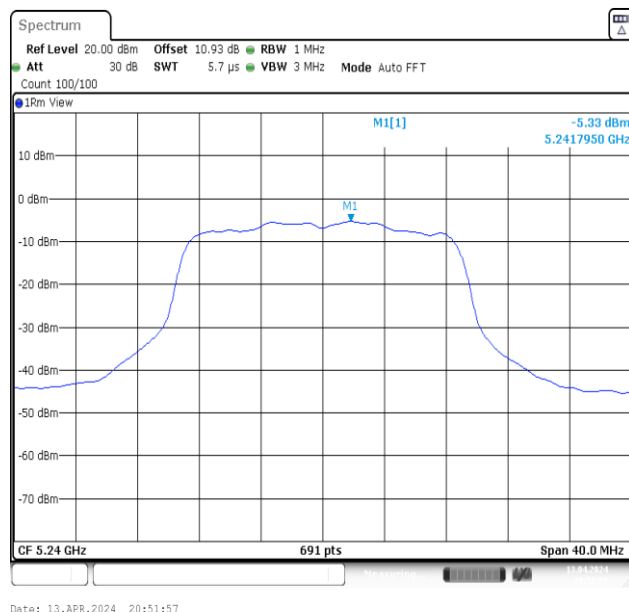
11N20MIMO-Ant2-5240-PASS
