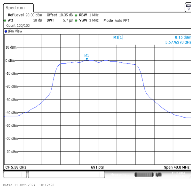
11AC20MIMO-Ant2-5580-PASS
