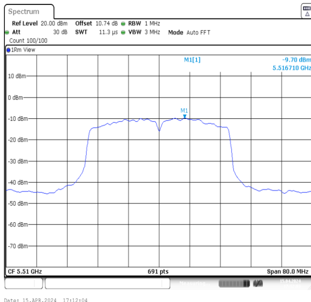
11N40MIMO-Ant2-5510-PASS
