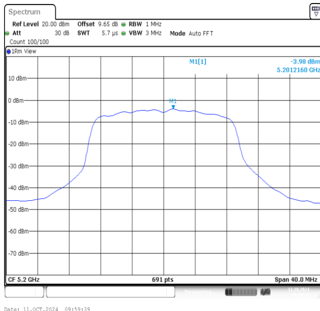
11AC20MIMO-Ant2-5200-PASS
