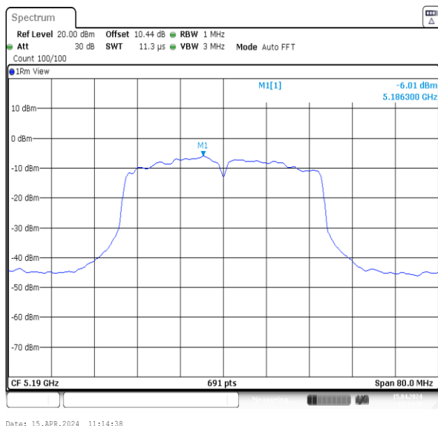
11N40MIMO-Ant1-5190-PASS
