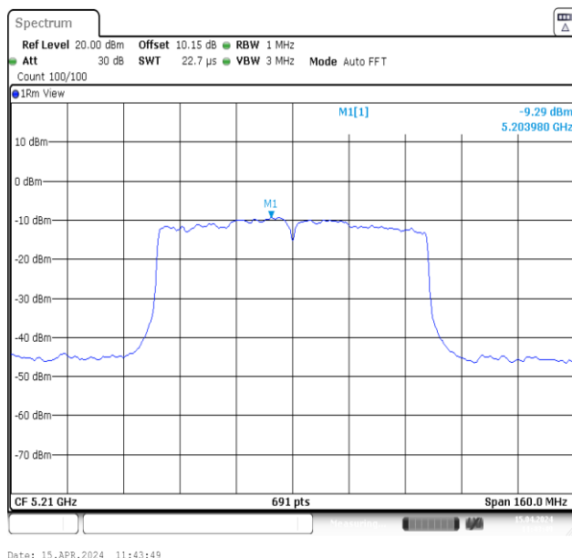
11AC80MIMO-Ant2-5210-PASS
