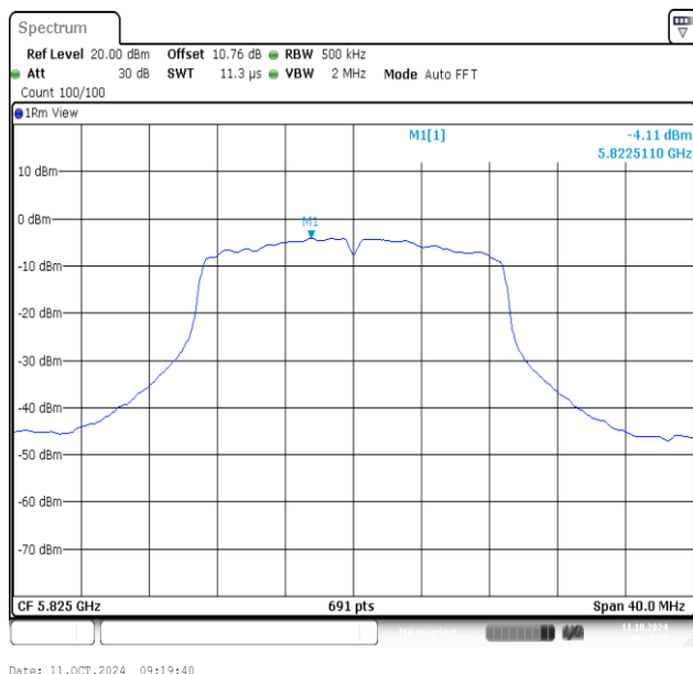
11AC20MIMO-Ant1-5825-PASS
