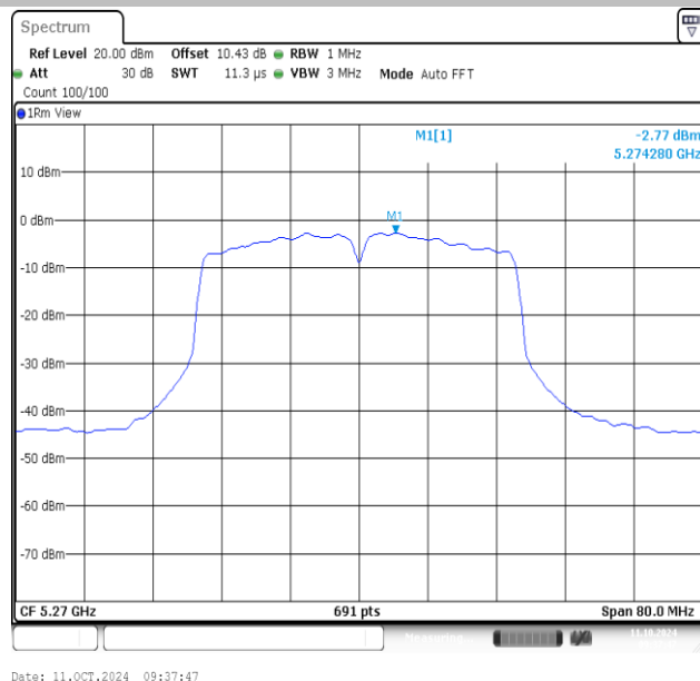
11AC40MIMO-Ant2-5270-PASS
