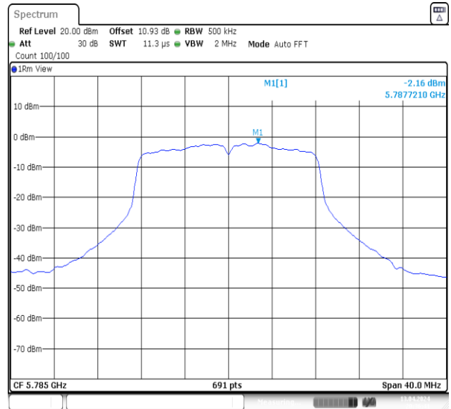
11A-Ant2-5785-PASS
