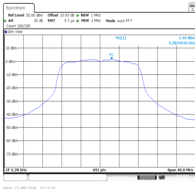
11A-Ant2-5280-PASS
