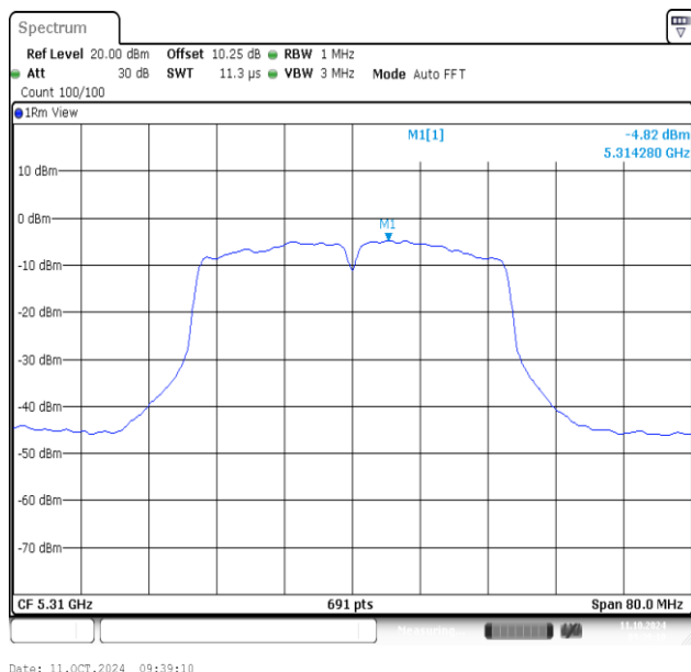
11AC40MIMO-Ant1-5310-PASS
