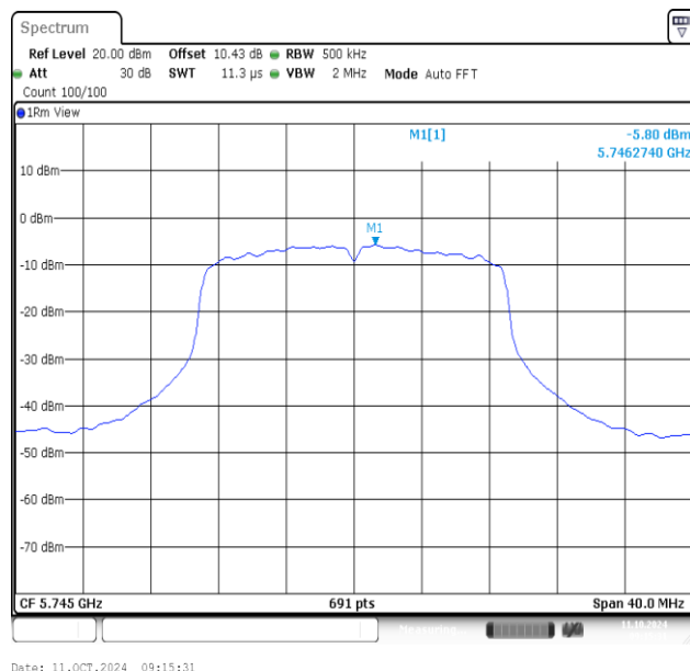
11AC20MIMO-Ant2-5745-PASS
