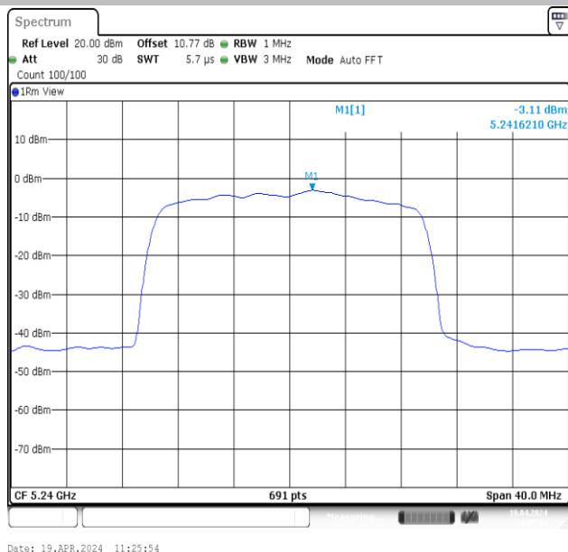
11AX20MIMO-Ant1-5240-PASS
