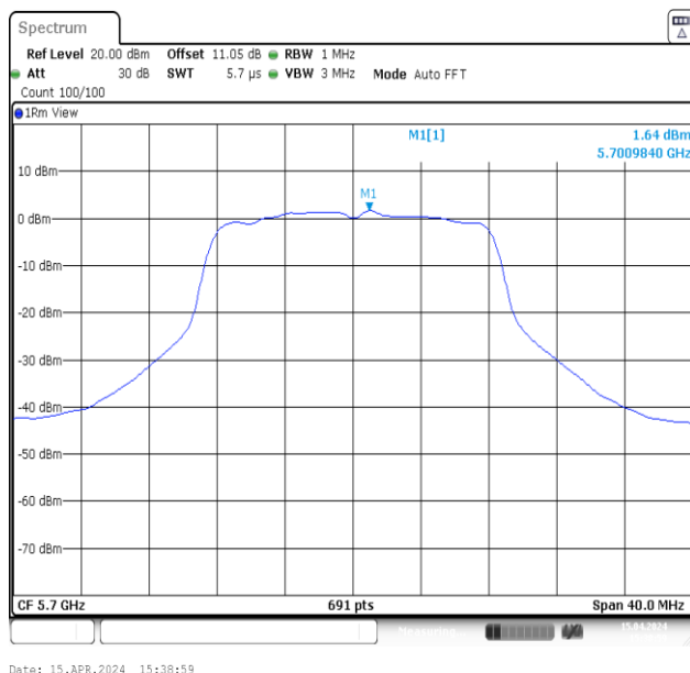
11A-Ant2-5700-PASS
