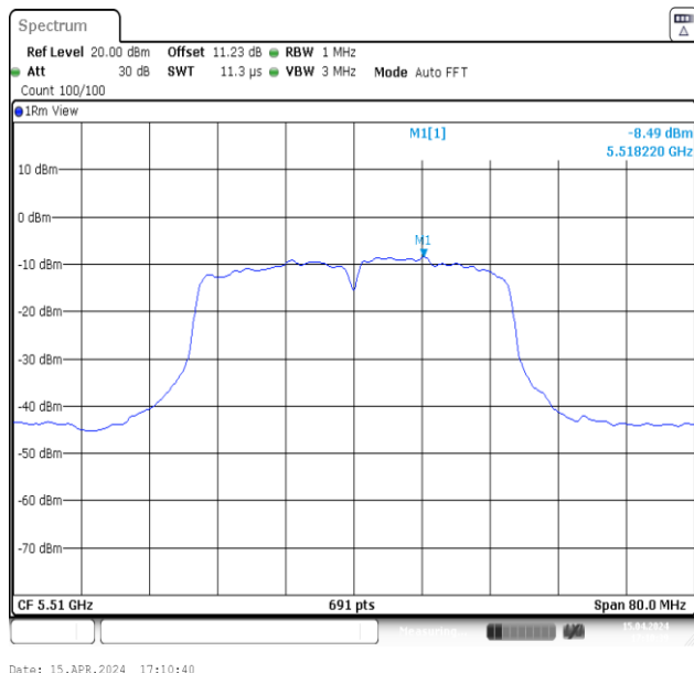
11N40MIMO-Ant1-5510-PASS
