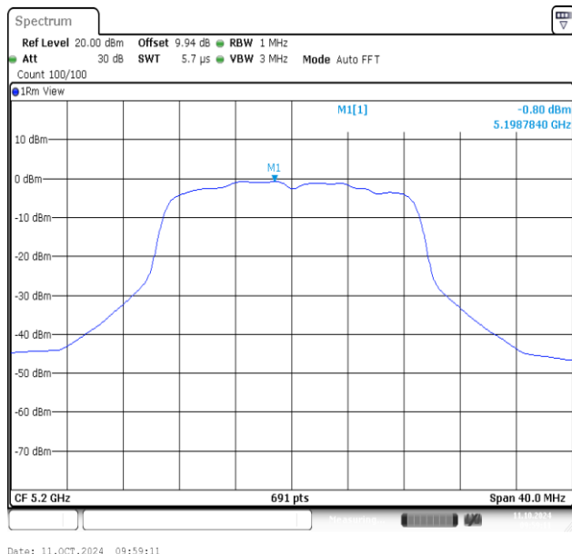
11AC20MIMO-Ant1-5200-PASS
