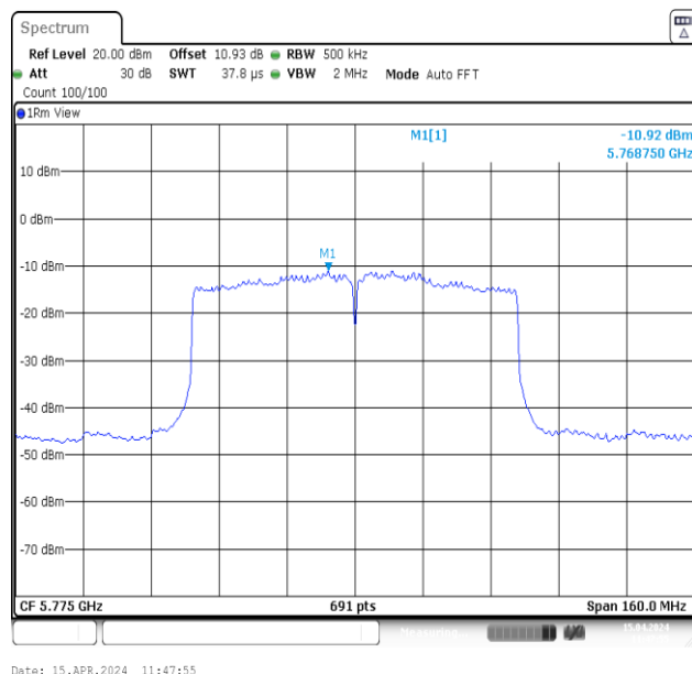
11AC80MIMO-Ant2-5775-PASS
