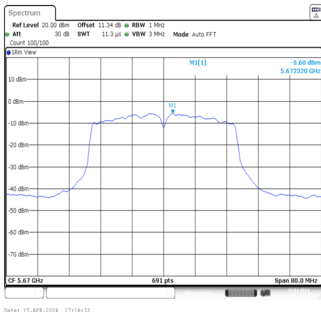
11N40MIMO-Ant1-5670-PASS
