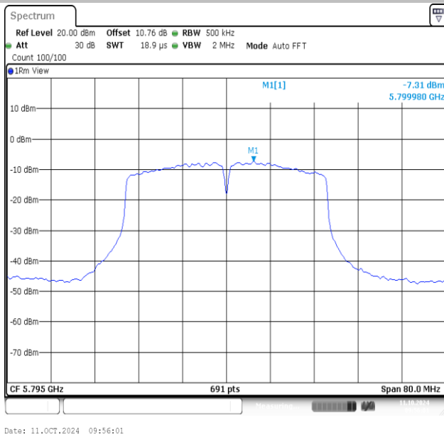
11AC40MIMO-Ant1-5795-PASS
