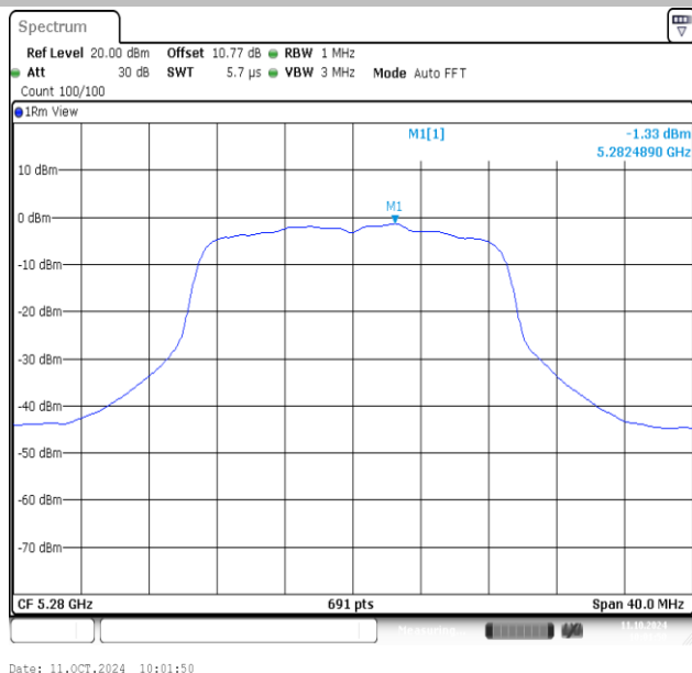
11AC20MIMO-Ant1-5280-PASS
