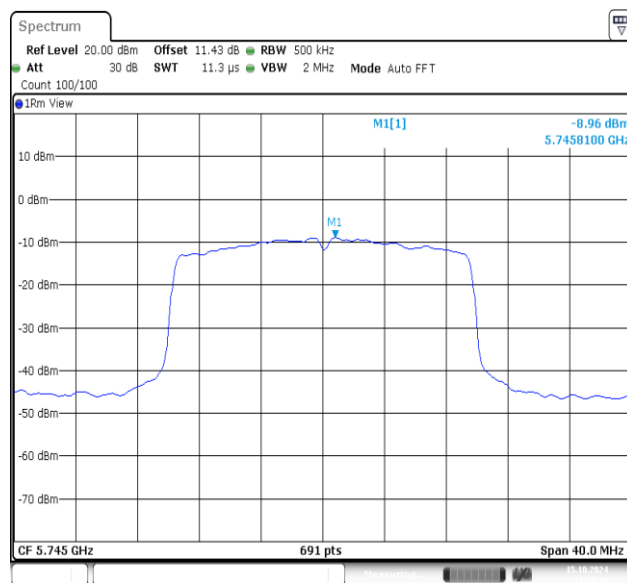
11AX20MIMO-Ant2-5745-PASS
