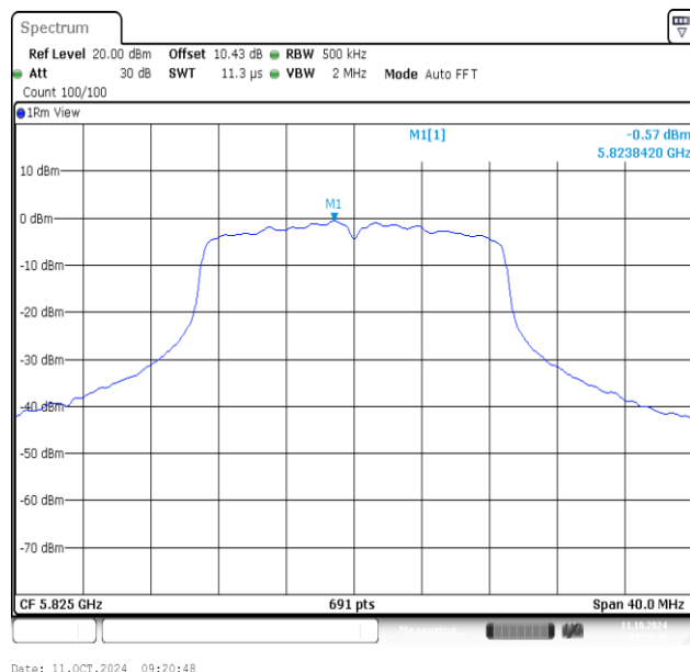
11AC20MIMO-Ant2-5825-PASS
