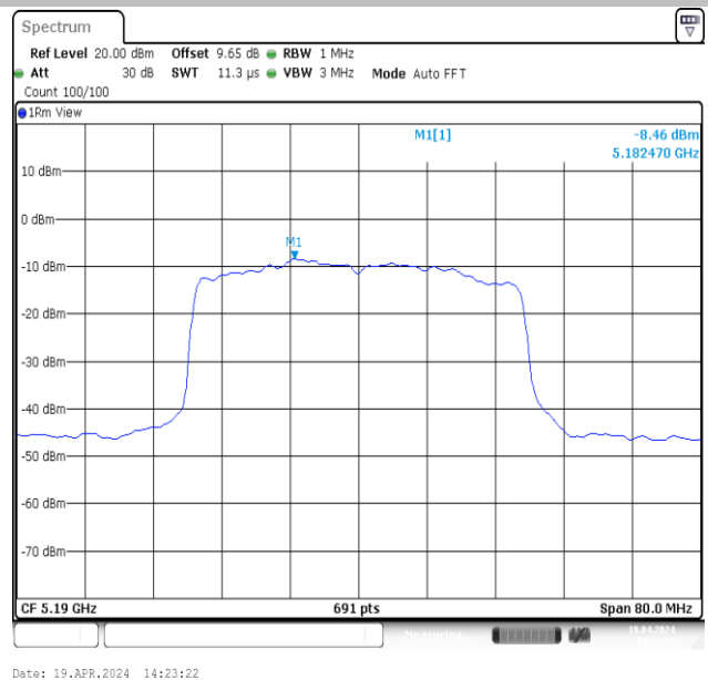
11AX40MIMO-Ant2-5190-PASS
