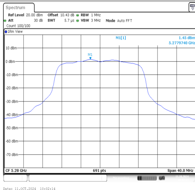
11AC20MIMO-Ant2-5280-PASS
