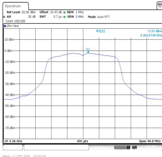
11AC20MIMO-Ant2-5260-PASS
