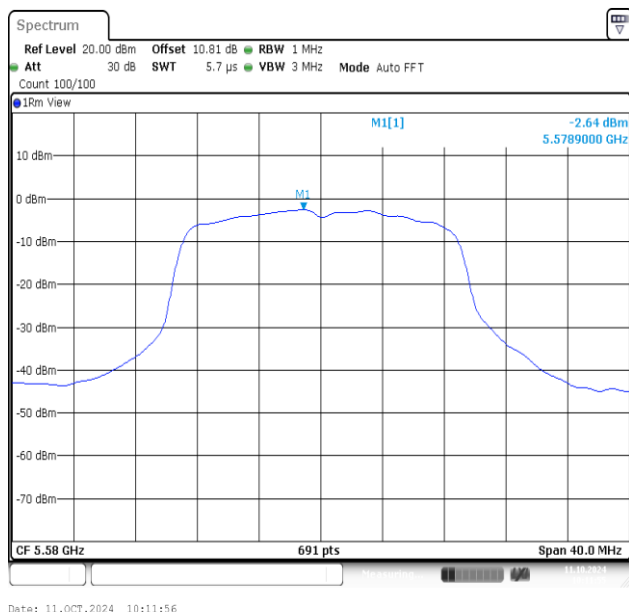
11AC20MIMO-Ant1-5580-PASS
