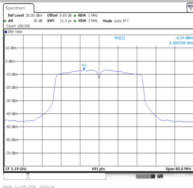
11AC40MIMO-Ant2-5190-PASS
