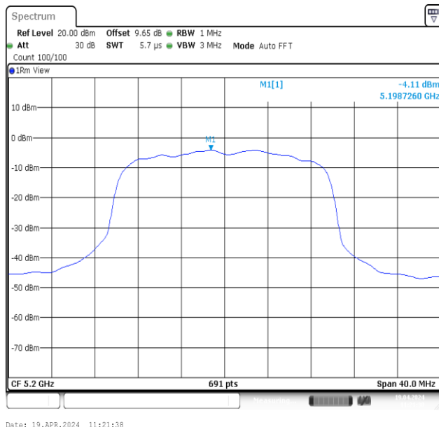
11AX20MIMO-Ant2-5200-PASS
