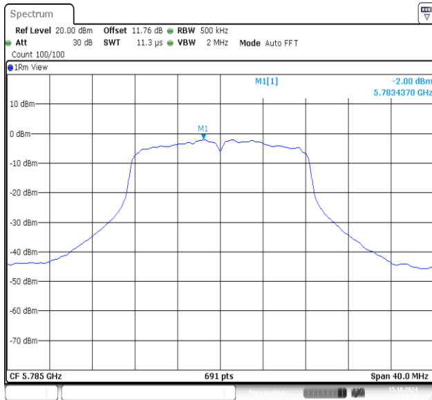
11A-Ant1-5785-PASS
