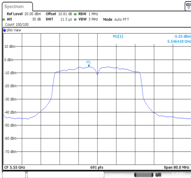
11AC40MIMO-Ant1-5550-PASS
