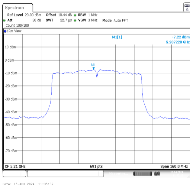
11AC80MIMO-Ant1-5210-PASS
