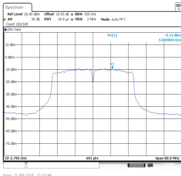
11N40MIMO-Ant2-5795-PASS
