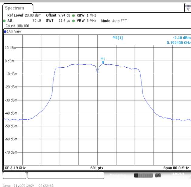
11AC40MIMO-Ant1-5190-PASS
