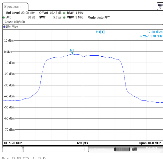
11AX20MIMO-Ant2-5260-PASS
