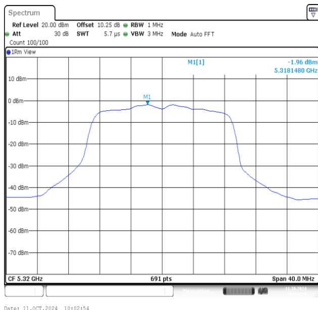
11AC20MIMO-Ant1-5320-PASS
