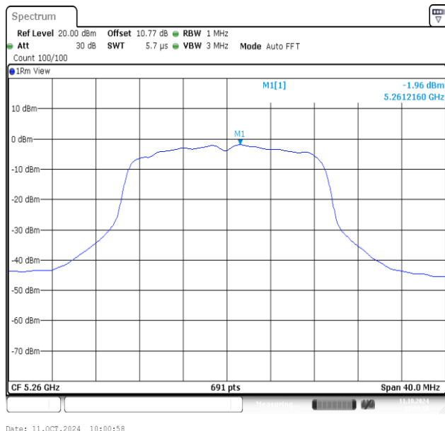
11AC20MIMO-Ant1-5260-PASS
