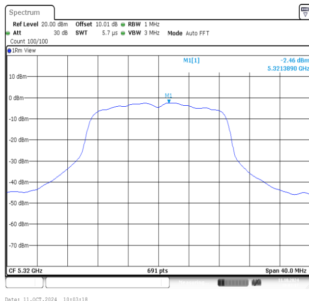
11AC20MIMO-Ant2-5320-PASS
