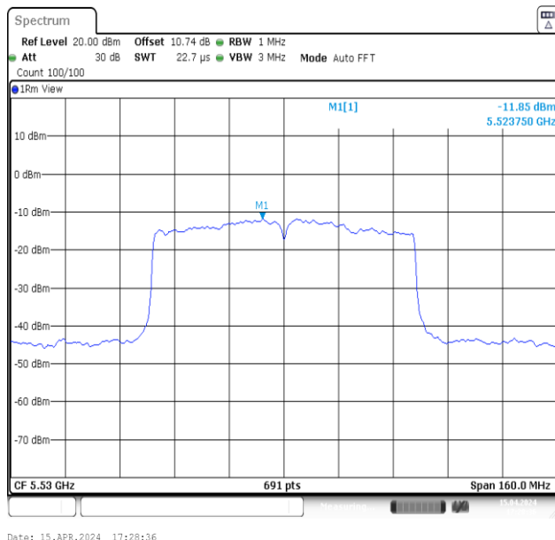
11AC80MIMO-Ant2-5530-PASS
