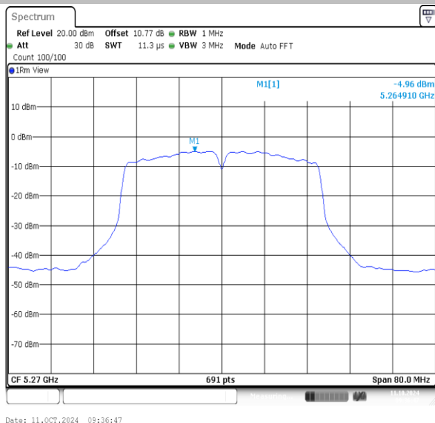
11AC40MIMO-Ant1-5270-PASS
