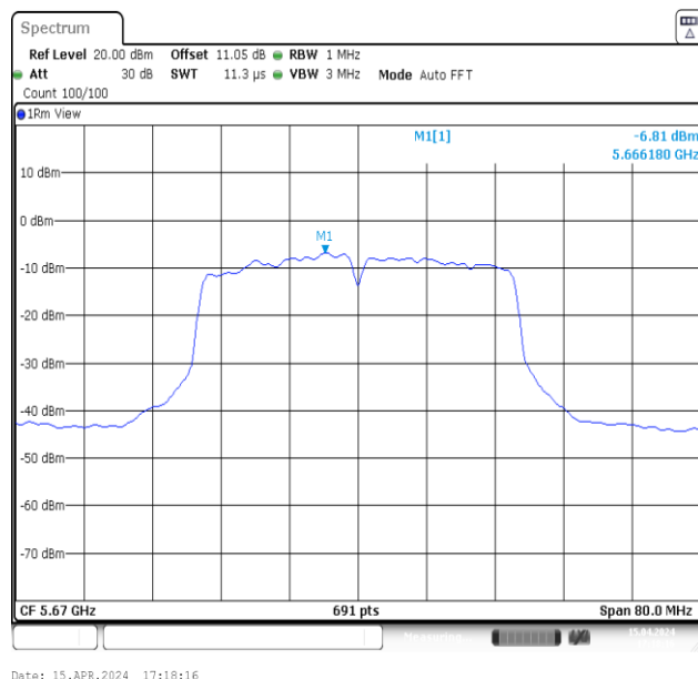
11N40MIMO-Ant2-5670-PASS
