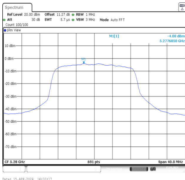
11N20MIMO-Ant1-5280-PASS
