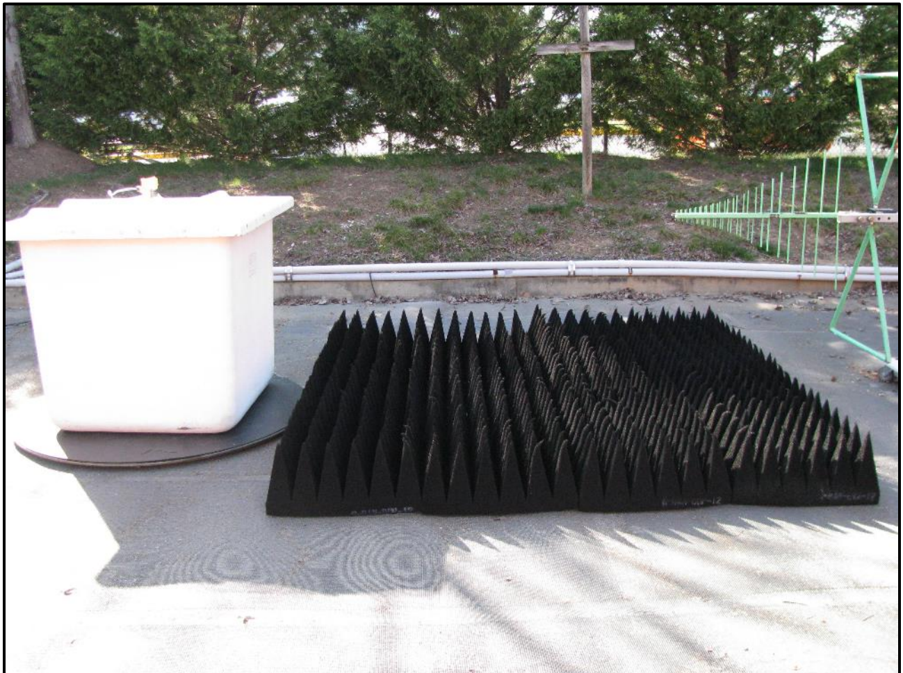
Photograph 59: Radiated Emissions – TC #6; Fiberglass Container, Front View
