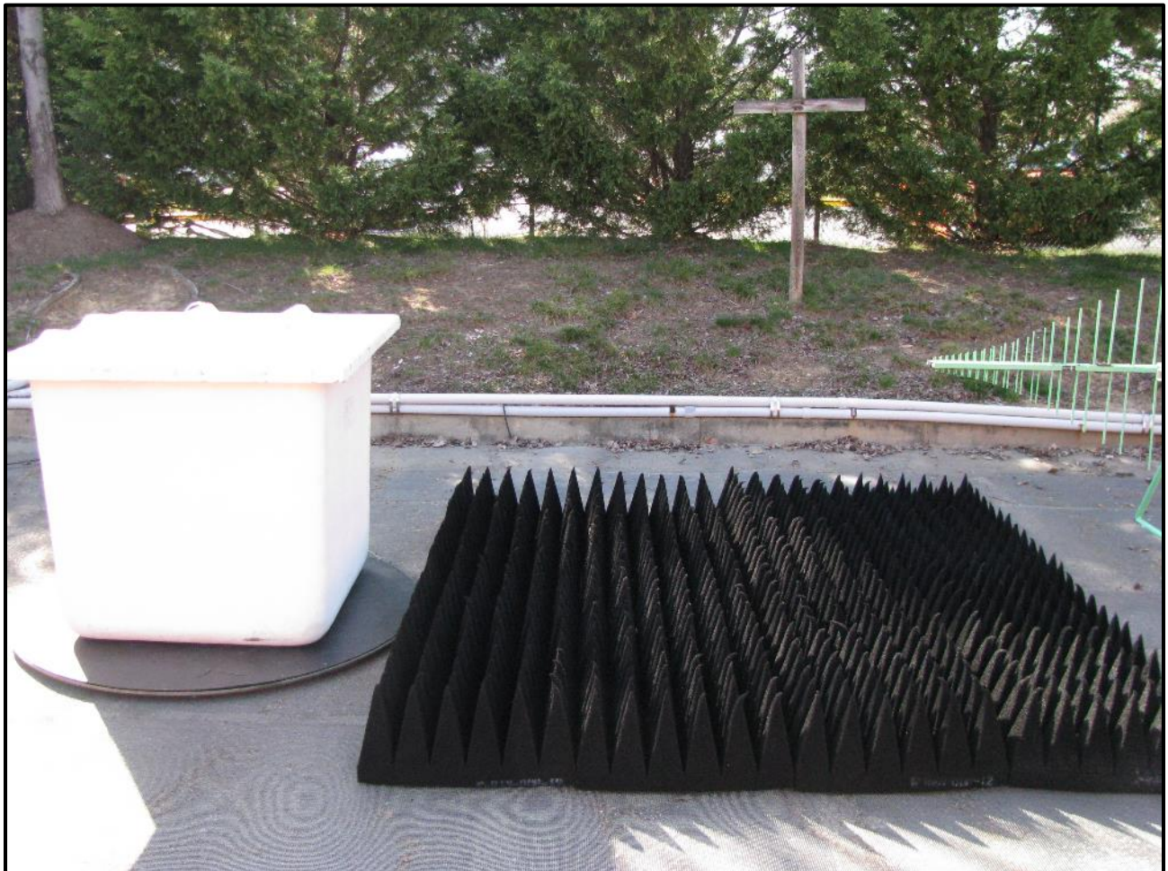
Photograph 63: Radiated Emissions – TC #8; Fiberglass Container, Front View
