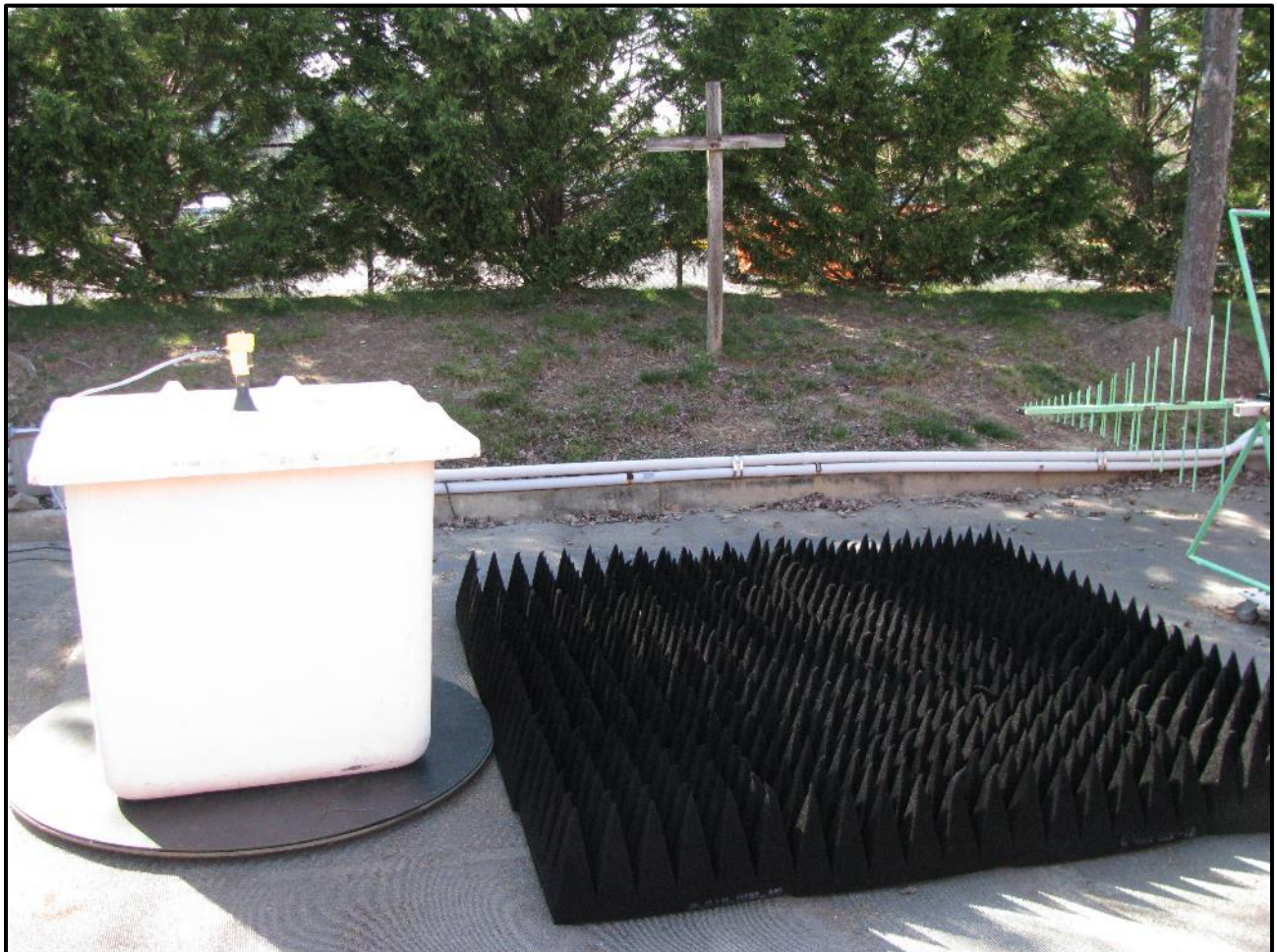
Photograph 49: Radiated Emissions – TC #1; Fiberglass Container, Front View
