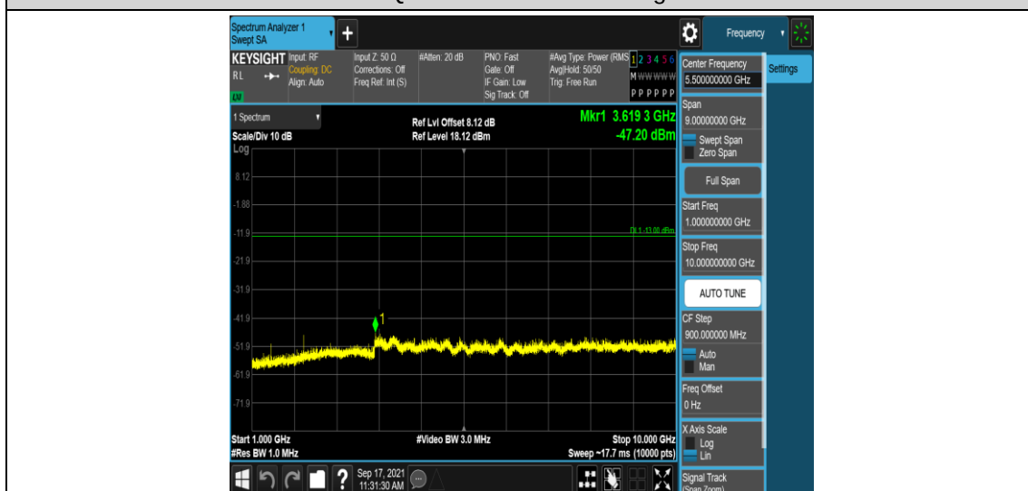
Band12-5MHz-16QAM-23035-1RB#0-Range4:1000~10000MHz
