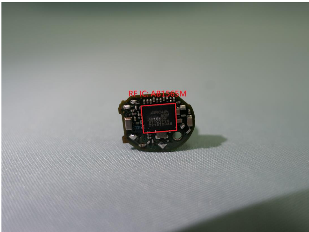
( 16 ) EUT Photo_Right Ear
