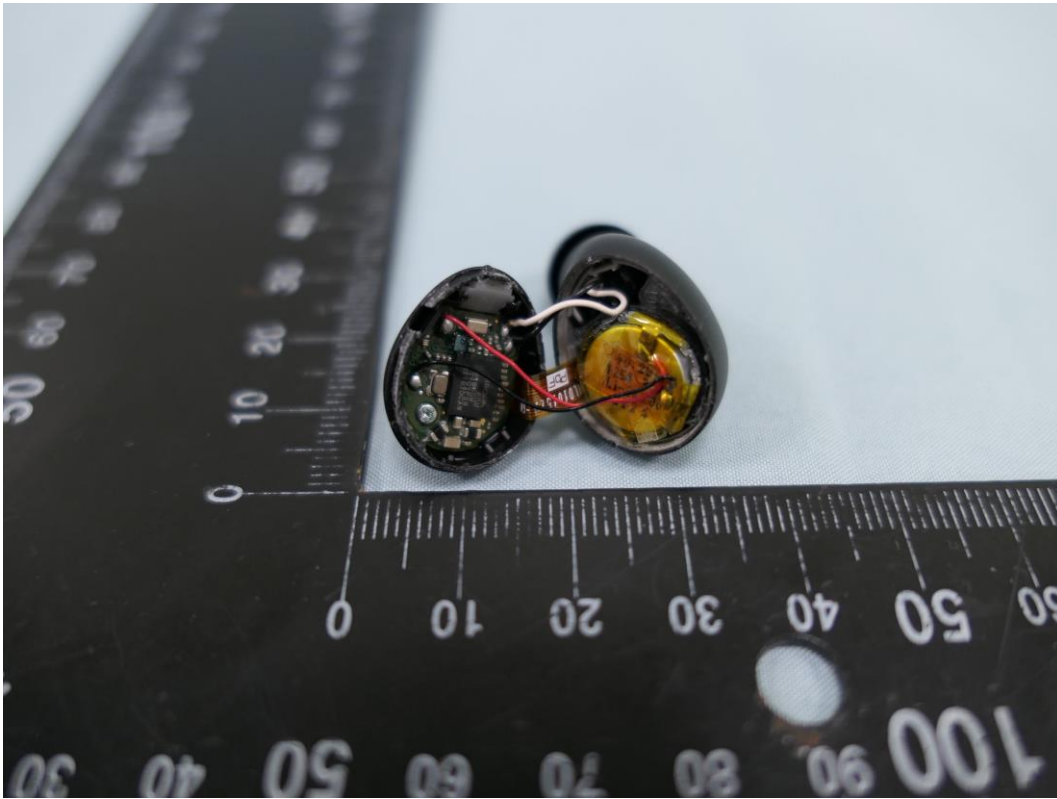
( 12 ) EUT Photo_Right Ear
