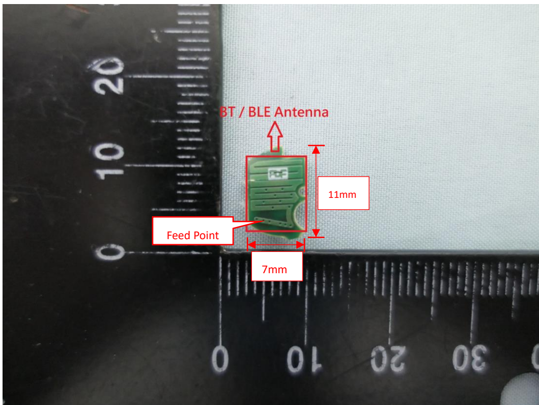
( 10 ) EUT Photo_Left Ear
