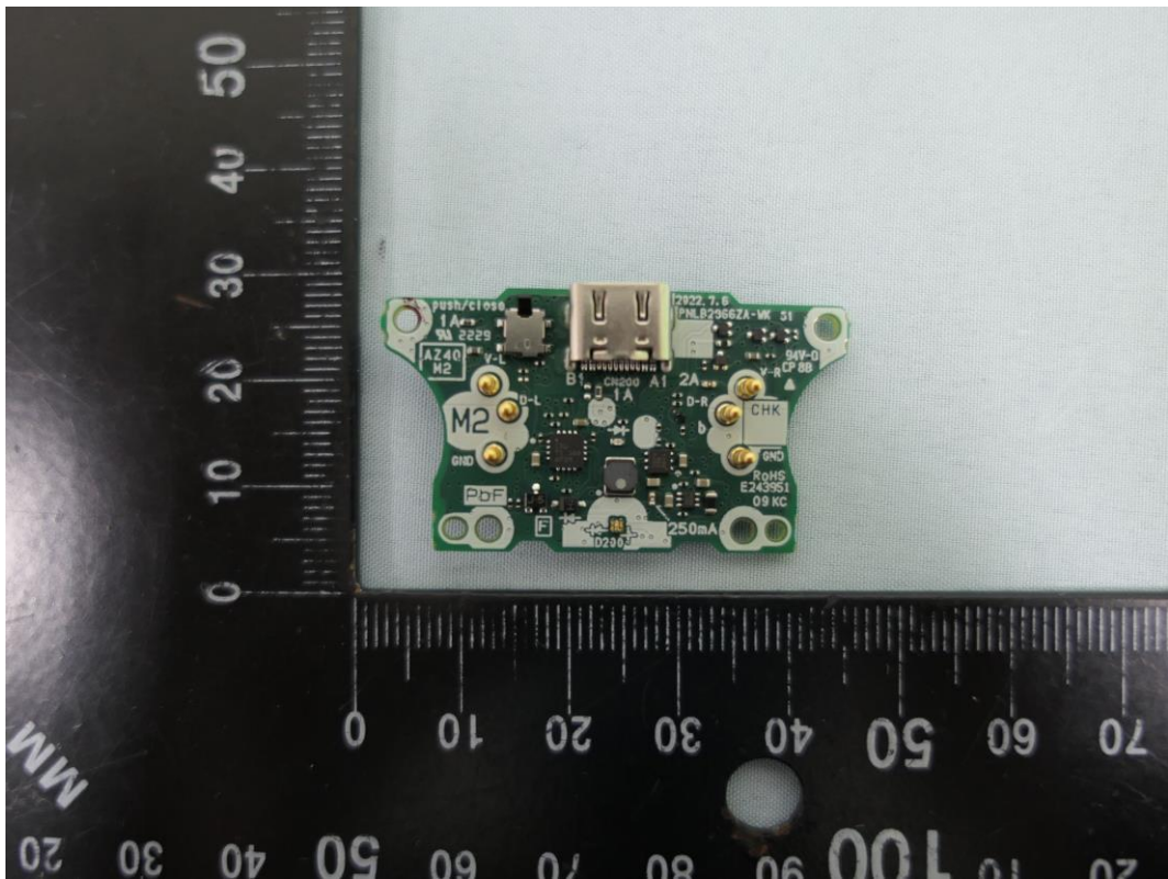
( 28 ) EUT Photo_Charging Box
