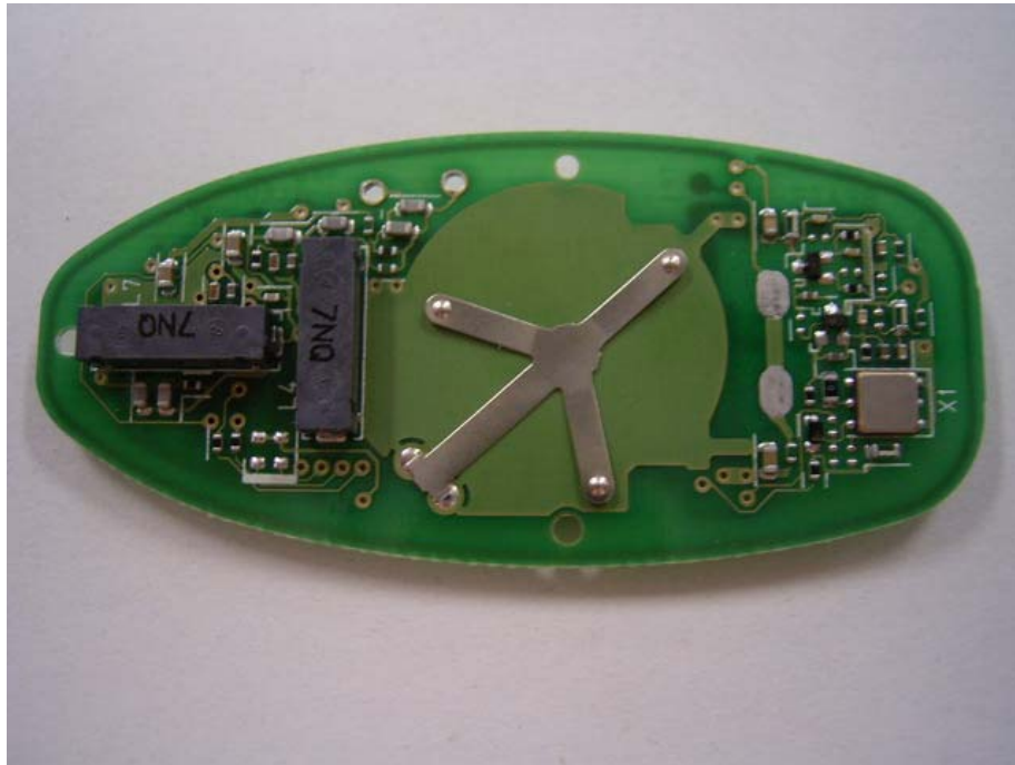
Side B of PWB
