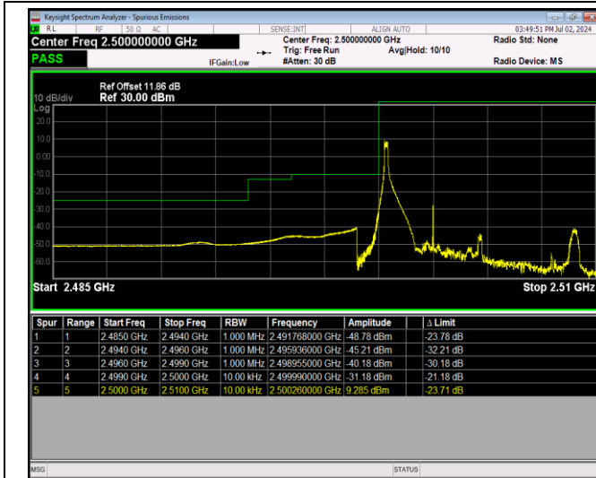
Band7-5MHz-64QAM-20775-25RB#0
