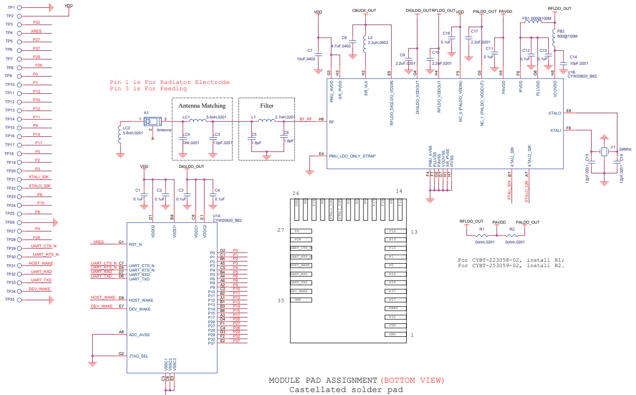
Figure 8. CYBT-2x305x-02 Schematic Diagram
