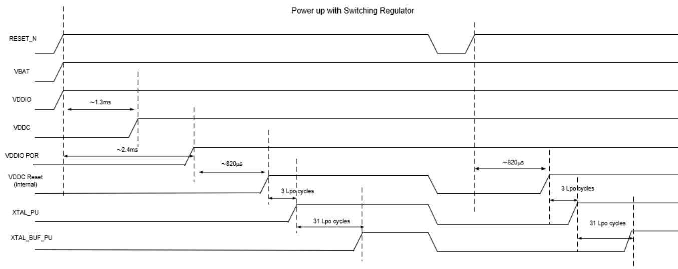
Figure 10. Reset Timing
