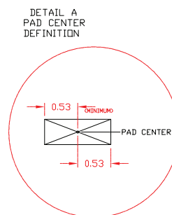
Top View (Seen on Host PCB)
