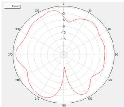
Phi=0 Freq=2400MHz
