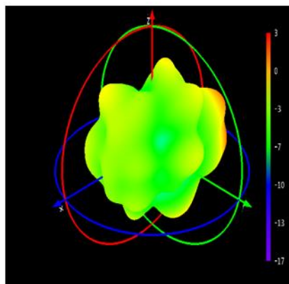
Phi=0 Freq=2400MHz
