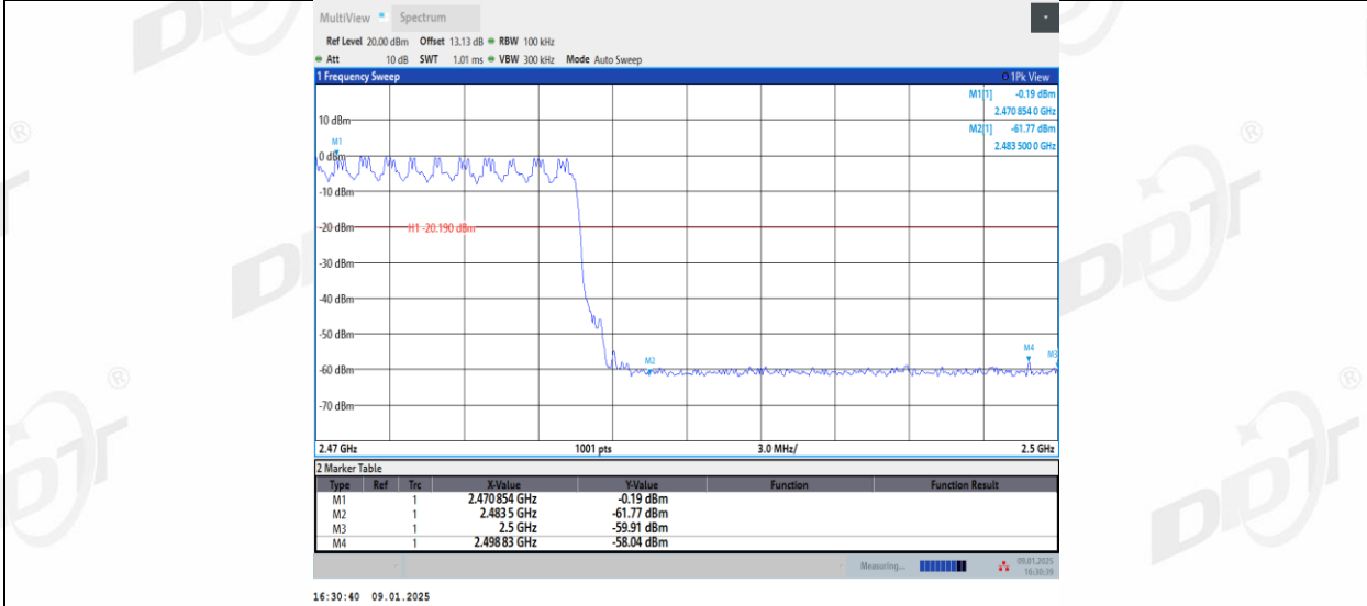
2DH5_Right side_High_Hop_2480
