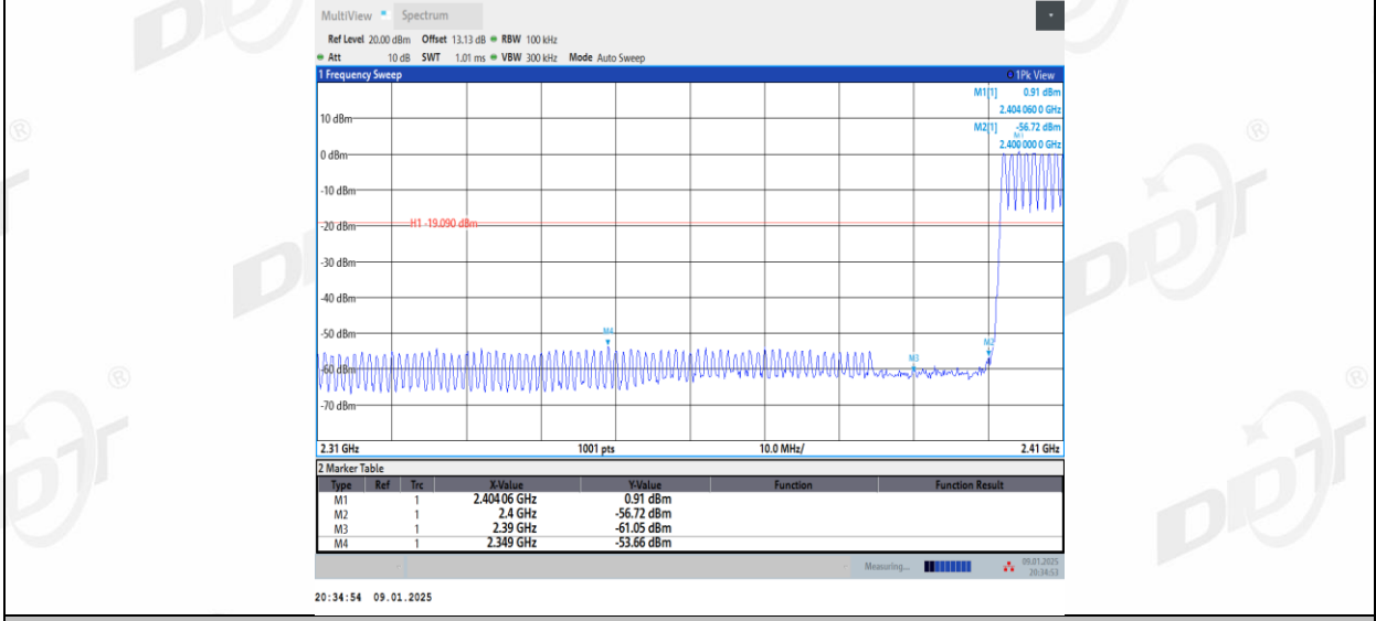
DH5_Left side_High_Hop_2480
