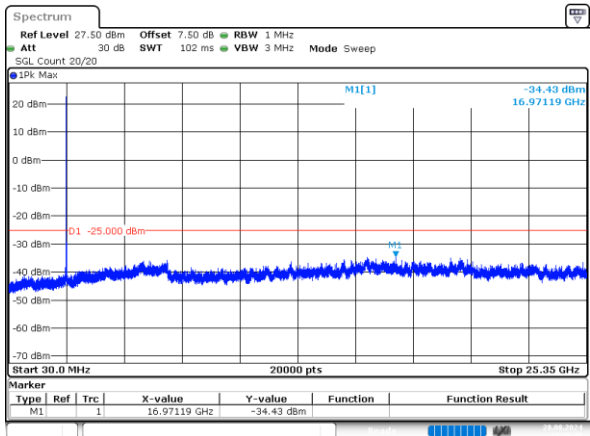
15MHz_Middle_QPSK_1@0
