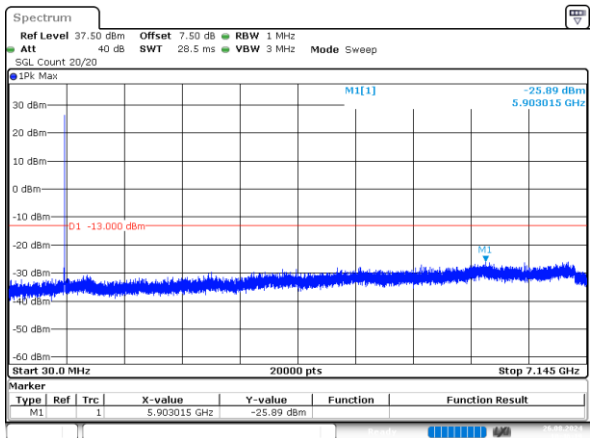
3MHz_High_QPSK_1@0
