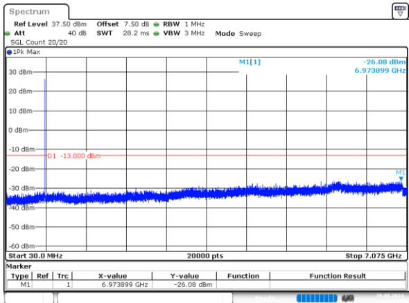
1.4MHz_Middle_QPSK_1@0
