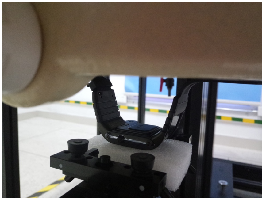
Back Side(Test distance: 5mm, Thickness of DUT: 15mm)
