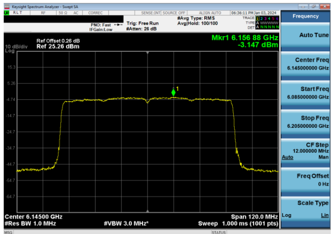
Plot 7-492. LPI Power Spectral Density Plot Antenna WF2a (80MHz 802.11ax RU996 (UNII Band 5) – Ch. 39)
