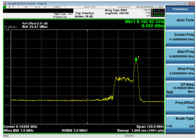
Plot 7-491. LPI Power Spectral Density Plot Antenna WF2a (80MHz 802.11ax RU26 (UNII Band 5) – Ch. 39)
