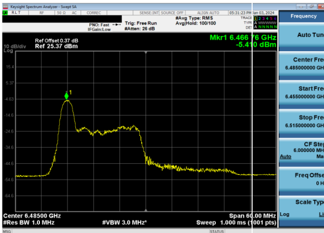
Plot 7-501. LPI Power Spectral Density Plot Antenna WF2a (40MHz) 802.11ax RU26 (UNII Band 6) – Ch. 107)
