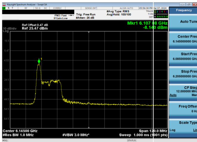
Plot 7-489. LPI Power Spectral Density Plot Antenna WF2a (80MHz 802.11ax RU26 (UNII Band 5) – Ch. 39)
