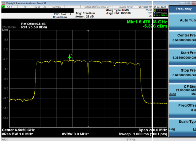
Plot 7-512. LPI Power Spectral Density Plot Antenna WF2a (160MHz 802.11ax RU996x2 (UNII Band 6) – Ch. 111)
