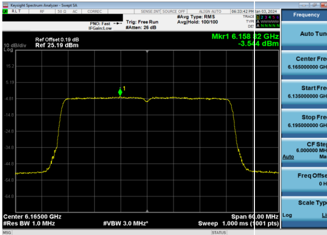
Plot 7-488. LPI Power Spectral Density Plot Antenna WF2a (40MHz 802.11ax RU484 (UNII Band 5) – Ch. 43)
