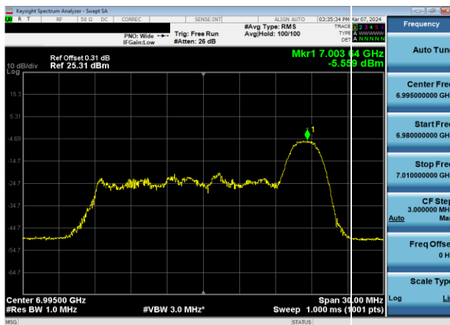
Plot 7-467. LPI Power Spectral Density Plot Antenna WF7a (20MHz 802.11ax RU26 (UNII Band 8) – Ch. 209)
