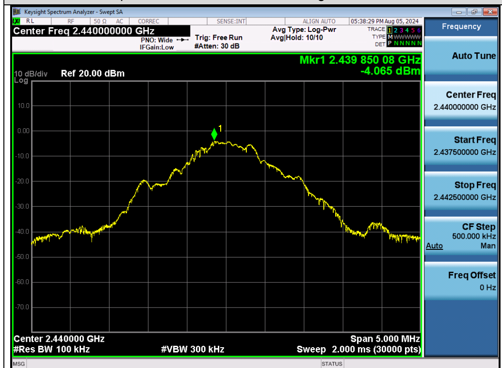
Test_Graph_2.4G_ANT1_2440_GFSK_Reference Level
