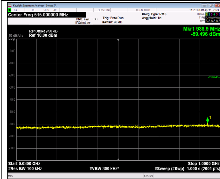
Band66_20MHz_QPSK_132572_1RB#0_30~1000_30~1000
