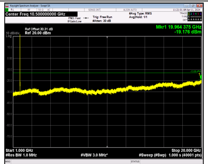
Band66_20MHz_QPSK_132072_1RB#0_1000~20000_1000~20000
