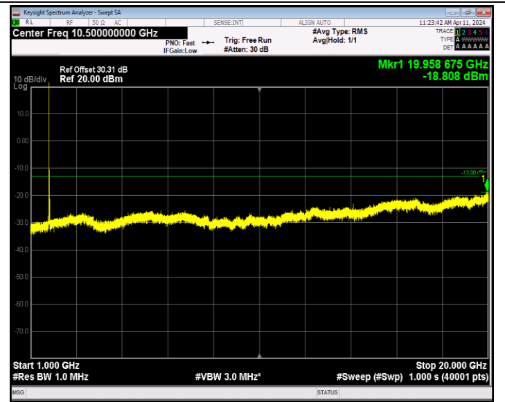
Band66_20MHz_16QAM_132572_1RB#0_1000~20000_1000~2000
