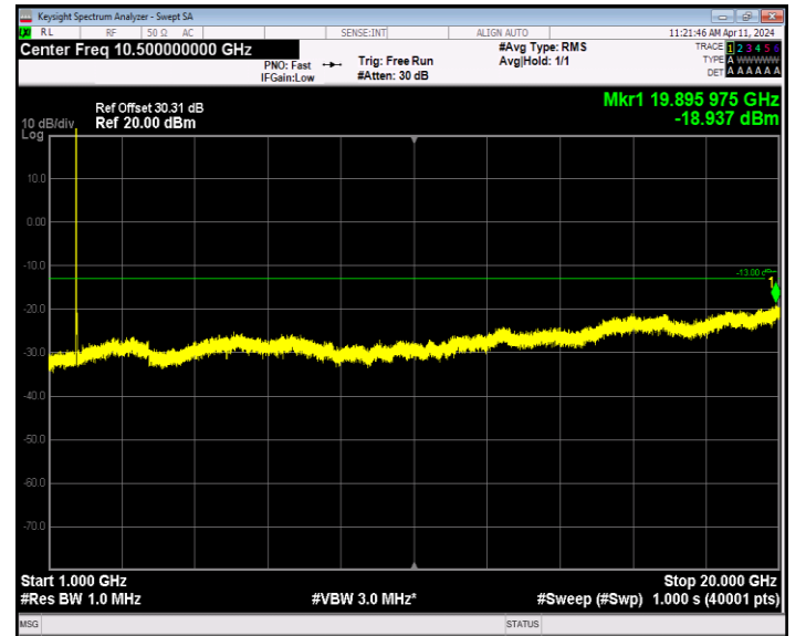
Band66_20MHz_64QAM_132072_1RB#0_1000~20000_1000~2000
