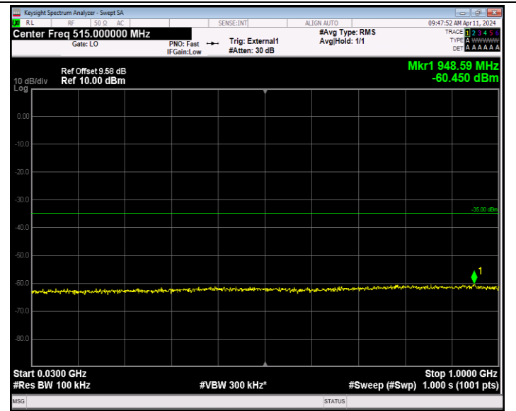
Band41_20MHz_64QAM_41490_1RB#0_30~1000_30~1000
