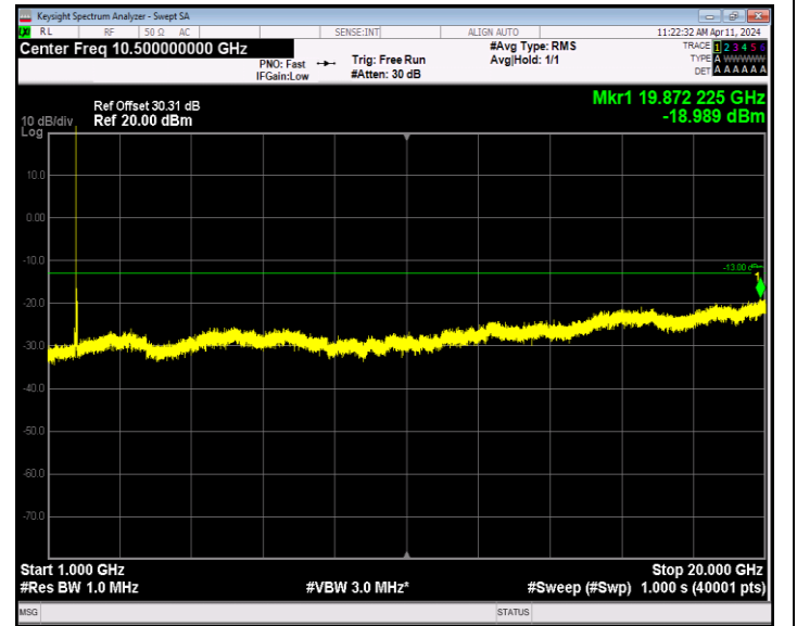
Band66_20MHz_16QAM_132322_1RB#0_1000~20000_1000~20000
