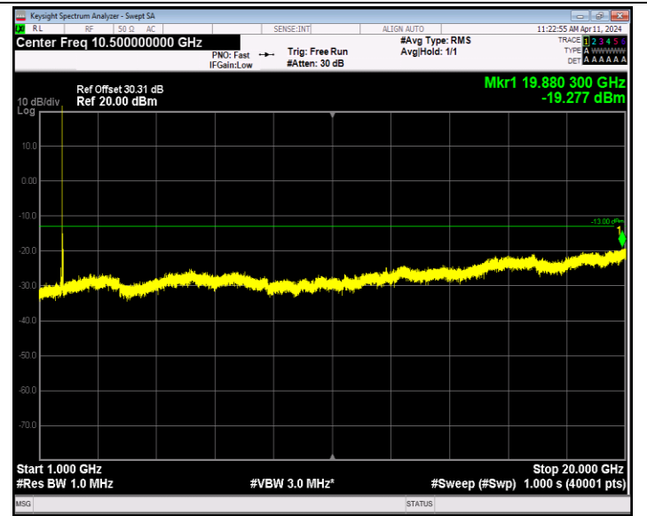
Band66_20MHz_64QAM_132322_1RB#0_1000~20000_1000~20000
