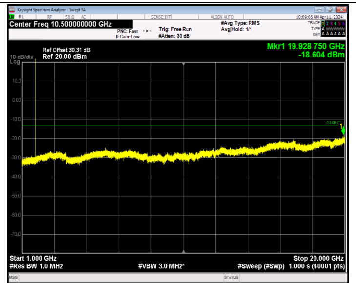
Band66_1.4MHz_64QAM_132665_1RB#0_1000~20000_1000~20000
