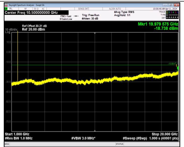
Band66_1.4MHz_64QAM_131979_1RB#0_1000~20000_1000~20000
