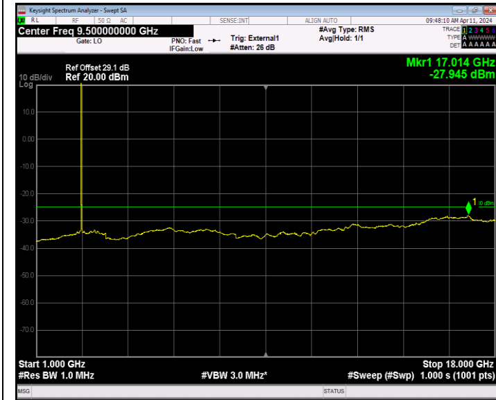
Band41_20MHz_64QAM_41490_1RB#0_1000~18000_1000~18000
