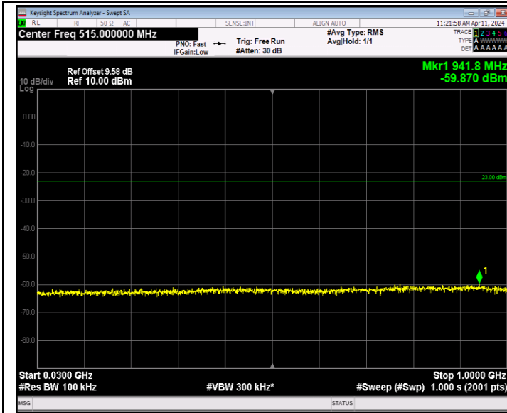
Band66_20MHz_QPSK_132322_1RB#0_30~1000_30~1000
