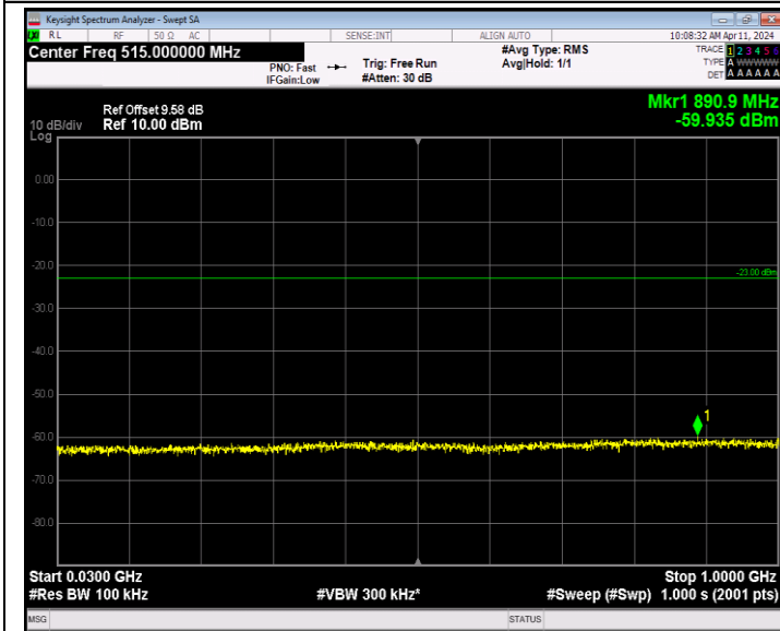
Band66_1.4MHz_16QAM_132665_1RB#0_30~1000_30~1000
