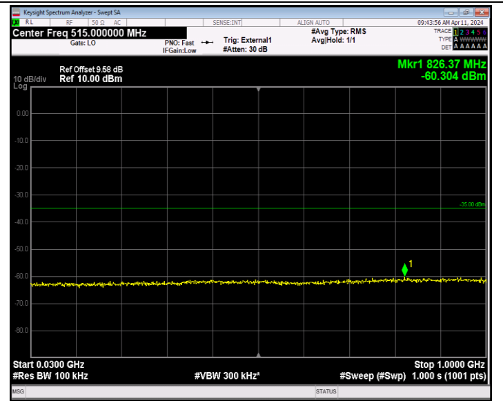
Band41_20MHz_16QAM_40620_1RB#0_30~1000_30~1000
