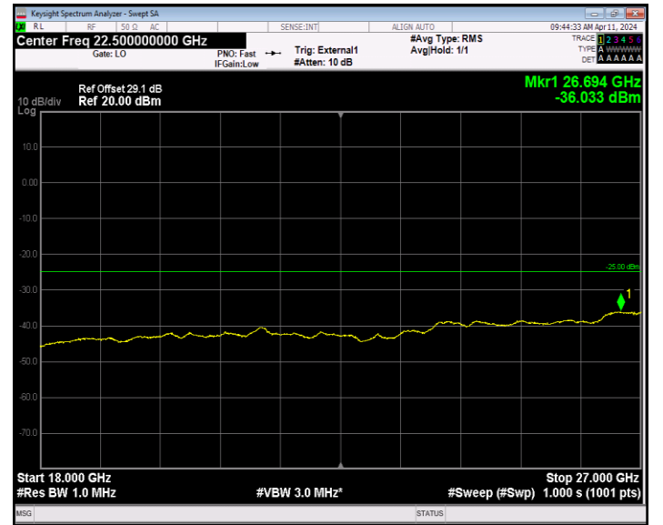
Band41_20MHz_16QAM_40620_1RB#0_18000~27000_18000~27000
