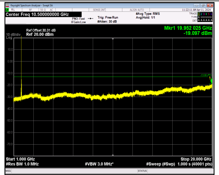
Band66_20MHz_QPSK_132322_1RB#0_1000~20000_1000~2000
