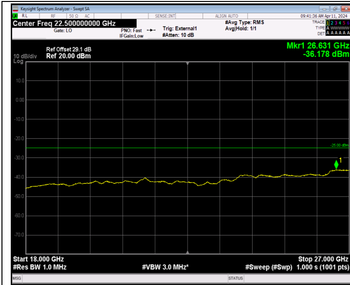
Band41_20MHz_16QAM_39750_1RB#0_18000~27000_18000~27000
