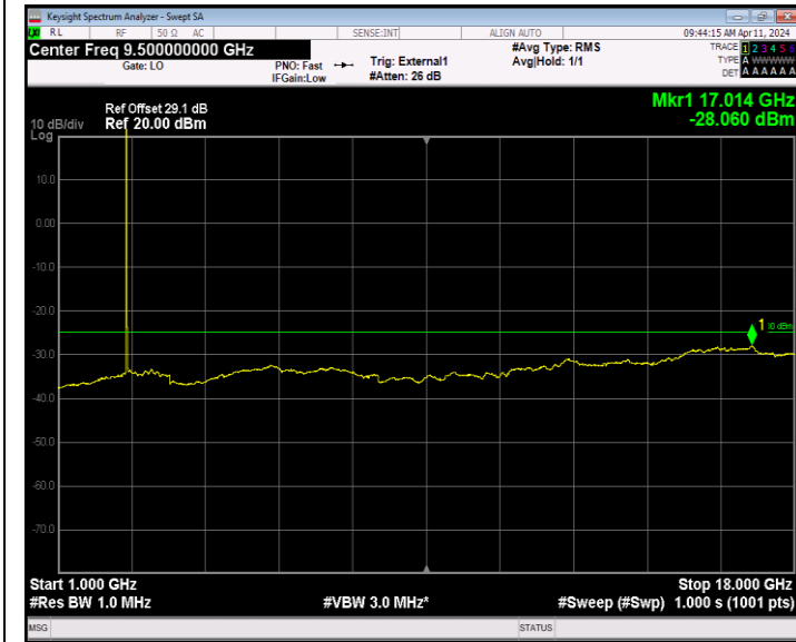
Band41_20MHz_16QAM_40620_1RB#0_1000~18000_1000~18000
