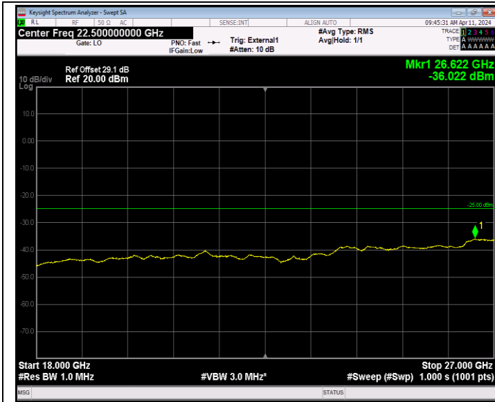
Band41_20MHz_64QAM_40620_1RB#0_18000~27000_18000~27000
