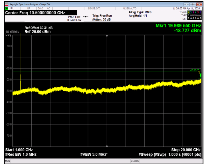
Band66_20MHz_64QAM_132572_1RB#0_1000~20000_1000~20000
