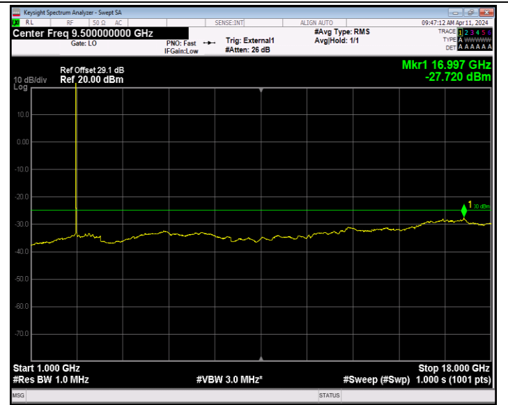
Band41_20MHz_16QAM_41490_1RB#0_1000~18000_1000~18000
