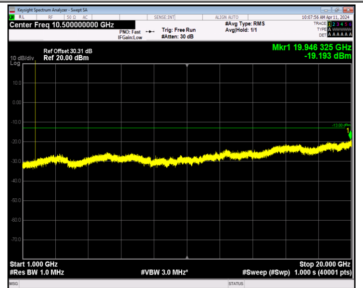
Band66_1.4MHz_64QAM_132322_1RB#0_1000~20000_1000~20000
