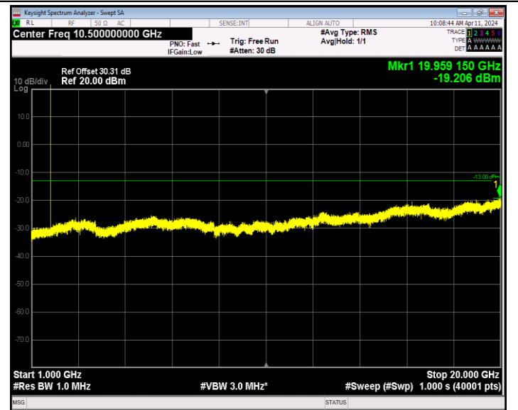
Band66_1.4MHz_16QAM_132665_1RB#0_1000~20000_1000~20000
