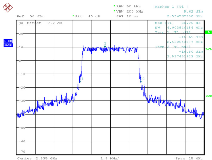
LTE band 7, 5MHz Bandwidth, 16QAM (-26dBc BW)
