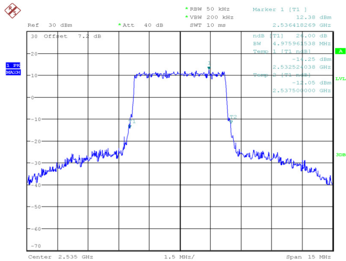
LTE band 7, 5MHz Bandwidth, QPSK (-26dBc BW)
