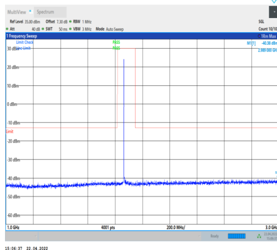
1-N25--15-40-M-1-DFT-PI2BPSK-Inner_1RB_Left-1 @1-1000-3000-Ant0--40.38--13-PASS
