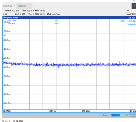
1-N25--15-40-M-1-DFT-PI2BPSK-Inner_1RB_Left-1 @1-30-1000-Ant0--49.92--23-PASS
