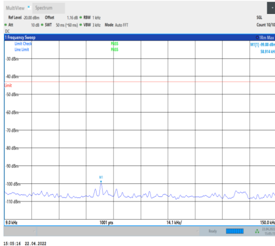
1-N25--15-40-L-1-DFT-PI2BPSK-Inner_1RB_Left-1 @1-0.009-0.15-Ant0--99.88--43-PASS
