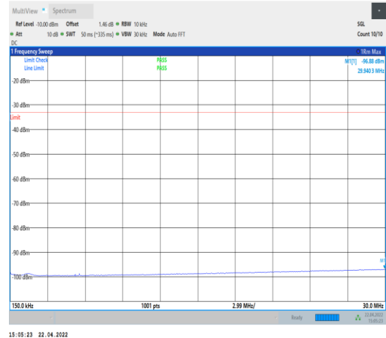
1-N25--15-40-L-1-DFT-PI2BPSK-Inner_1RB_Left-1@ 1-0.15-30-Ant0--96.88--33-PASS
