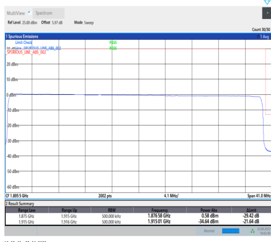
1-N25--15-40-H-6-CP-QPSK-Outer_Full-216@0-A nt0-seegraph-PASS-see graph
