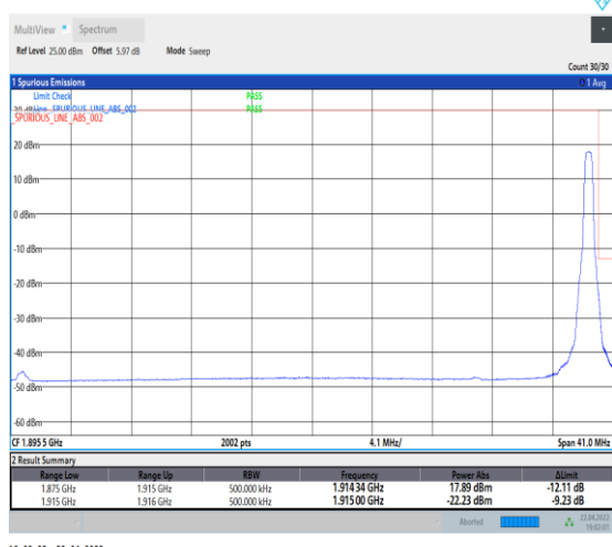
1-N25--15-40-H-5-CP-QPSK-Edge_1RB_Right-1@215 -Ant0-seegraph-PASS-see graph
