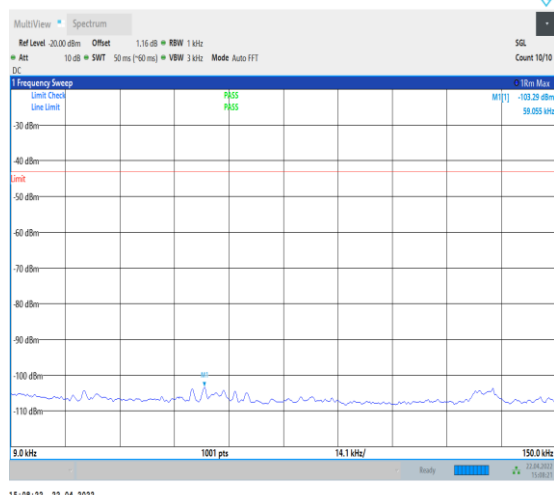
1-N25--15-40-H-1-DFT-PI2BPSK-Inner_1RB_Left-1 @1-0.009-0.15-Ant0--103.29--43-PASS
