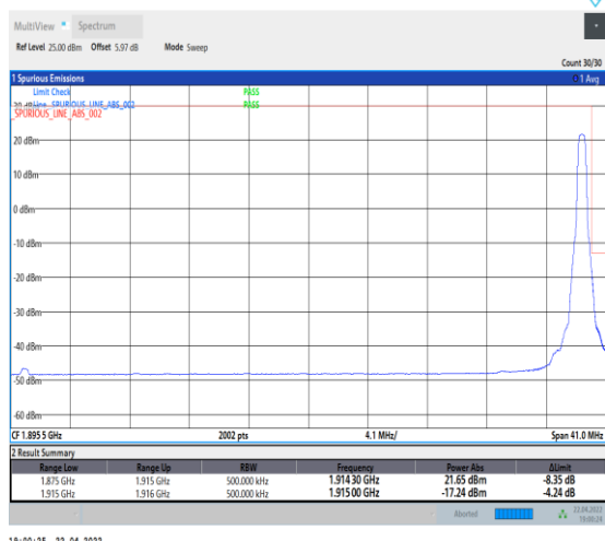
1-N25--15-40-H-2-DFT-PI2BPSK-Edge_1RB_Right-1 @215-Ant0-seegraph-PASS-see graph
