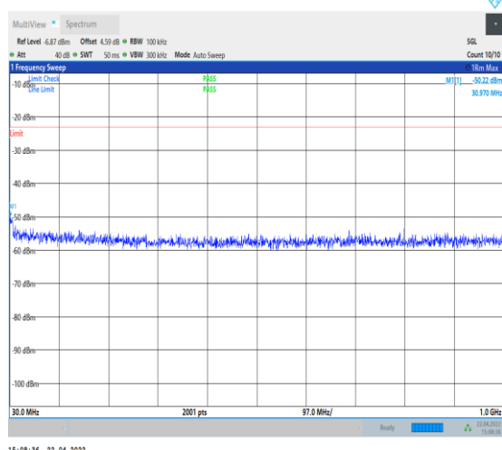
1-N25--15-40-H-1-DFT-PI2BPSK-Inner_1RB_Left-1 @1-30-1000-Ant0--50.22--23-PASS
