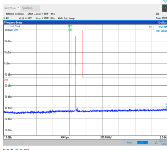
1-N25--15-40-H-1-DFT-PI2BPSK-Inner_1RB_Left-1 @1-1000-3000-Ant0--40.24--13-PASS
