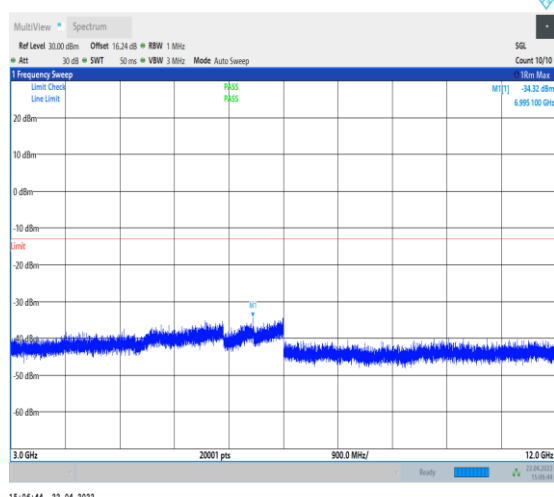
1-N25--15-40-M-1-DFT-PI2BPSK-Inner_1RB_Left-1 @1-3000-12000-Ant0--34.32--13-PASS
