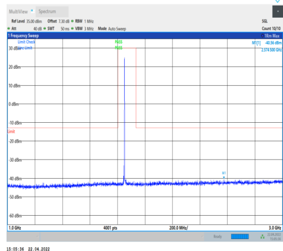
1-N25--15-40-L-1-DFT-PI2BPSK-Inner_1RB_Left-1@ 1-1000-3000-Ant0--40.56--13-PASS
