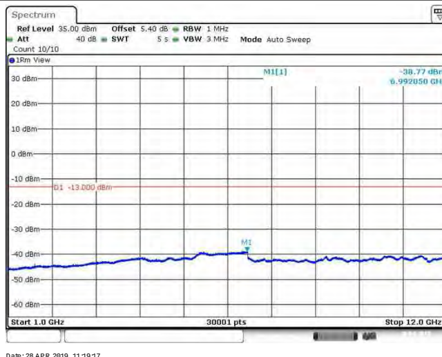
Band26_15MHz_16QAM_26915_1RB#0
