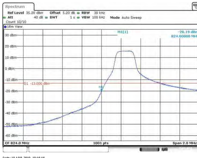
Band26_3MHz_64QAM_26805_15RB#0
