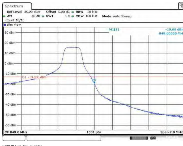
Band26_3MHz_64QAM_27025_15RB#0
