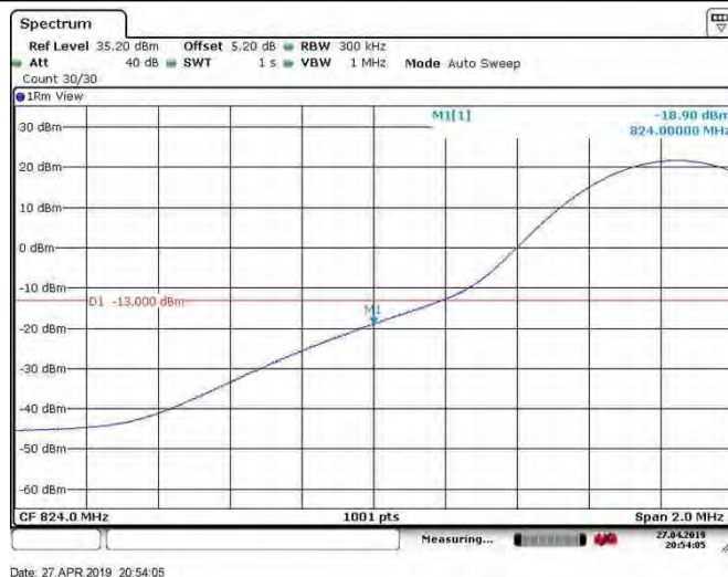
Band26_15MHz_64QAM_26865_75RB#0
