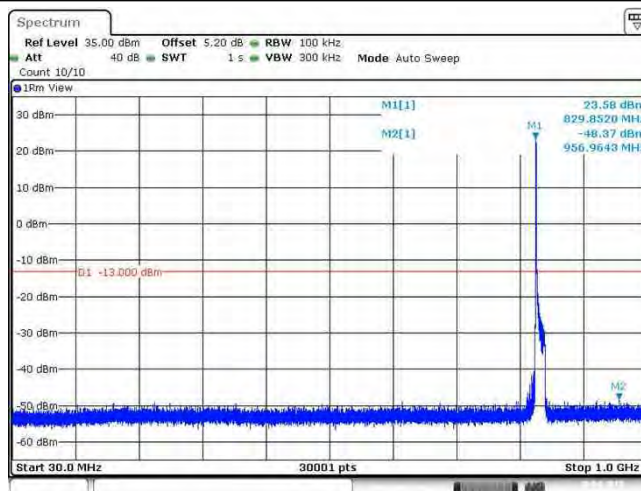
Band26_15MHz_QPSK_26915_1RB#0
