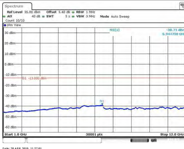
Band26_15MHz_64QAM_26865_1RB#0
