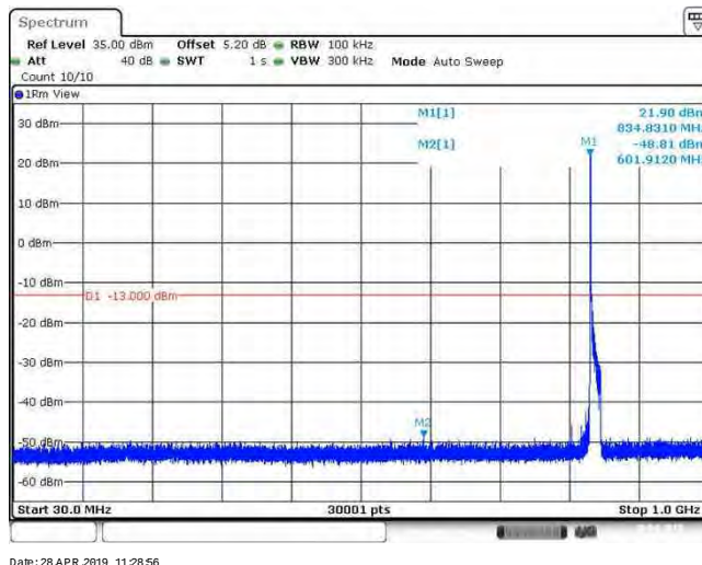
Band26_15MHz_64QAM_26965_1RB#0
