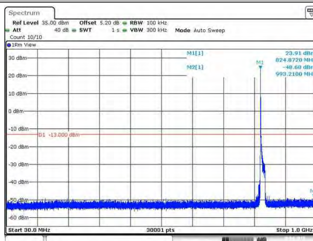
Band26_15MHz_QPSK_26865_1RB#0
