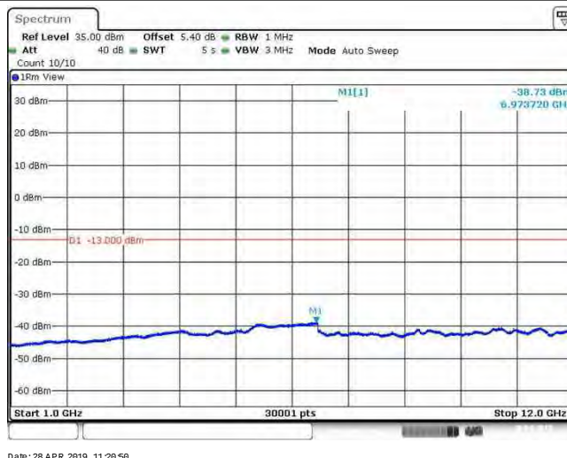
Band26_15MHz_64QAM_26915_1RB#0
