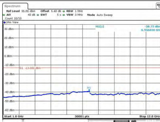
Band26_15MHz_QPSK_26865_1RB#0
