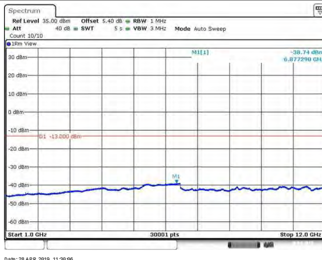
Band26_15MHz_16QAM_26865_1RB#0
