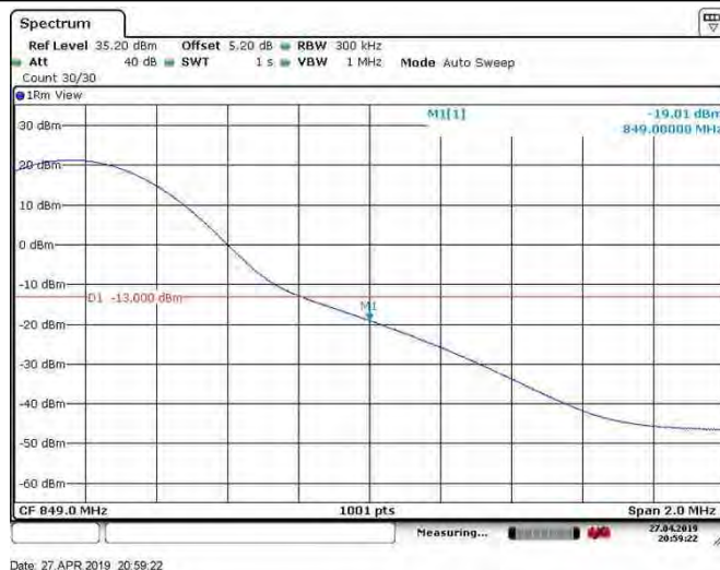
Band26_15MHz_64QAM_26965_75RB#0
