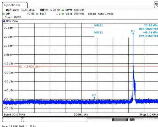
Band26_15MHz_QPSK_26965_1RB#0
