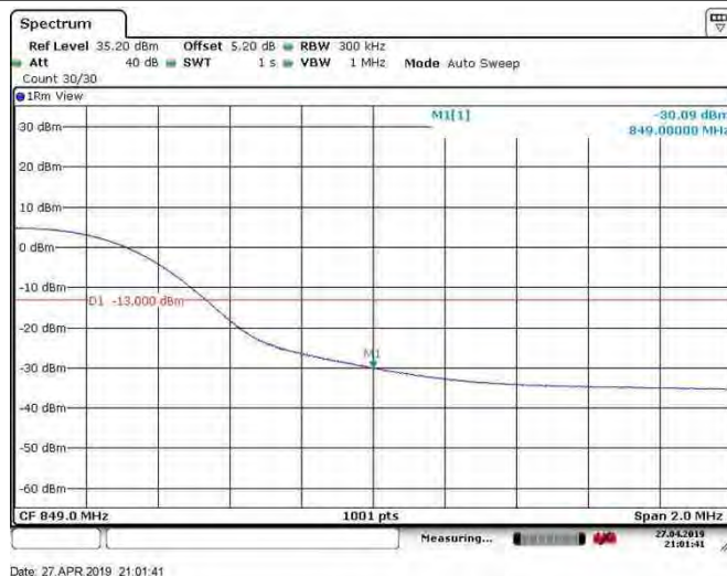
Band26_15MHz_64QAM_26865_1RB#0
