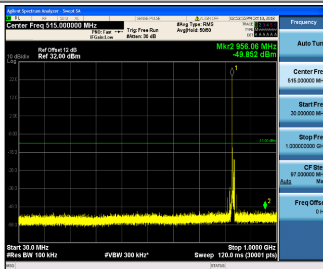
Band26_10MHz_16QAM_20525_1RB#0
