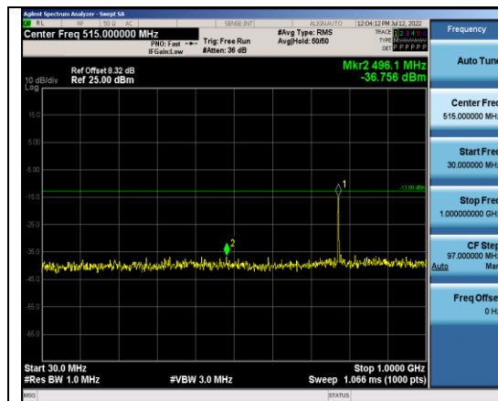
Band13-10MHz-QPSK-23230-1RB#0- Range1:30~1000MHz
