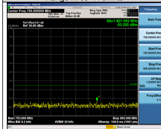
Band13-10MHz-16QAM-23230-1RB#0- Range5:793~805MHz
