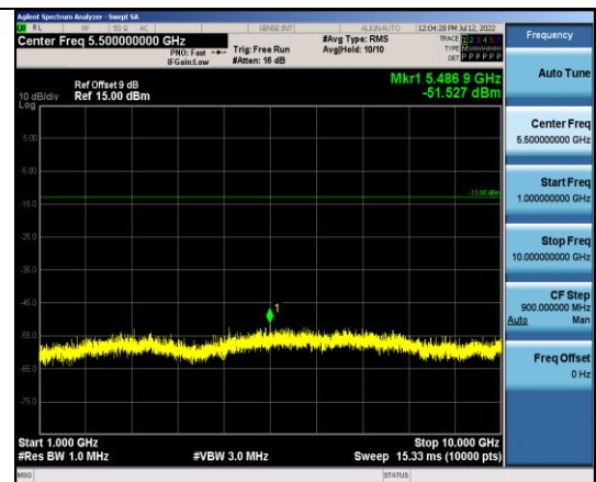
Band13-10MHz-QPSK-23230-1RB#0- Range2:1000~10000MHz
