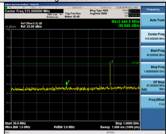
Band13-10MHz-16QAM-23230-1RB#0- Range1:30~1000MHz
