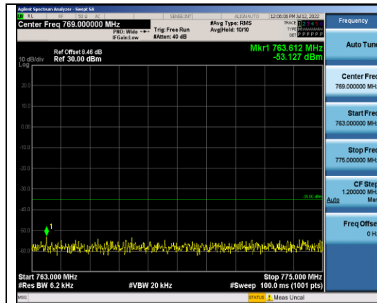
Band13-10MHz-16QAM-23230-1RB#0- Range4:763~775MHz
