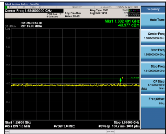
Band13-10MHz-16QAM-23230-1RB#0- Range3:1559~1610MHz
