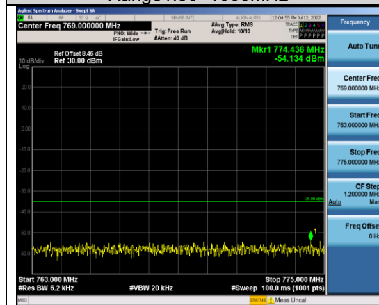
Band13-10MHz-QPSK-23230-1RB#0- Range4:763~775MHz
