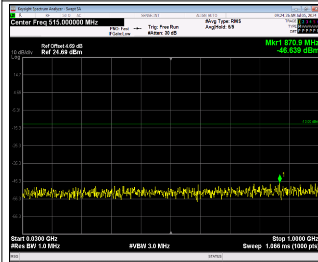
Band66-1.4MHz-16QAM-131979-1RB#0-Range1:3~0~1000MHz
