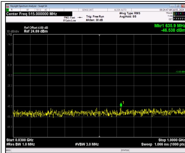
Band66-1.4MHz-QPSK-132665-1RB#0-Range1:30~1000MHz
