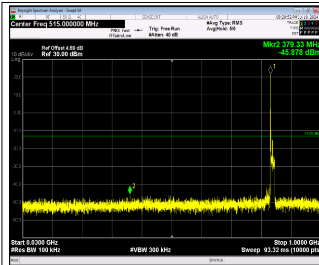
Band41-5MHz-QPSK-39675-1RB#0-Range1:30~1000MHz
