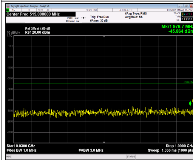
Band41-5MHz-QPSK-40620-1RB#0-Range1:30~1000MHz
