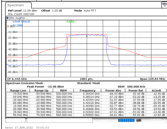
802.11ax (40MHz) / 6445MHz / Chain A / NSS-1
