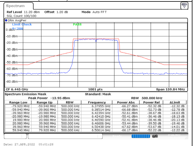
802.11ax (40MHz) / 6445MHz / Chain B / NSS-1
