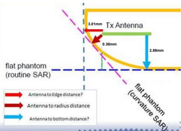
X=3.01mm, Y=2.88mm, Z=0.38mm Exterior Radius Dimension for WLAN
