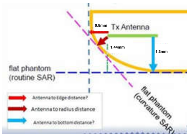
X=0.8mm, Y=1.3mm, Z=1.44mm Exterior Radius Dimension for WWAN
