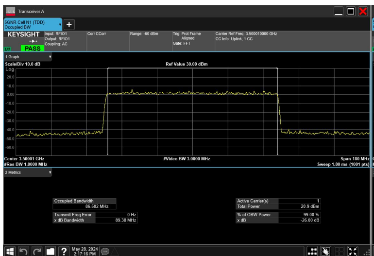
90MHz_30kHz_3500MHz_DFT-s-OFDM16QAM_RB243@0
