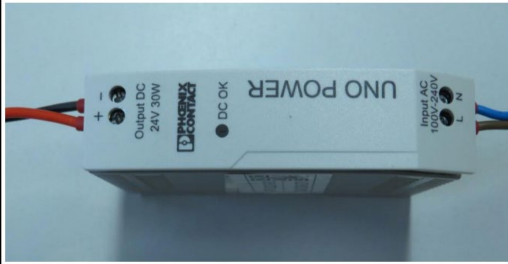
EUT power supply AC/DC-adapter
