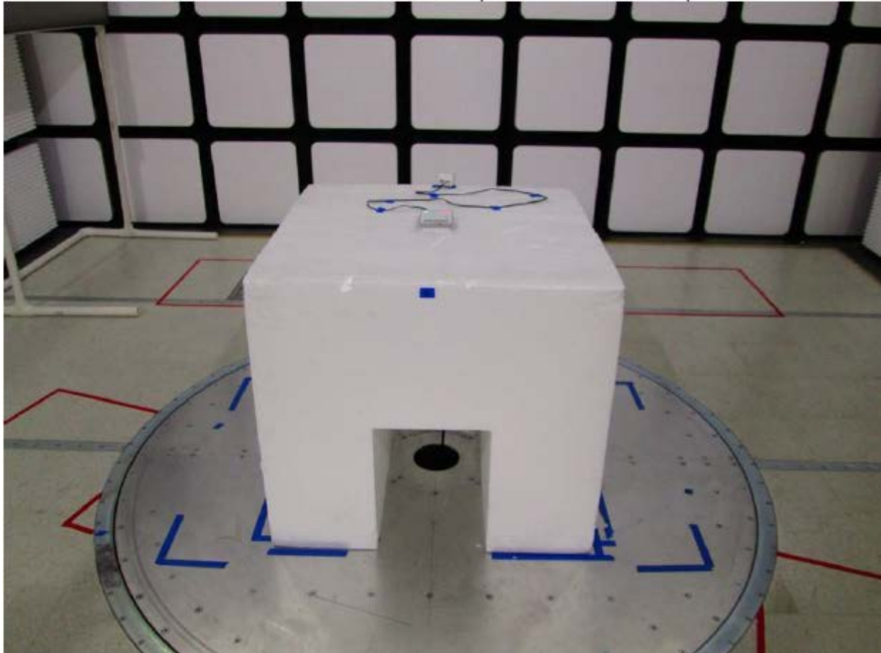
Radiated Testing Below 1GHz - Front View
