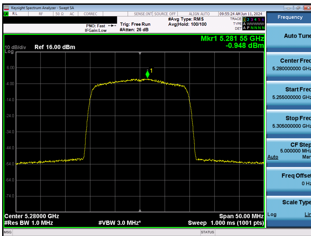
Plot 7-135. Power Spectral Density Plot MIMO ANT2 (20MHz BW 802.11ax (UNII Band 2A) – Ch. 56)
