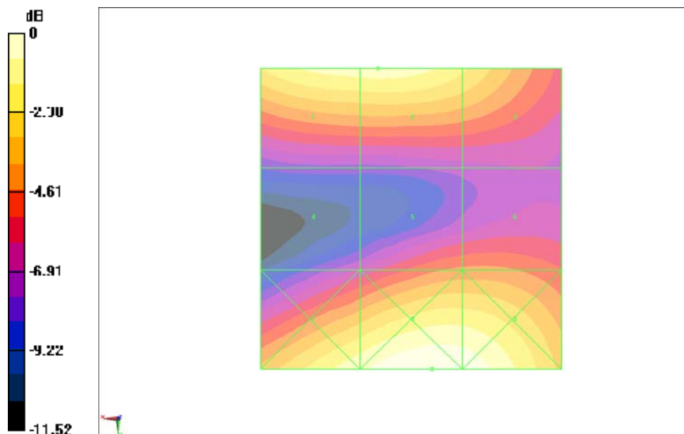
Fig B.9 HAC RF E-Field WCDMA 1900 Low
