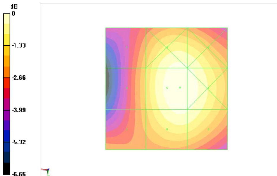
Fig B.17 HAC RF H-Field WCDMA 1900 Middle
