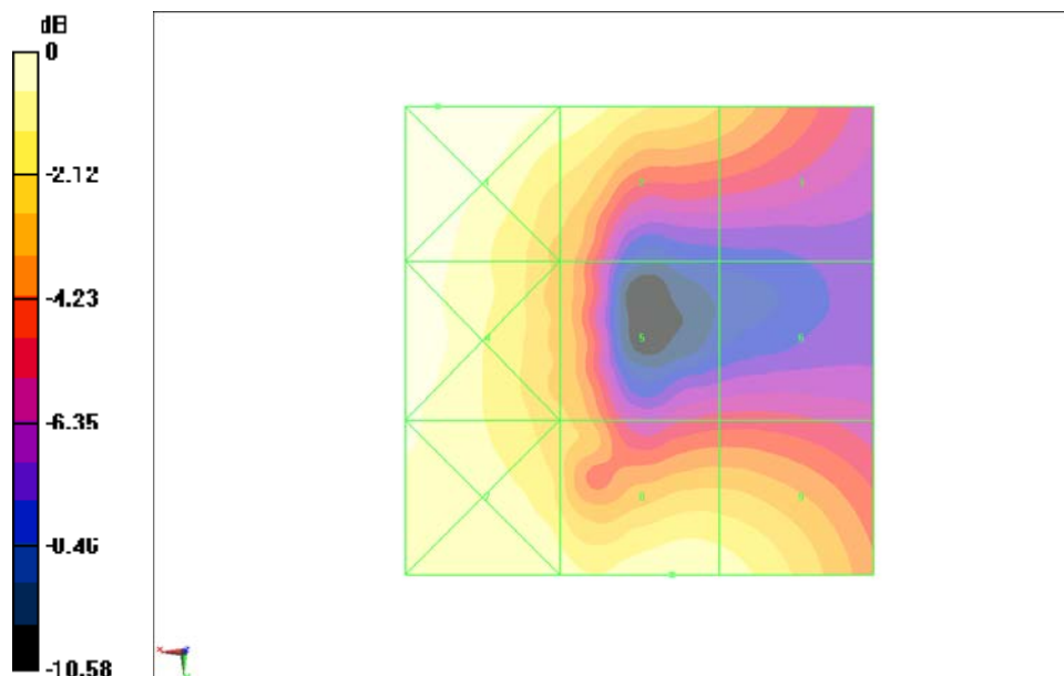
Fig B.7 HAC RF E-Field WCDMA 1900 High
