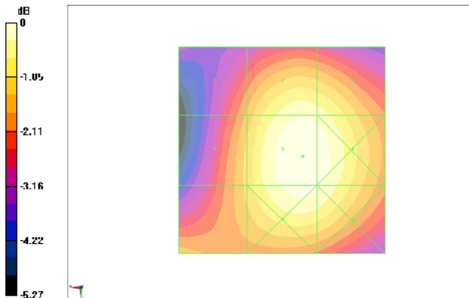
Fig B.18 HAC RF H-Field WCDMA 1900 Low
