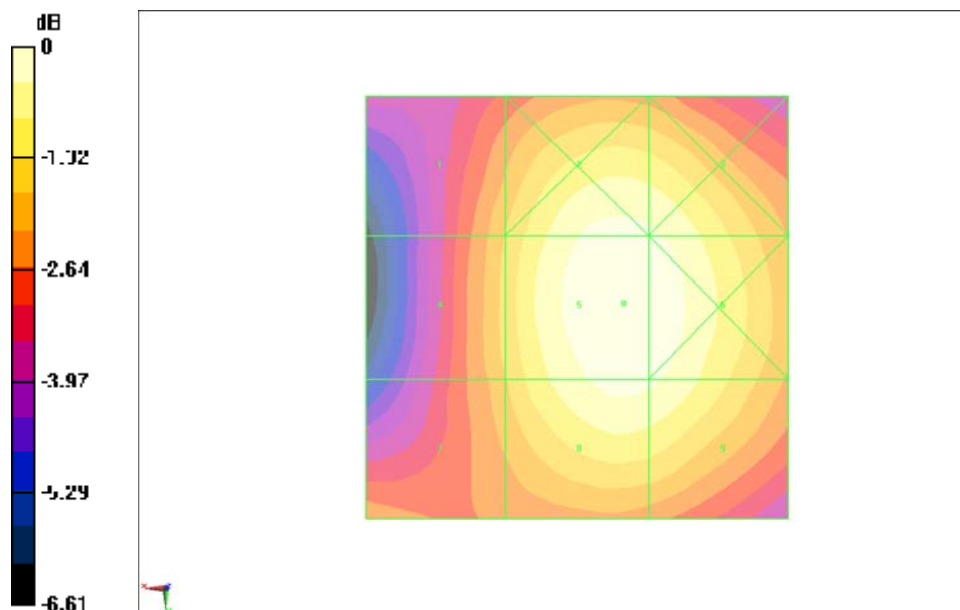
Fig B.14 HAC RF H-Field GSM 1900 Middle
