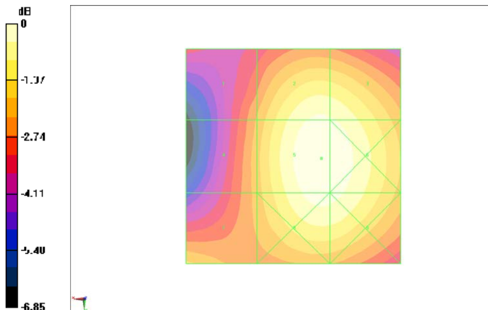
Fig B.16 HAC RF H-Field WCDMA 1900 High
