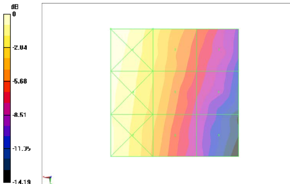
Fig B.10 HAC RF H-Field GSM 850 High
