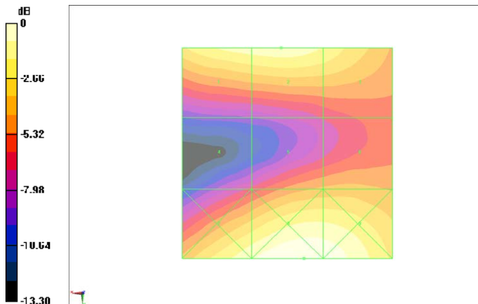
Fig B.8 HAC RF E-Field WCDMA 1900 Middle
