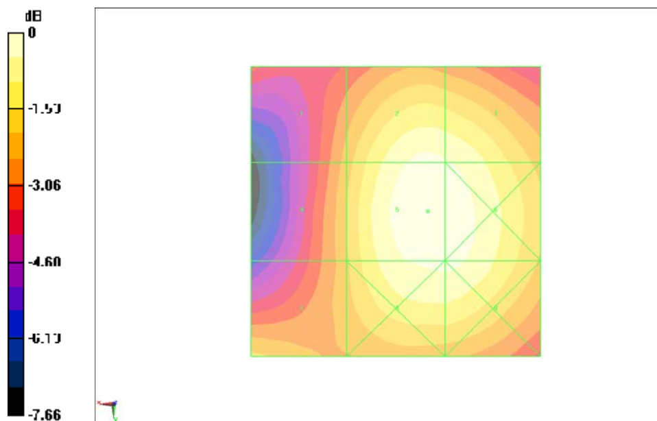
Fig B.13 HAC RF H-Field GSM 1900 High
