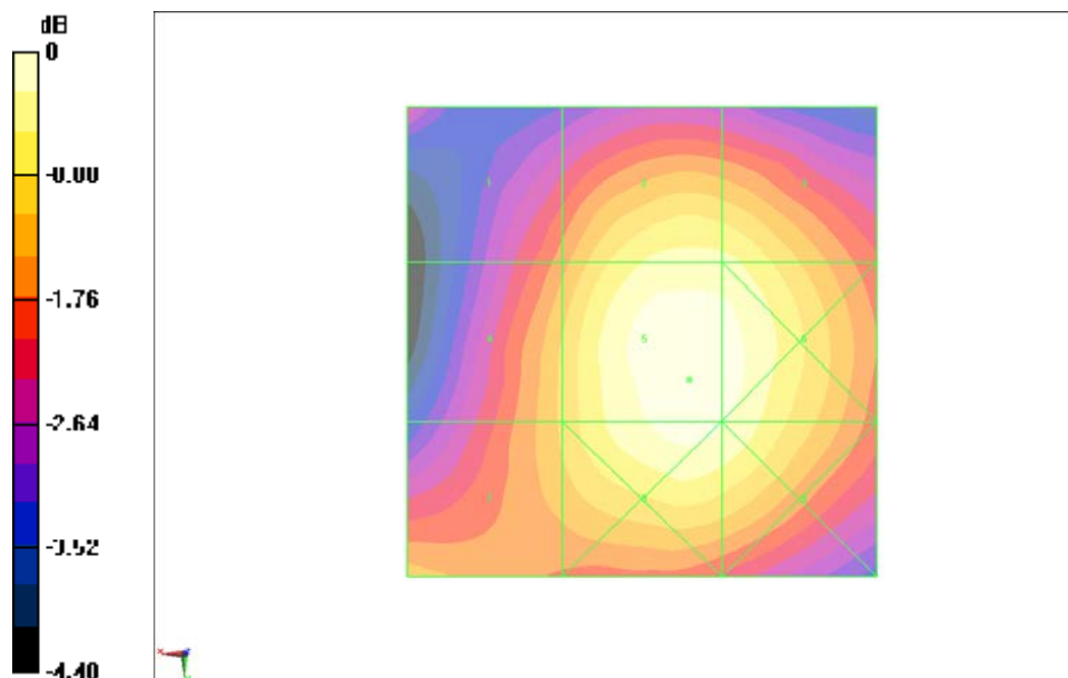
Fig B.15 HAC RF H-Field GSM 1900 Low
