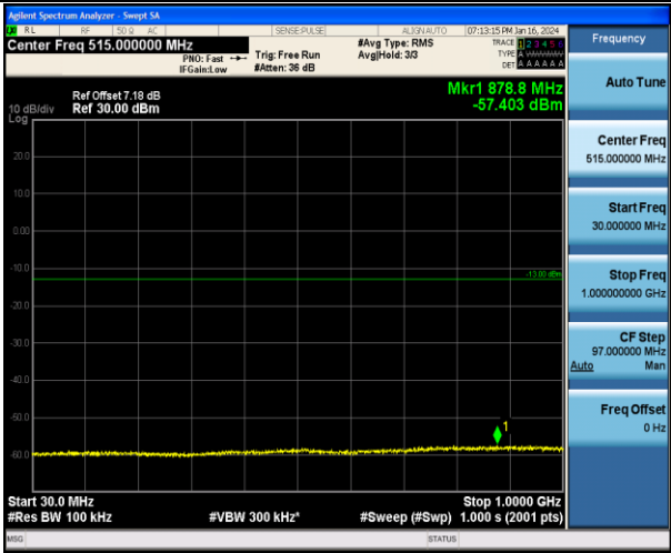
Band2_5MHz_QPSK_18900_1RB#0_30~1000_30~1000
