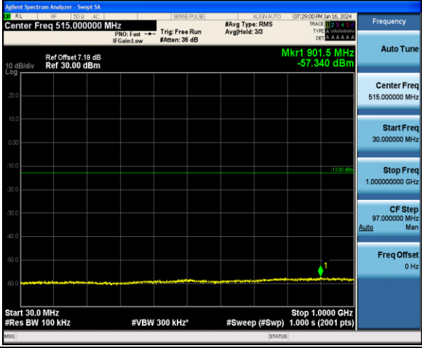
Band2_10MHz_16QAM_18650_1RB#0_30~1000_30~1000
