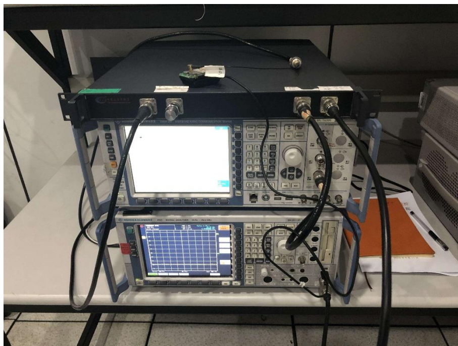
Test Setup Photo 2 for RF test
