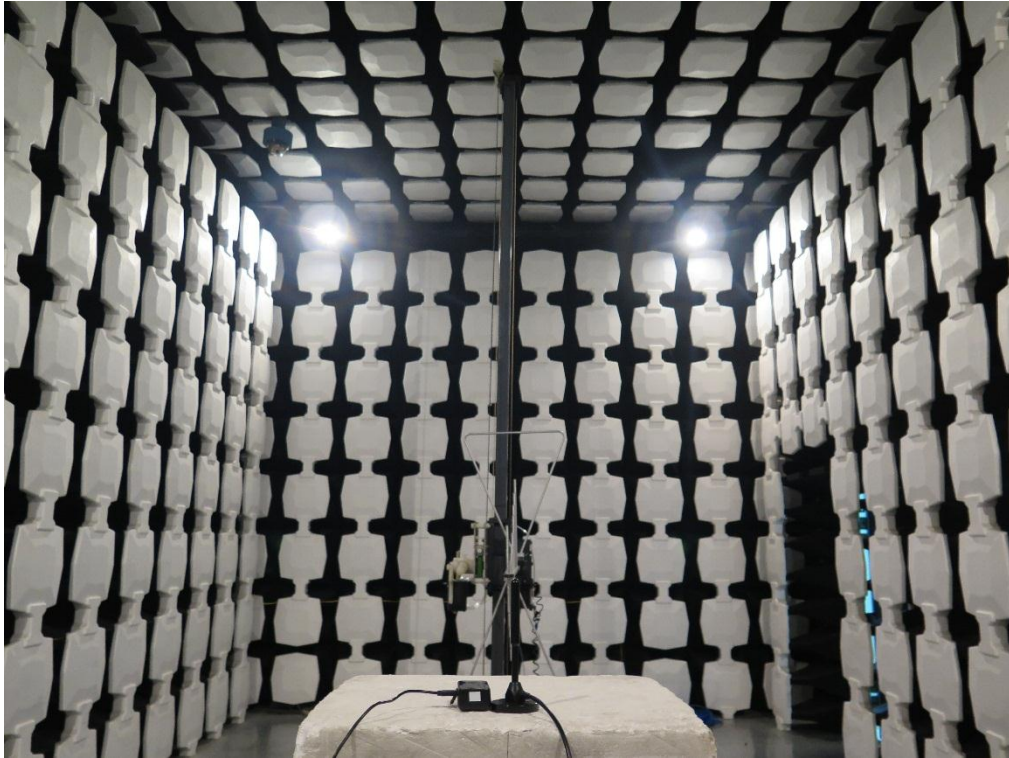
Test Setup Photo for RSE 30M-3G (The first measurement for ERP/EIRP)
