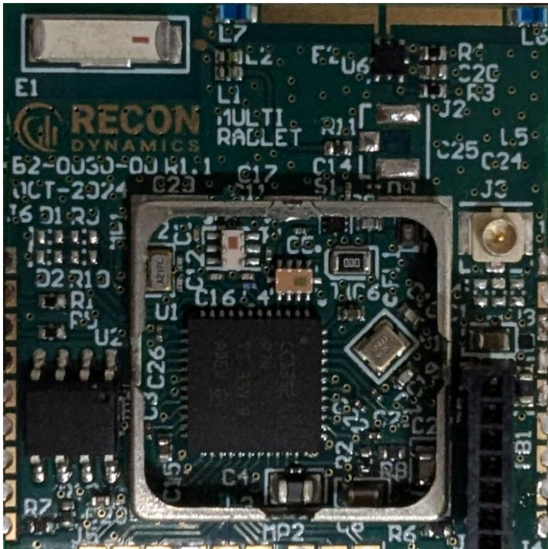
Photograph 2 – Front View of the Device with the Shield Removed
