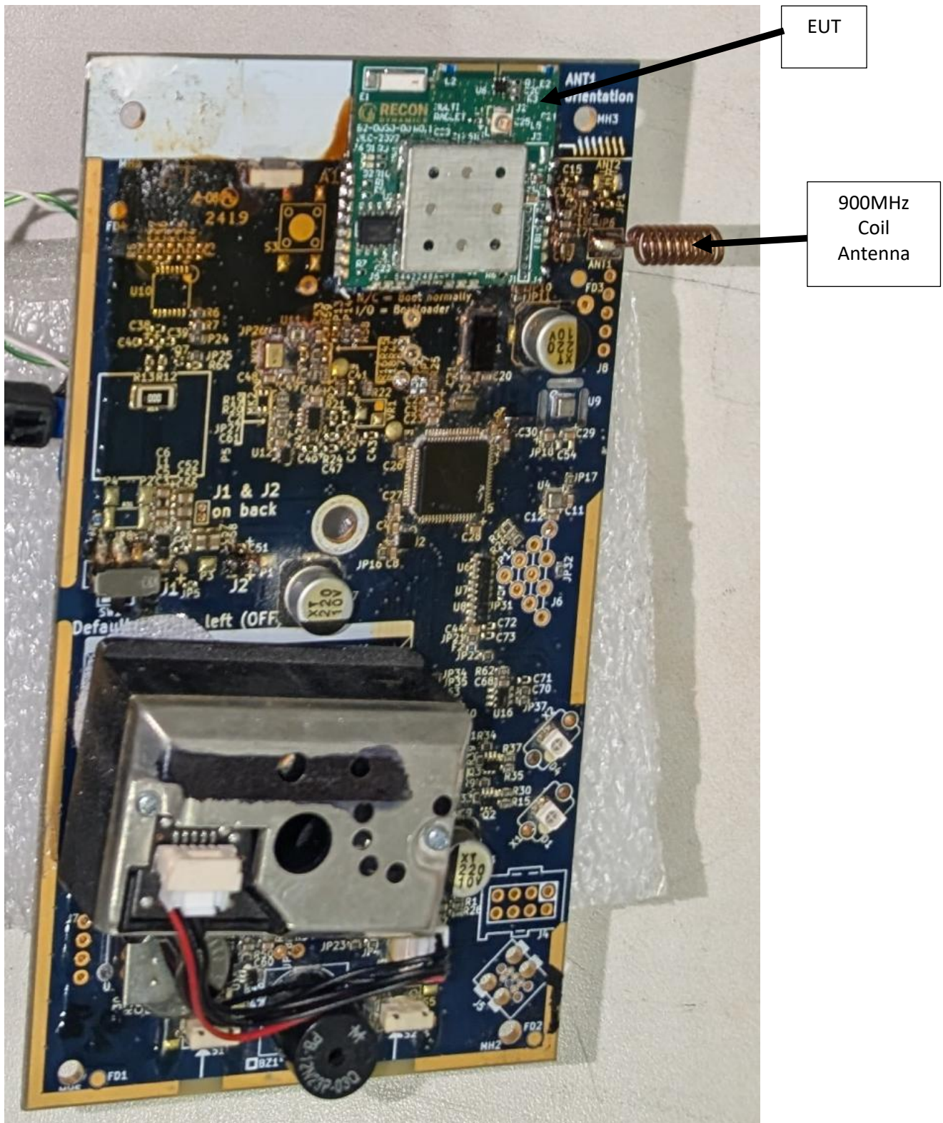
Photograph 5 – Device Attached to Host Device for Testing with 900 MHz Coil Antenna
