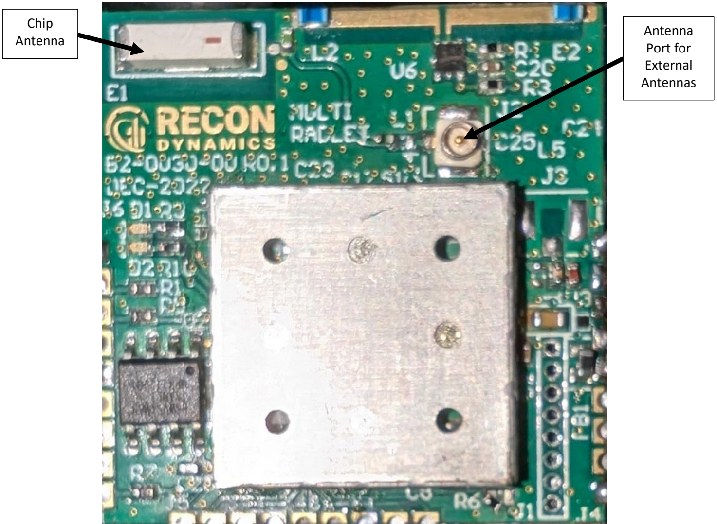
Photograph 1 – Front View of the Device
