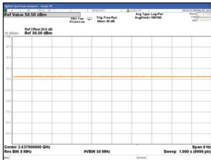
Chain1 : Ducty Cycle @ 802.11n(HT40) Mode
