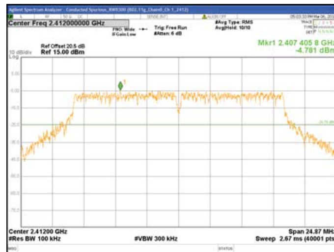
Chain0 : Conducted Spurious @ 802.11g Mode Ch 1
