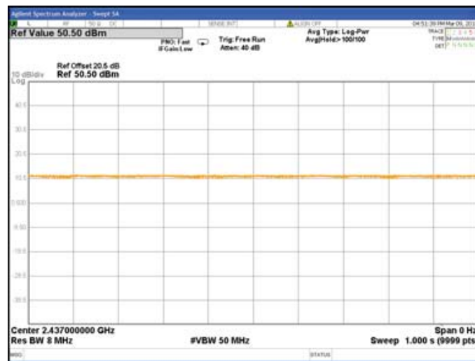
Chain0 : Ducty Cycle @ 802.11n(HT20) Mode
