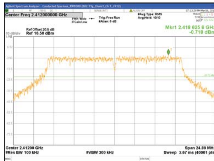
Chain1 : Conducted Spurious @ 802.11g Mode Ch 1
