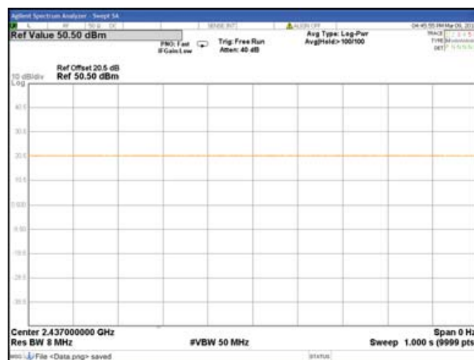
Chain0 : Ducty Cycle @ 802.11g Mode
