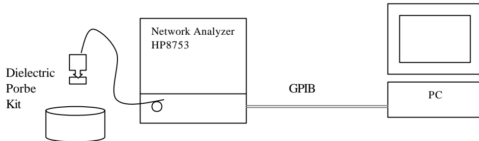
Figure 5: Test configuration
