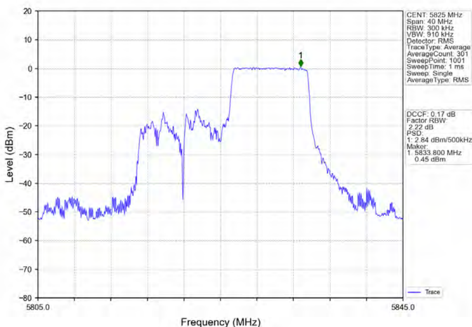
802.11ax(HE20)_HCH_5825MHz_RU106_Right_Ant2_NTNV
