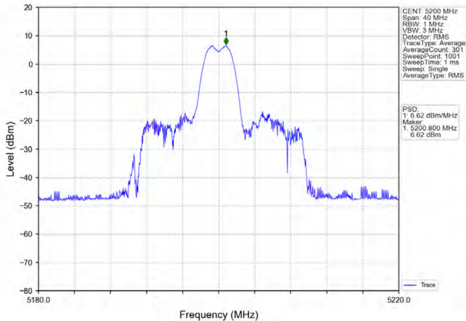
802.11ax(HE20)_MCH_5200MHz_RU26_Mid_Ant1_NTNV
