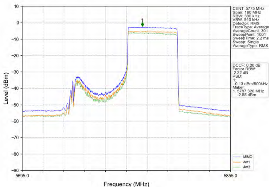
802.11ax(HE80)_MCH_5775MHz_RU484_Right_MIMO_NTNV
