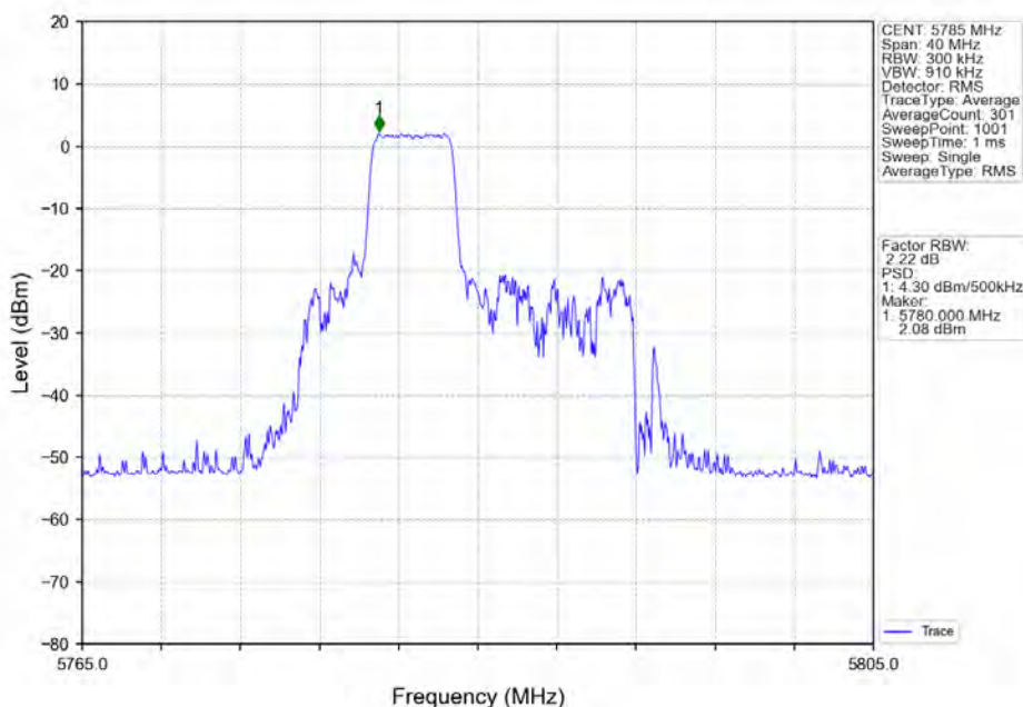
802.11ax(HE20)_MCH_5785MHz_RU52_Mid_Ant2_NTNV
