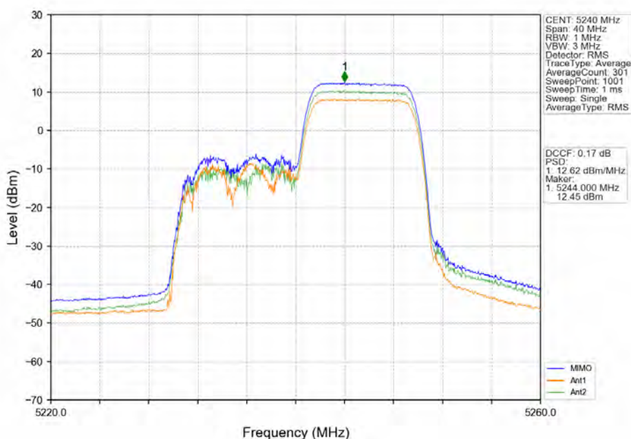
802.11ax(HE20)_HCH_5240MHz_RU106_Right_MIMO_NTNV
