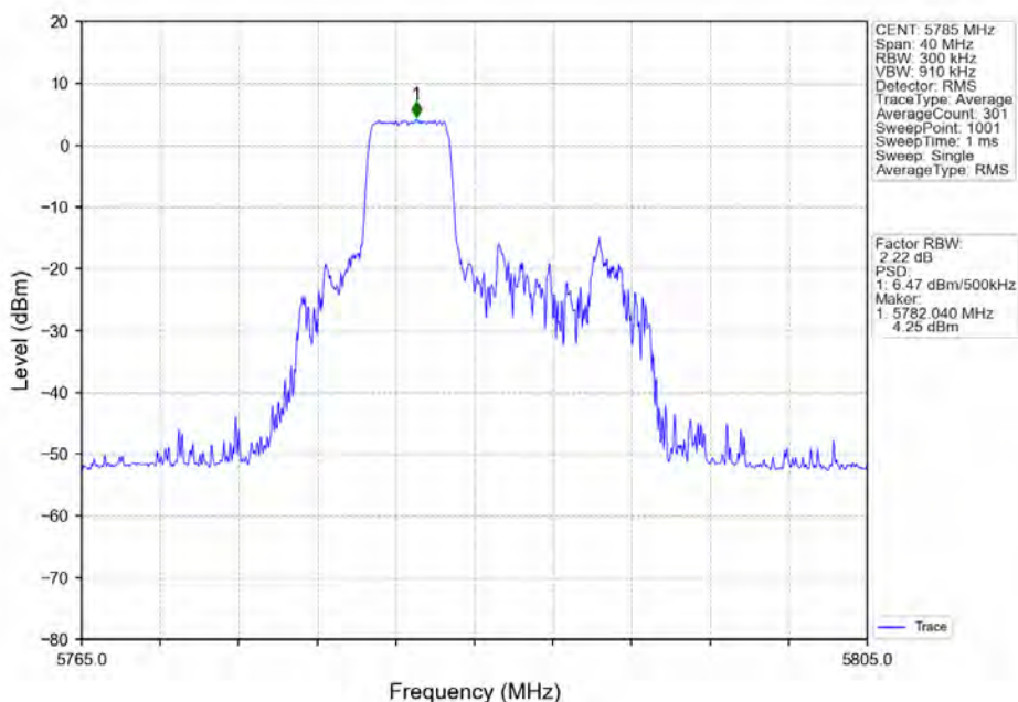
802.11ax(HE20)_MCH_5785MHz_RU52_Mid_Ant1_NTNV
