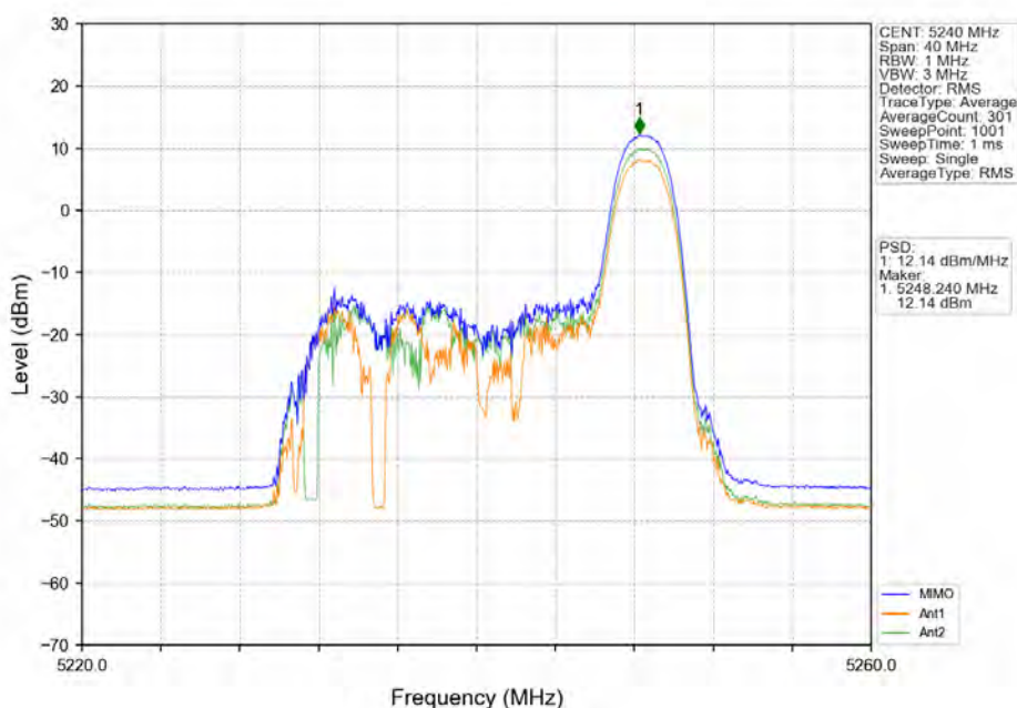
802.11ax(HE20) HCH_5240MHz_RU26_Right_MIMO_NTNV
