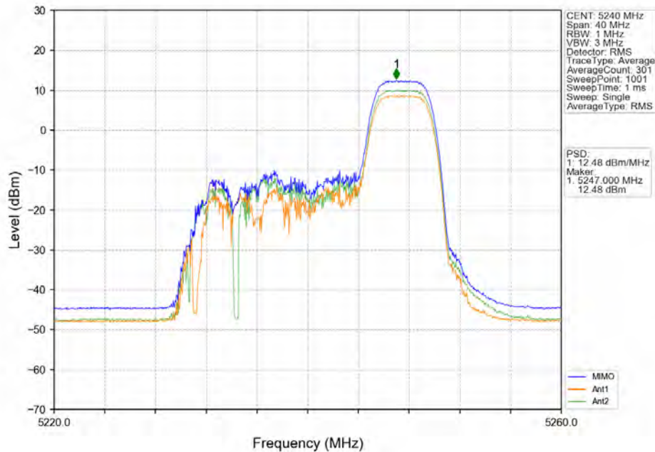
802.11ax(HE20) HCH_5240MHz_RU52_Right_MIMO_NTNV
