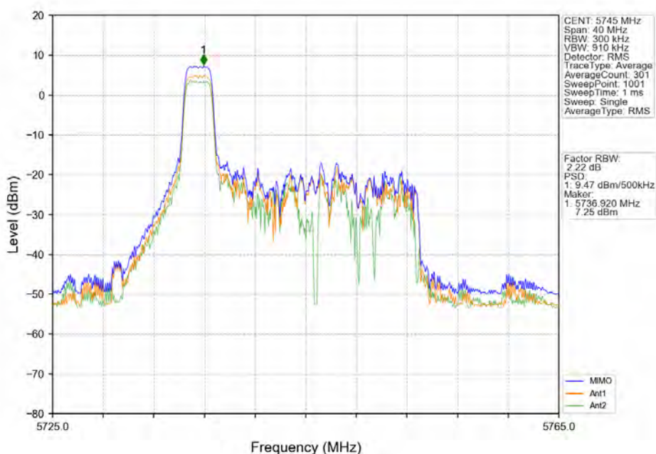
802.11ax(HE20)_LCH_5745MHz_RU26_Left MIMO_NTNV
