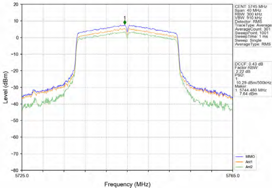
802.11ax(HE20)_LCH_5745MHz_RU242_Left_MIMO_NTNV
