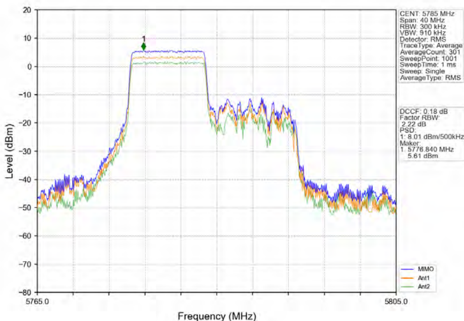
802.11ax(HE20)_MCH_5785MHz_RU106_Left_MIMO_NTNV
