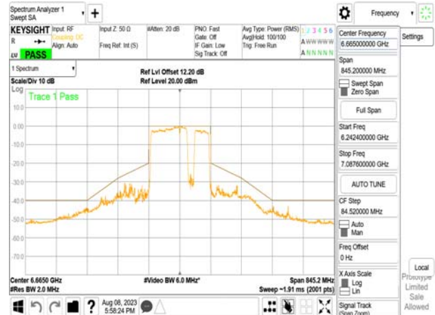
802.11be_160MHz_Chain1_6665MHz_SU_Punct40_High
