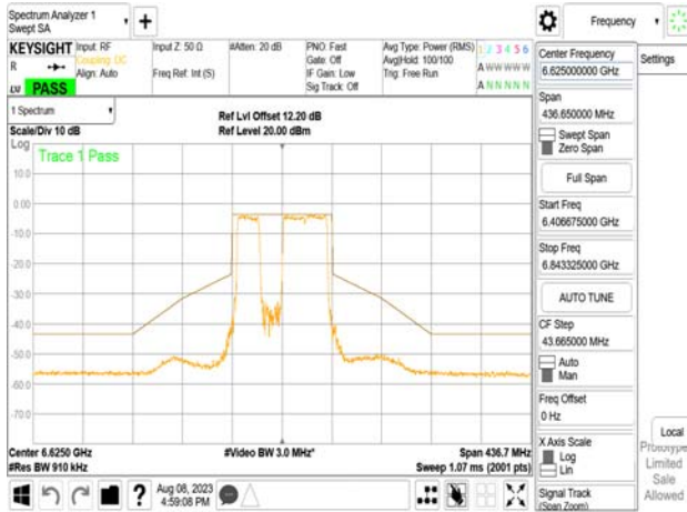
802.11be_80MHz_Chain1_6625MHz_SU_Punc20_Mid2
