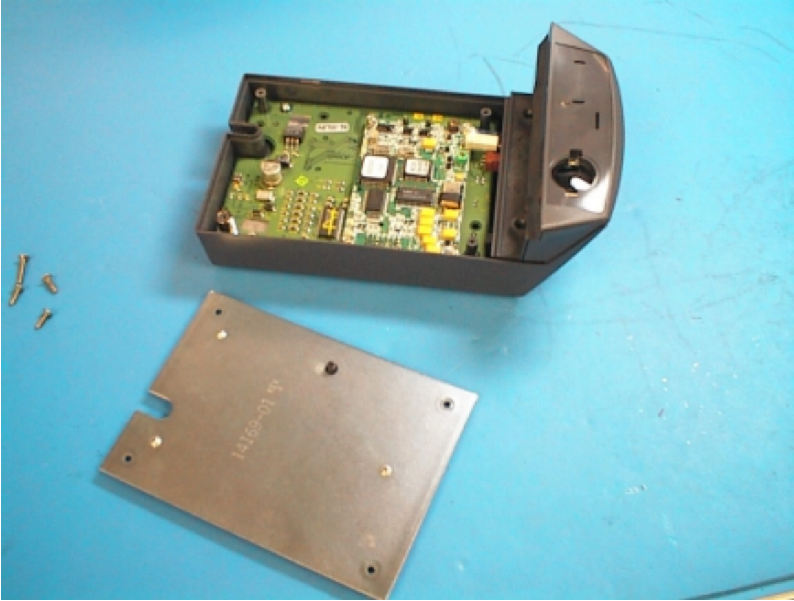
Photo 1 – Cover removed
