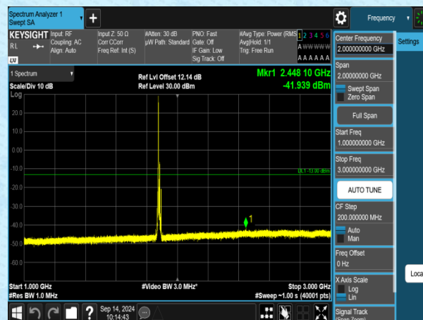
Band2-10MHz-QPSK-18900-1RB#0-1000~3000-PASS
