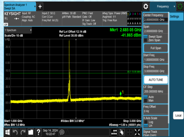
Band2-15MHz-QPSK-19125-1RB#0-1000~3000-PASS
