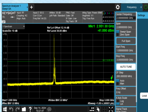
Band2-15MHz-QPSK-18900-1RB#0-1000~3000-PASS
