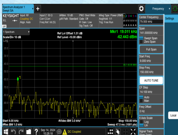
Band2-20MHz-QPSK-18900-1RB#0-0.009~0.15-PASS
