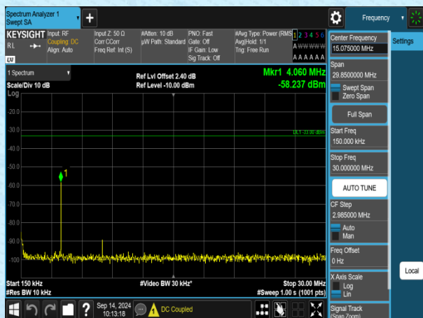
Band2-10MHz-QPSK-18650-1RB#0-0.15~30-PASS
