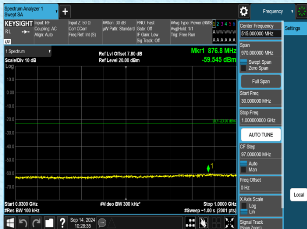
Band2-20MHz-QPSK-18900-1RB#0-30~1000-PASS
