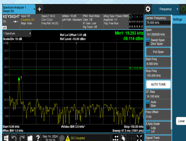
Band2-10MHz-QPSK-18900-1RB#0-0.009~0.15-PASS
