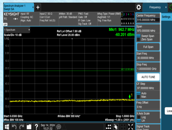
Band2-15MHz-QPSK-18900-1RB#0-30~1000-PASS
