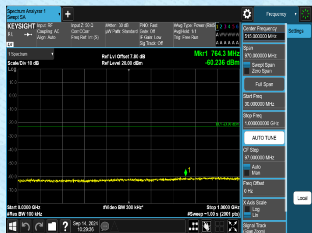
Band2-20MHz-QPSK-19100-1RB#0-30~1000-PASS
