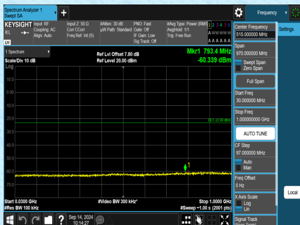
Band2-10MHz-QPSK-18900-1RB#0-30~1000-PASS
