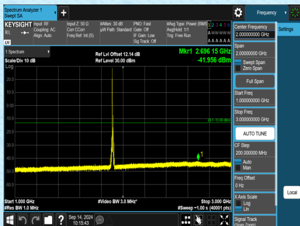
Band2-10MHz-QPSK-19150-1RB#0-1000~3000-PASS
