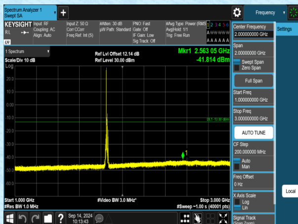
Band2-10MHz-QPSK-18650-1RB#0-1000~3000-PASS
