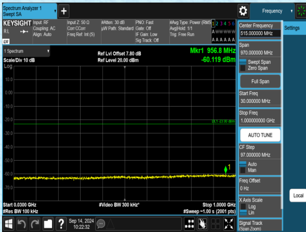
Band2-15MHz-QPSK-19125-1RB#0-30~1000-PASS
