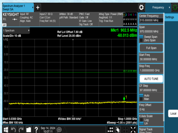
Band2-5MHz-QPSK-19175-1RB#0-30~1000-PASS
