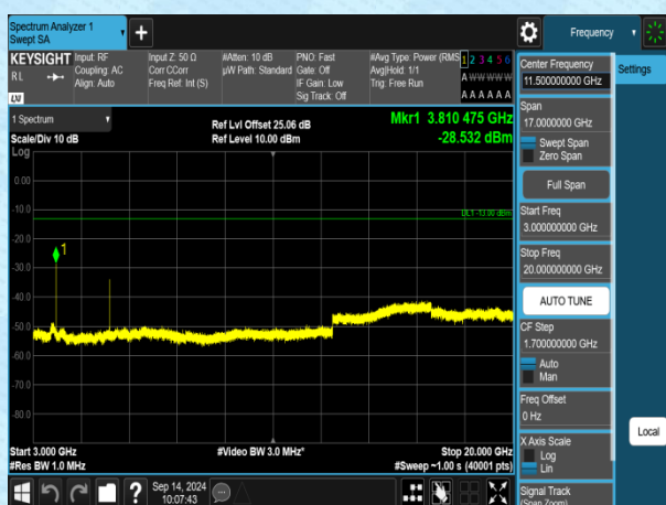
Band2-5MHz-QPSK-19175-1RB#0-3000~20000-PASS
