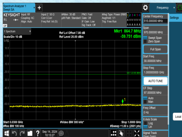
Band2-10MHz-QPSK-18650-1RB#0-30~1000-PASS
