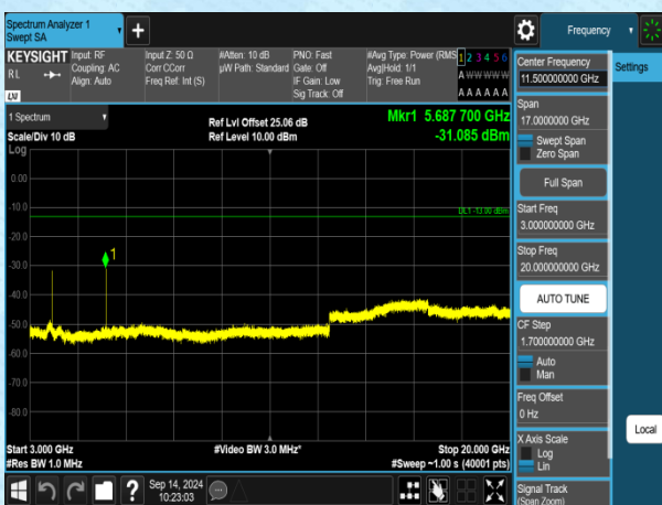
Band2-15MHz-QPSK-19125-1RB#0-3000~20000-PASS
