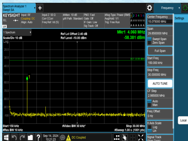
Band2-15MHz-QPSK-18900-1RB#0-0.15~30-PASS
