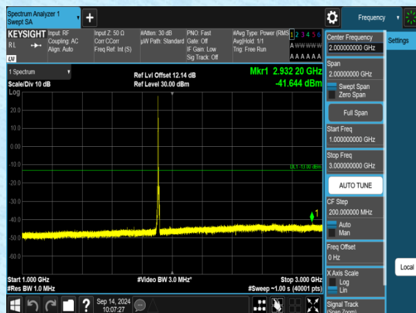
Band2-5MHz-QPSK-19175-1RB#0-1000~3000-PASS
