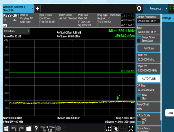
Band2-10MHz-QPSK-19150-1RB#0-30~1000-PASS
