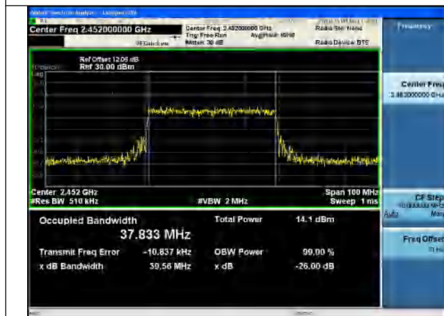
Test Mode:802.11be 2452MHz Chain0
