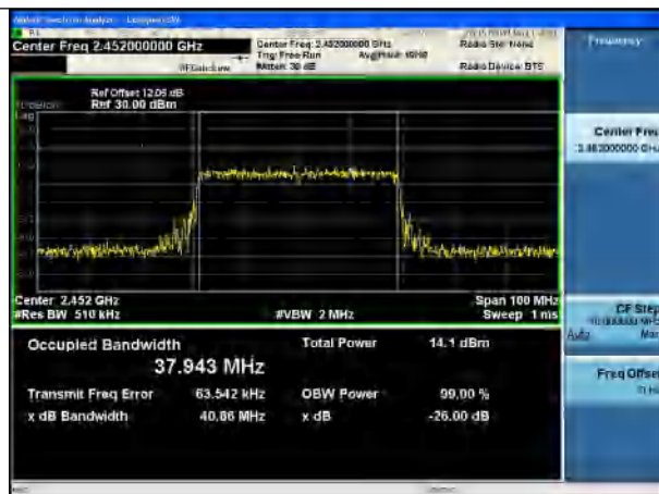
Test Mode:802.11be 2452MHz Chain1
