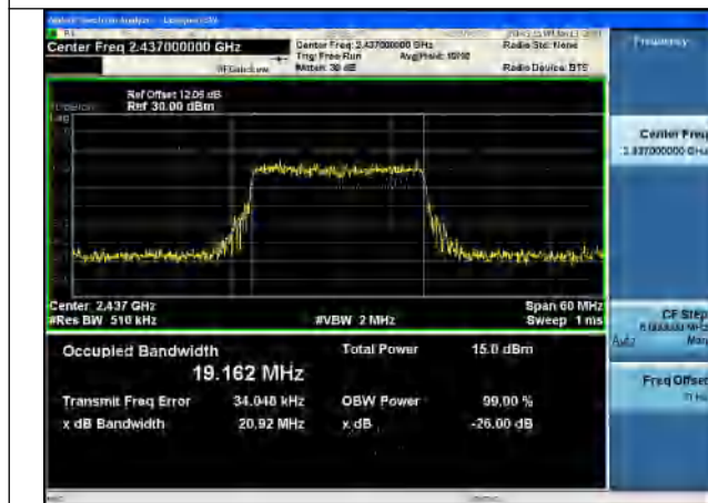
Test Mode:802.11be 2437MHz Chain1
