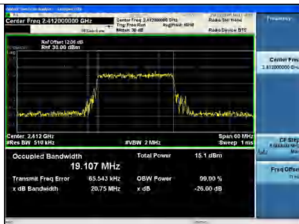
Test Mode:802.11be 2412MHz Chain1
