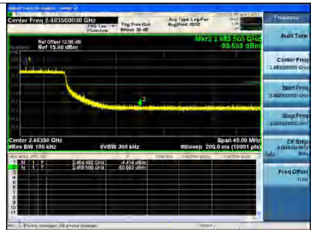
Test Mode:802.11be 2462MHz Chain1
