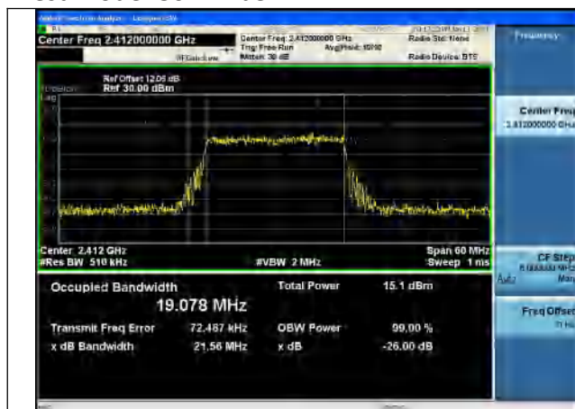
Test Mode:802.11be 2412MHz Chain0
