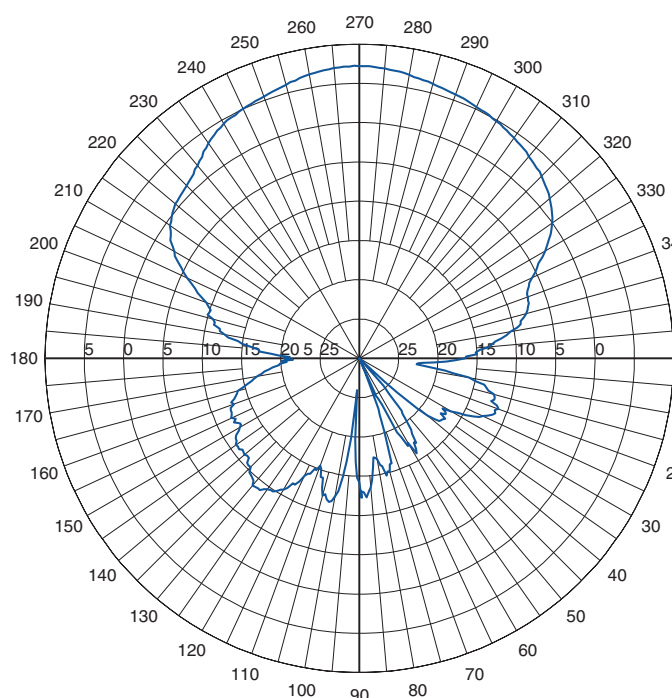
MP19008XFPT Elevation Cut
