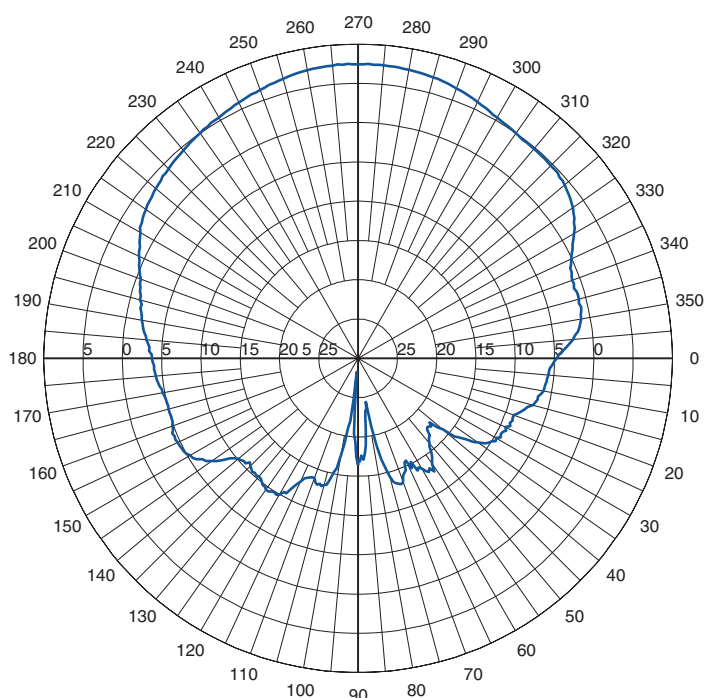
MP19008XFPT Azimuth Cut
