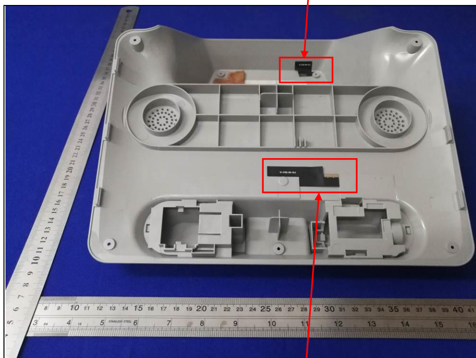
Diversity Antenna
