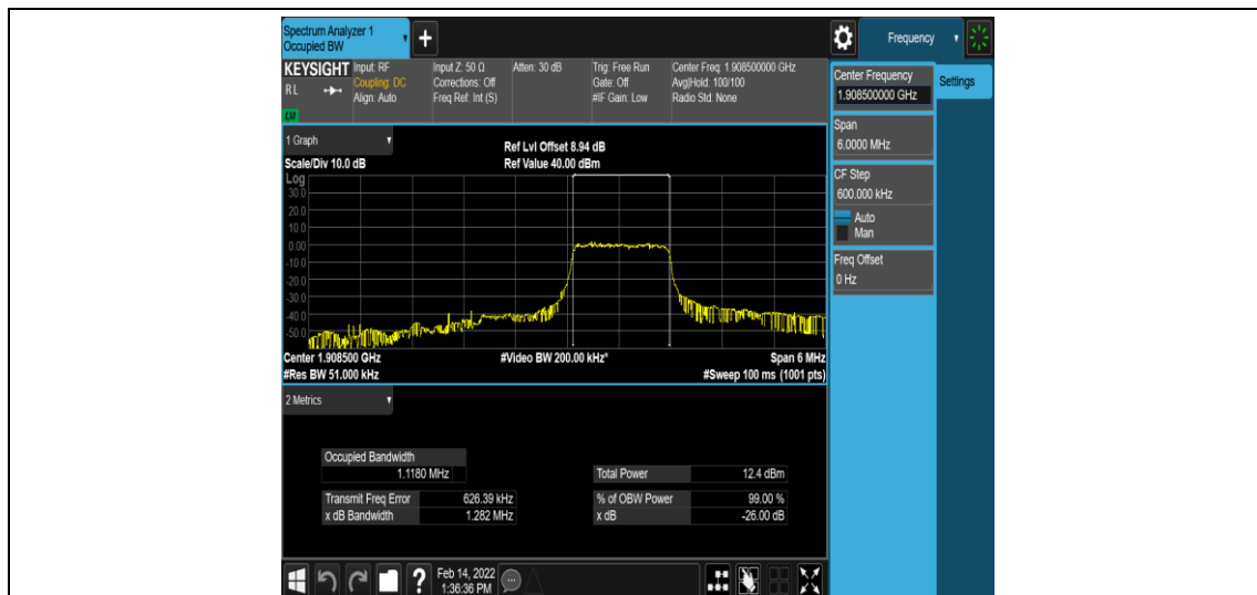
Band2-3MHz-QPSK-19185-6-0-High-1.1180-1.282-PASS
