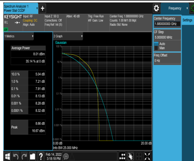
Band2-15MHz-QPSK-18900-6-0-Low-7.91-<=13-PASS
