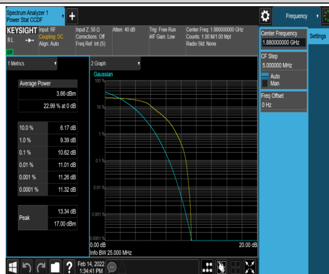
Band2-3MHz-16QAM-18900-6-0-Low-10.62-&lt;=13-PASS
