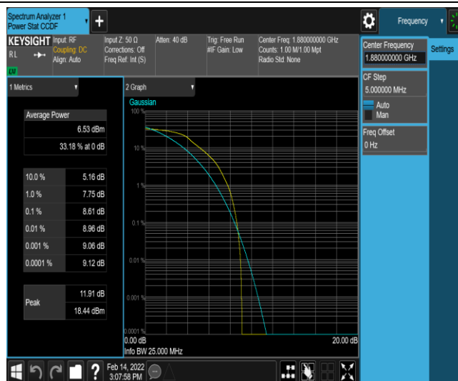
Band2-10MHz-16QAM-18900-6-0-Low-8.61-<=13-PASS
