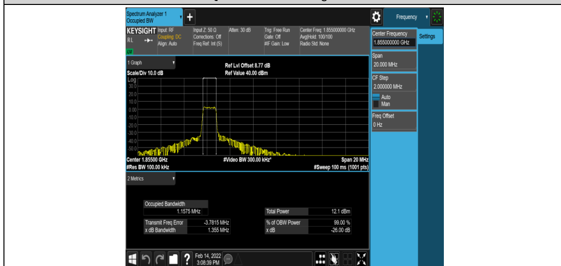
Band2-10MHz-QPSK-18650-6-0-Low-1.1575-1.355-PASS
