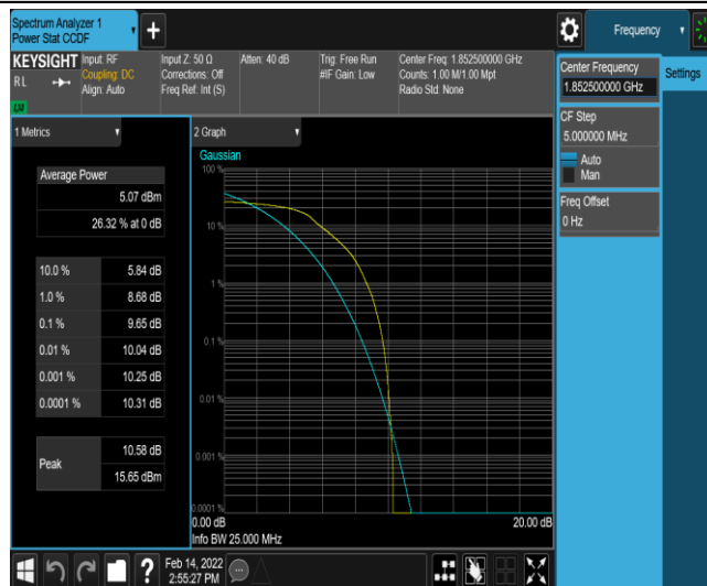
Band2-5MHz-16QAM-18625-6-0-Low-9.65-&lt;=13-PASS
