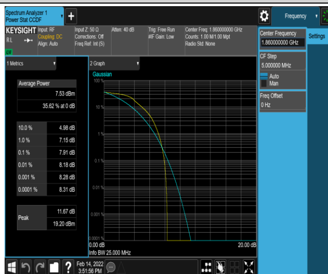
Band2-20MHz-16QAM-18700-6-0-Low-7.91-&lt;=13-PASS
