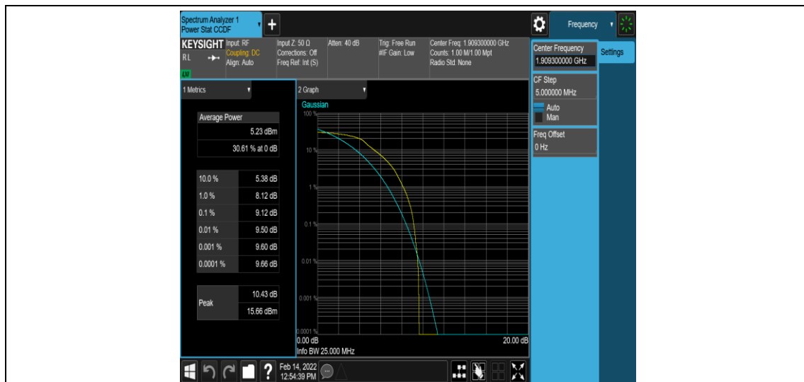
Band2-1.4MHz-16QAM-19193-6-0-Low-9.12-<=13-PASS
