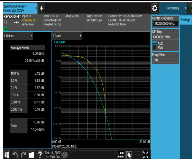
Band2-15MHz-16QAM-19125-6-0-Low-9.67-&lt;=13-PASS
