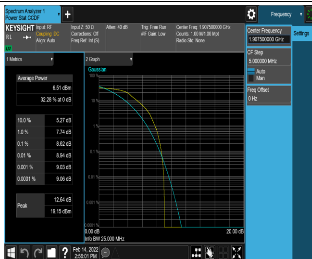
Band2-5MHz-QPSK-19175-6-0-Low-8.62-&lt;=13-PASS
