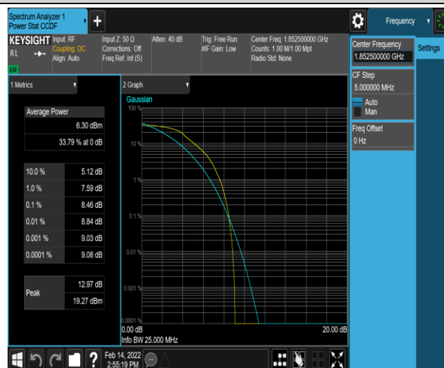
Band2-5MHz-OPSK-18625-6-0-Low-8.46-<=13-PASS
