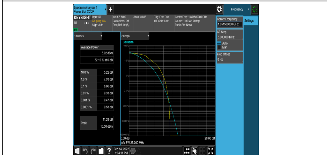
Band2-3MHz-QPSK-18615-6-0-Low-8.86-<=13-PASS
