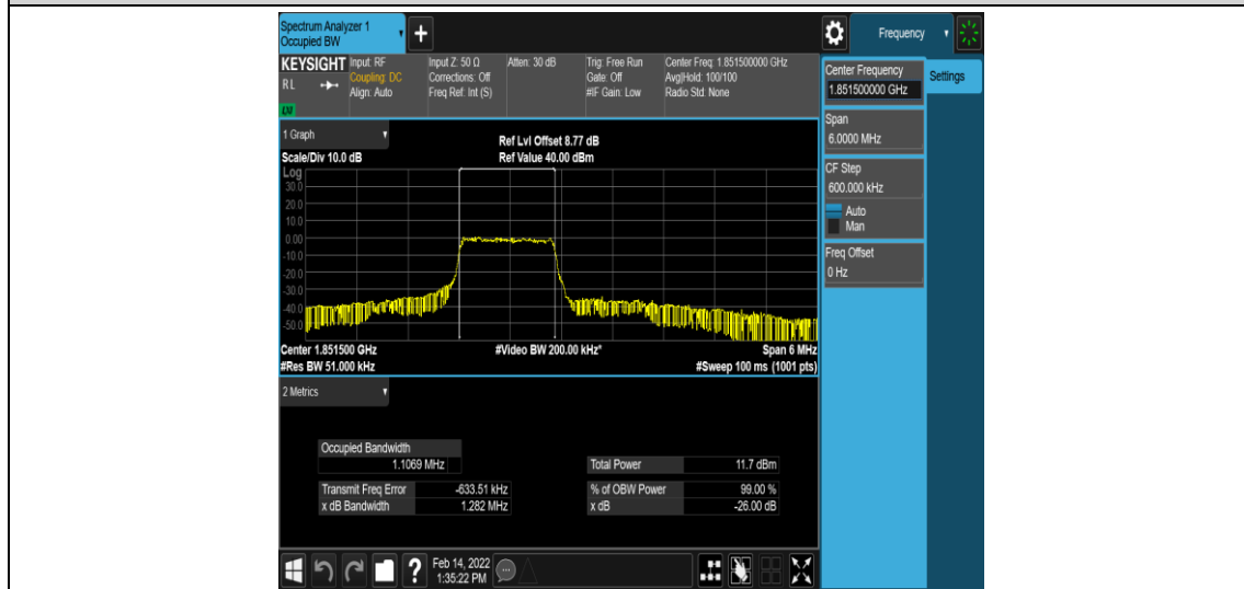
Band2-3MHz-QPSK-18615-6-0-Low-1.1069-1.282-PASS
