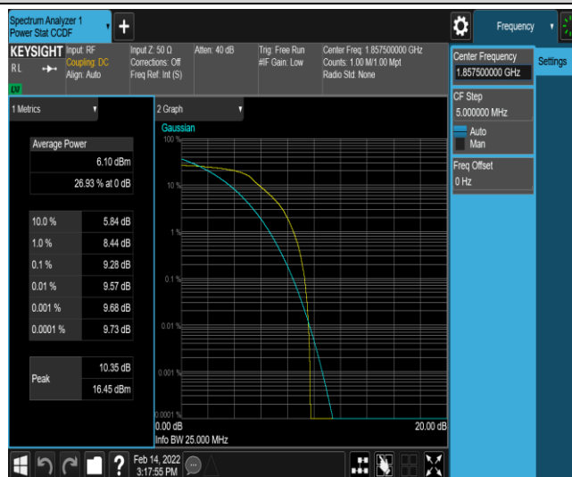
Band2-15MHz-QPSK-18675-6-0-Low-9.28-<=13-PASS
