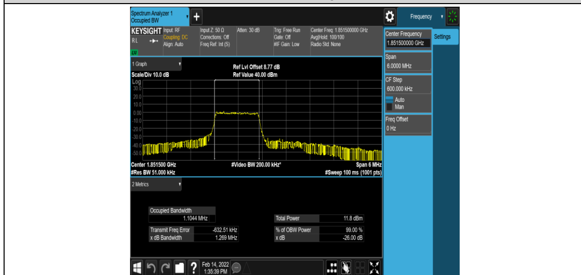
Band2-3MHz-16QAM-18615-6-0-Low-1.1044-1.269-PASS
