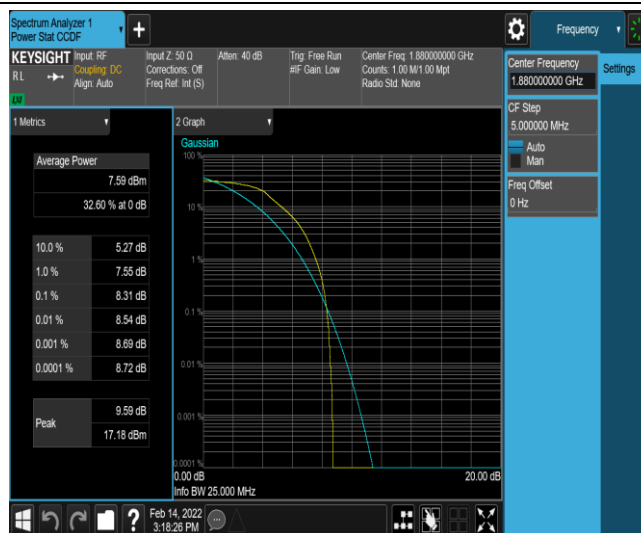
Band2-15MHz-16QAM-18900-6-0-Low-8.31-&lt;=13-PASS
