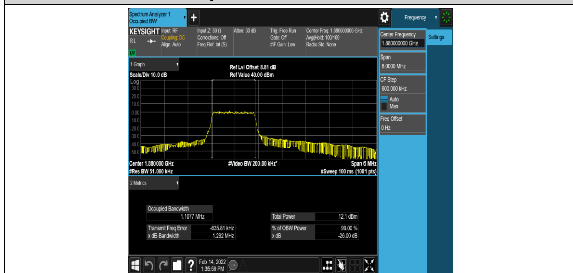
Band2-3MHz-QPSK-18900-6-0-Low-1.1077-1.292-PASS
