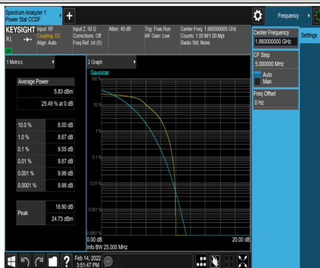
Band2-20MHz-QPSK-18700-6-0-Low-9.55-&lt;=13-PASS
