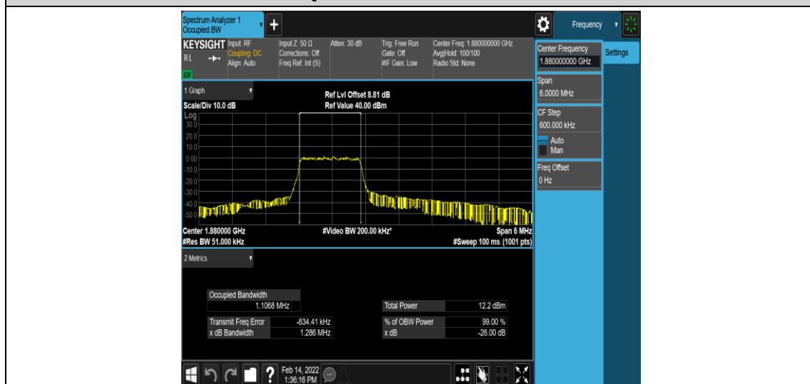
Band2-3MHz-16QAM-18900-6-0-Low-1.1068-1.286-PASS
