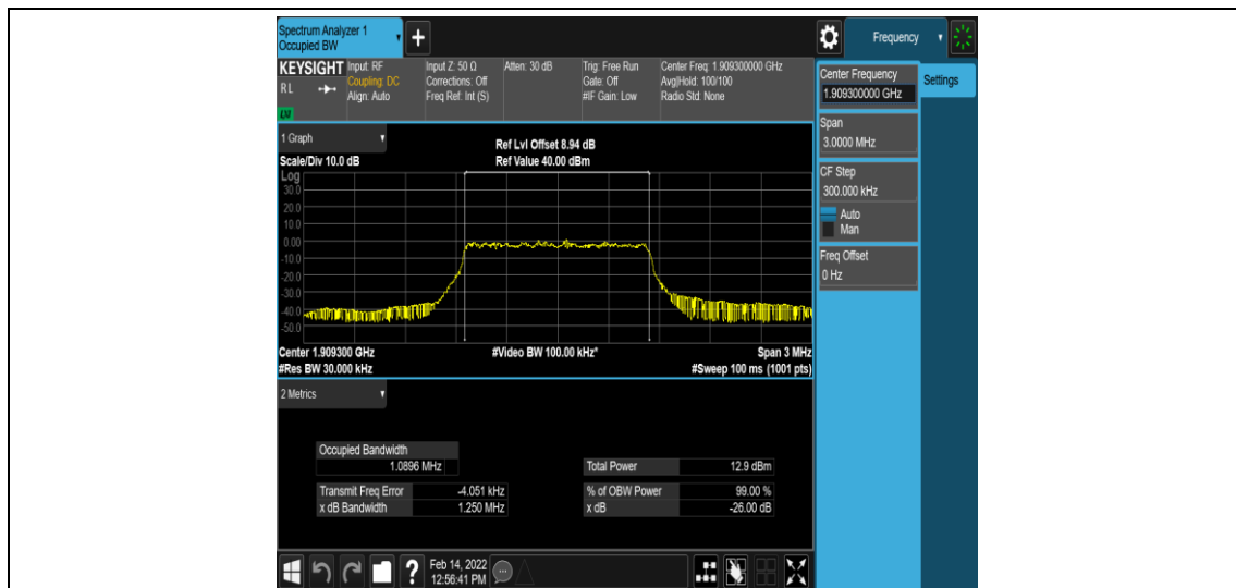
Band2-1.4MHz-16QAM-19193-6-0-High-1.0896-1.250-PASS
