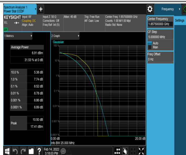
Band2-15MHz-16QAM-18675-6-0-Low-8.52-<=13-PASS
