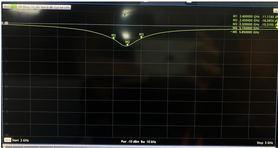
Figure 4.Return Loss
