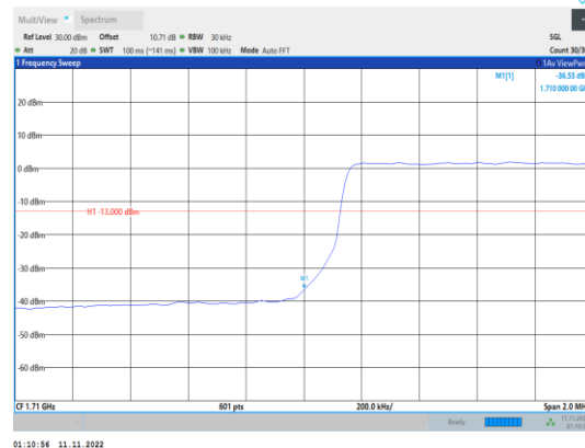
Band66-3MHz-16QAM-131987-15RB#0
