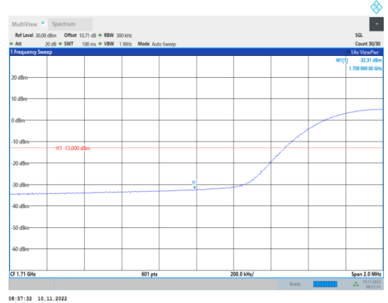
Band66-15MHz-16QAM-132047-75RB#0
