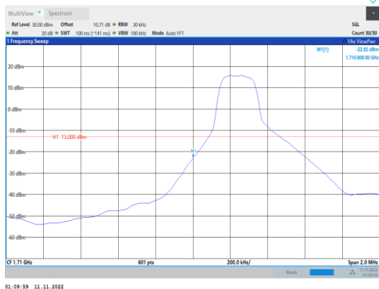
Band66-3MHz-QPSK-131987-1RB#0
