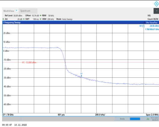
Band66-5MHz-QPSK-132647-25RB#0
