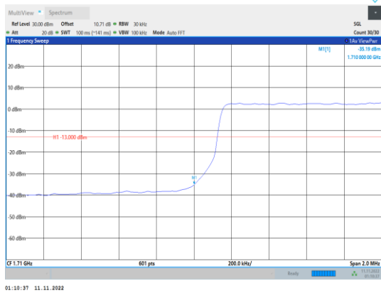
Band66-3MHz-QPSK-131987-15RB#0
