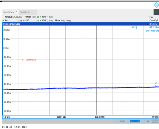
Band5-4132-1000~3000MHz
