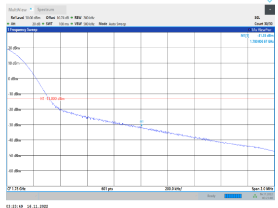
Band66-20MHz-64QAM-132572-1RB#99
