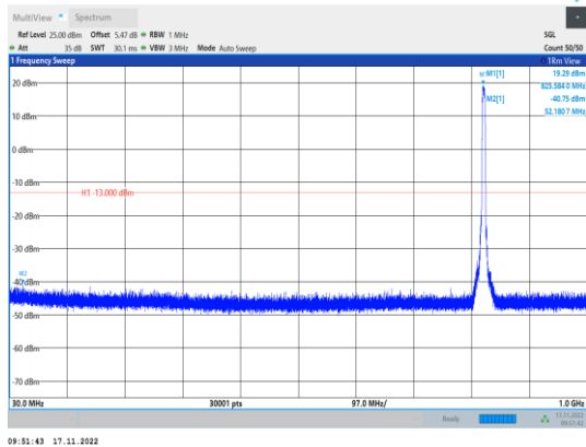
Band5-4132-30~1000MHz
