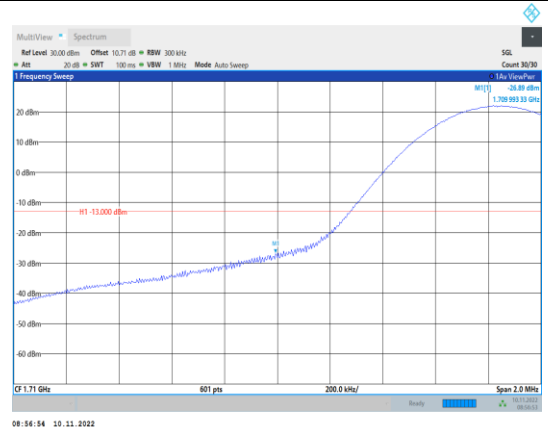
Band66-15MHz-16QAM-132047-1RB#0
