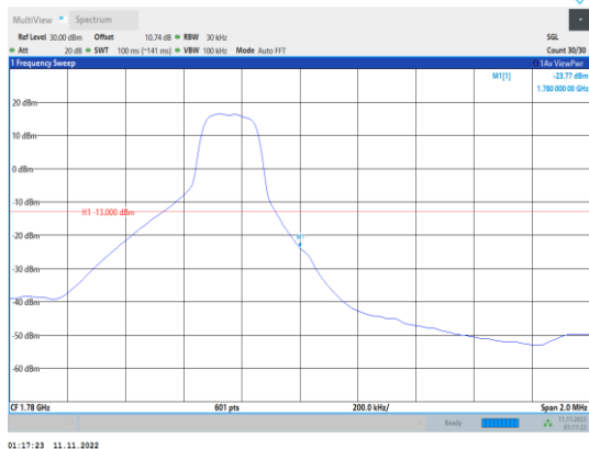
Band66-3MHz-QPSK-132657-1RB#14
