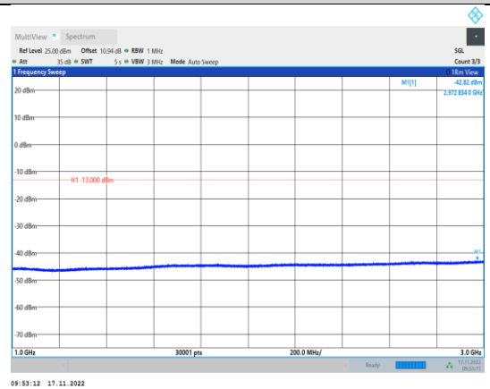
Band5-4182-1000~3000MHz
