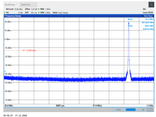
Band5-4182-30~1000MHz
