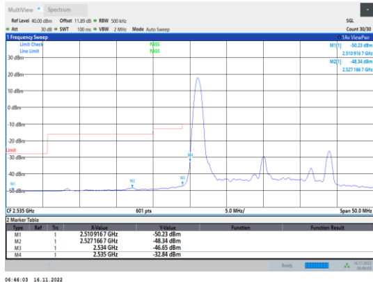
Band41-20MHz-64QAM-40140-1RB#0
