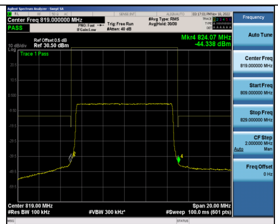
Band26-10MHz-QPSK-26740 Left-50RB#0
