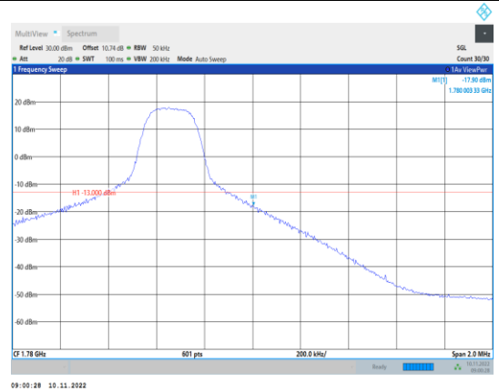
Band66-5MHz-16QAM-132647-1RB#24
