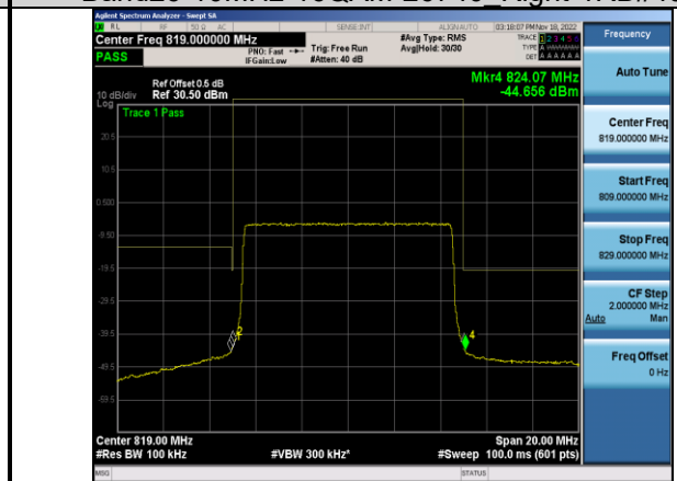
Band26-10MHz-16QAM-26740 Right-50RB#0
