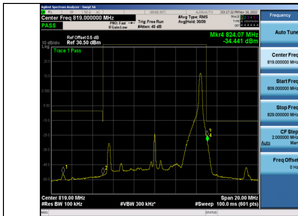
Band26-10MHz-QPSK-26740 Right-1RB#49
