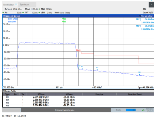
Band41-20MHz-16QAM-41140-100RB#0
