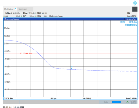
Band66-15MHz-64QAM-132597-75RB#0
