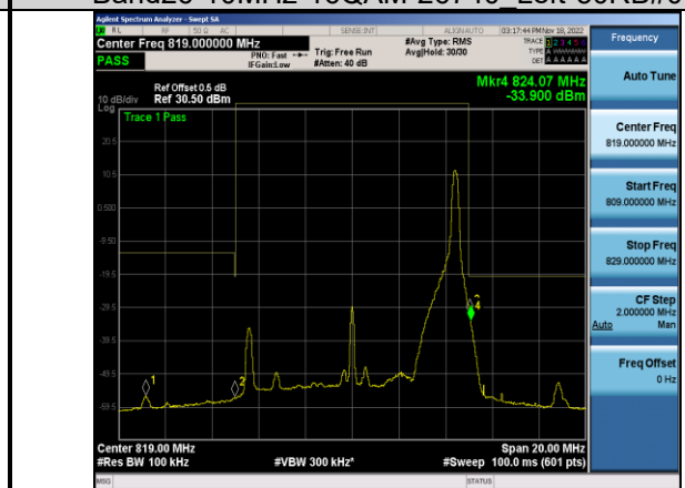
Band26-10MHz-16QAM-26740 Right-1RB#49
