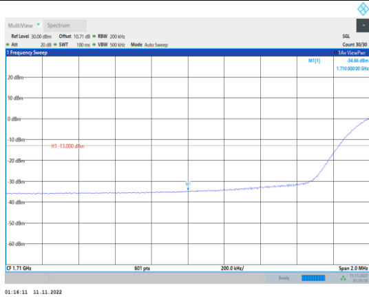
Band66-20MHz-QPSK-132072-100RB#0
