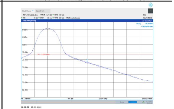
Band66-10MHz-QPSK-132622-1RB#49
