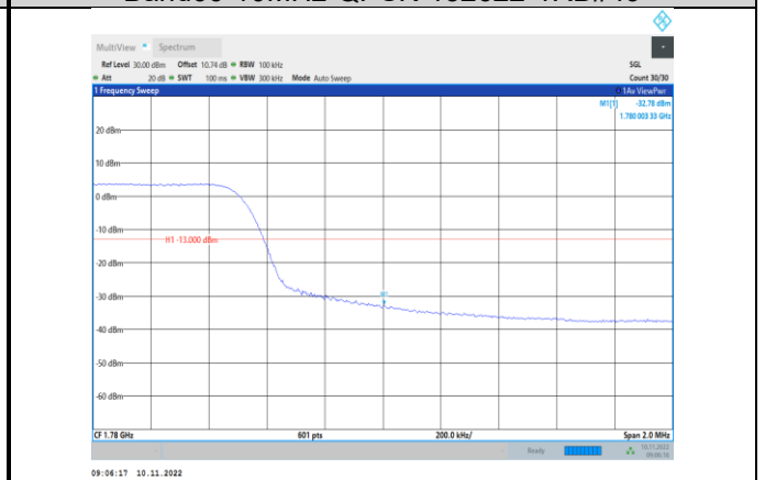
Band66-10MHz-QPSK-132622-50RB#0
