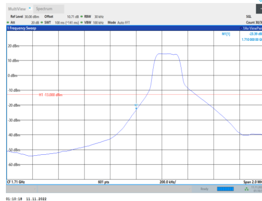
Band66-3MHz-16QAM-131987-1RB#0
