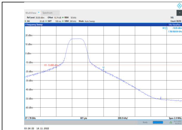
Band66-5MHz-64QAM-132647-1RB#24
