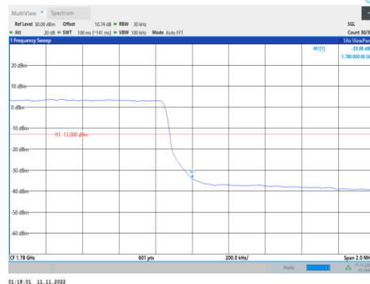
Band66-3MHz-QPSK-132657-15RB#0
