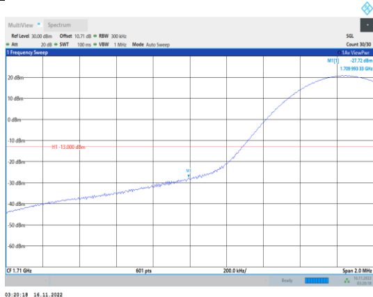
Band66-15MHz-64QAM-132047-1RB#0
