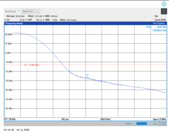
Band66-15MHz-64QAM-132597-1RB#74
