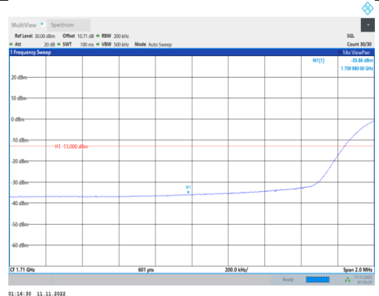
Band66-20MHz-16QAM-132072-100RB#0
