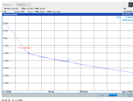
Band66-20MHz-16QAM-132572-1RB#99
