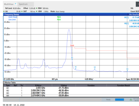
Band41-20MHz-64QAM-41140-1RB#99
