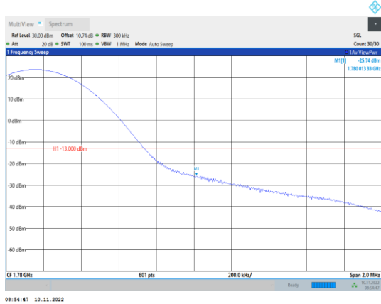
Band66-15MHz-QPSK-132597-1RB#74
