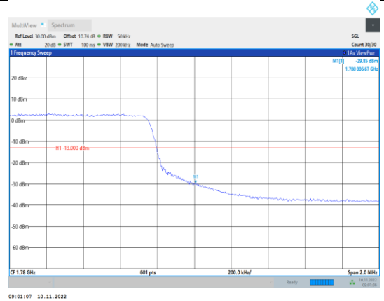
Band66-5MHz-16QAM-132647-25RB#0
