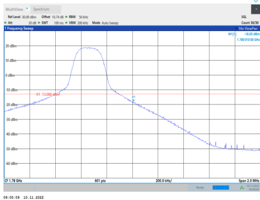
Band66-5MHz-QPSK-132647-1RB#24
