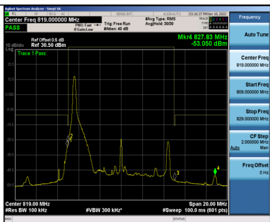
Band26-10MHz-QPSK-26740 Left-1RB#0
