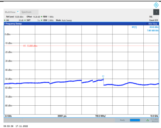
Band5-4182-3000~10000MHz
