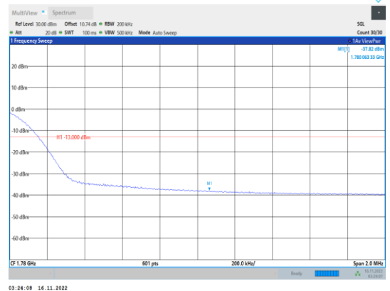
Band66-20MHz-64QAM-132572-100RB#0
