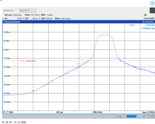
Band66-5MHz-16QAM-131997-1RB#0
