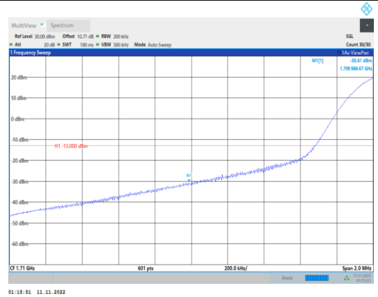
Band66-20MHz-16QAM-132072-1RB#0
