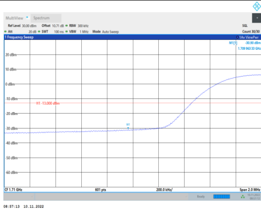
Band66-15MHz-QPSK-132047-75RB#0
