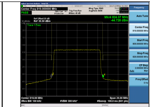
Band26-10MHz-16QAM-26740 Left-50RB#0
