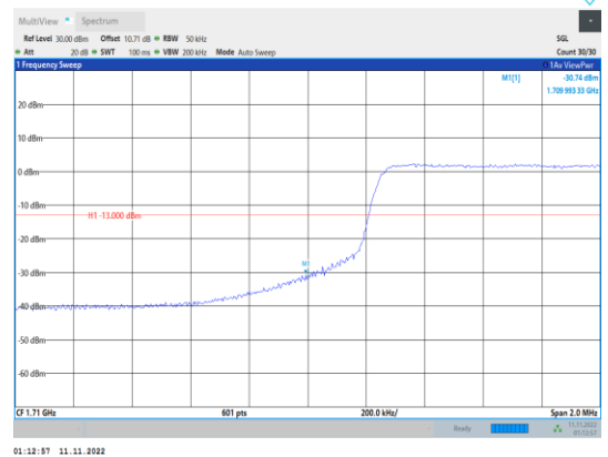
Band66-5MHz-16QAM-131997-25RB#0
