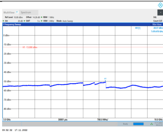
Band5-4132-3000~10000MHz
