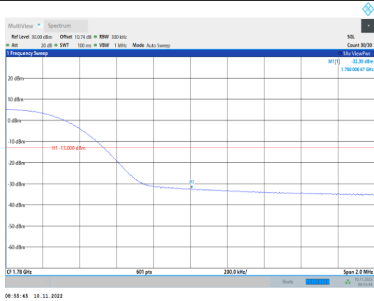
Band66-15MHz-16QAM-132597-75RB#0
