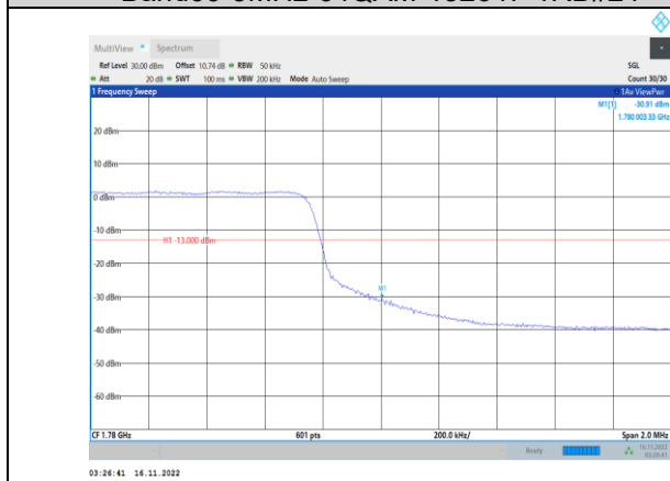
Band66-5MHz-64QAM-132647-25RB#0
