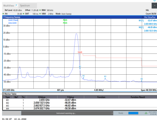
Band41-20MHz-16QAM-41140-1RB#99
