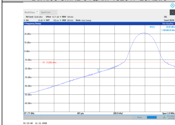
Band66-10MHz-QPSK-132022-1RB#0
