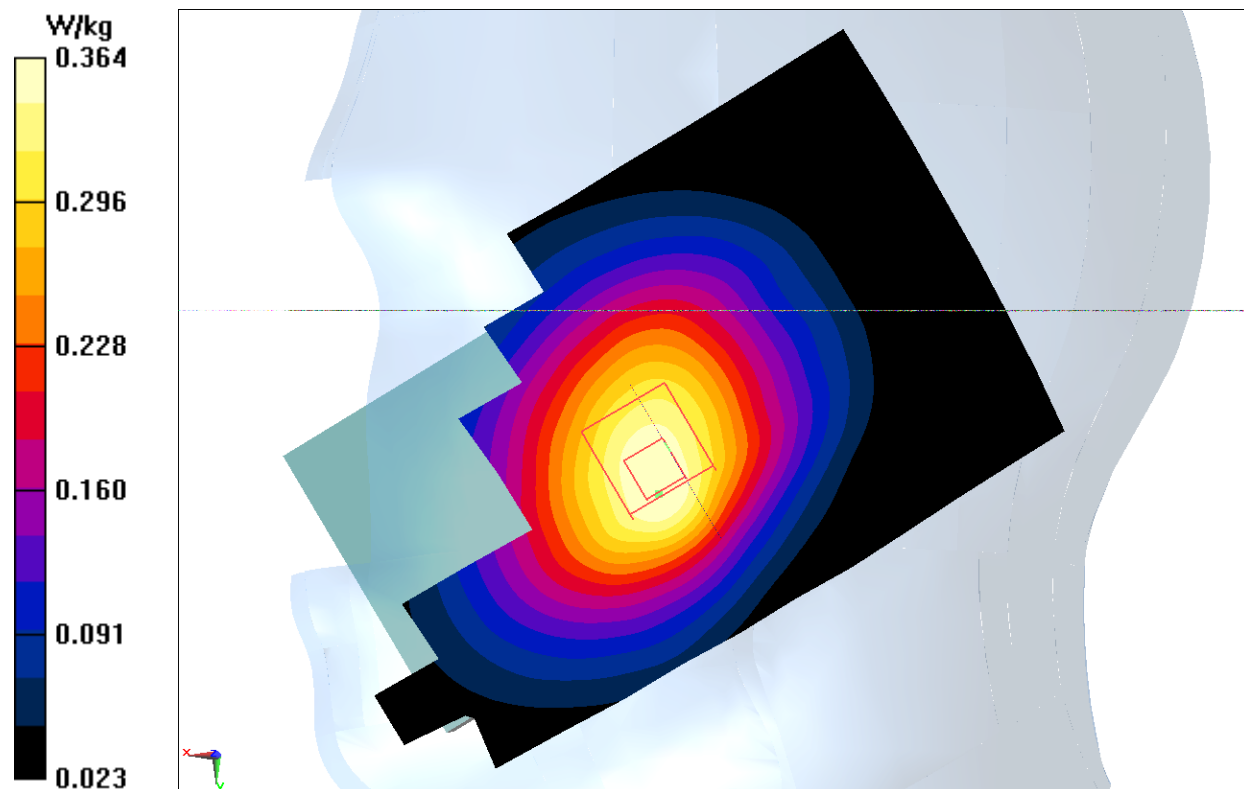
Fig.I.1 850MHz
