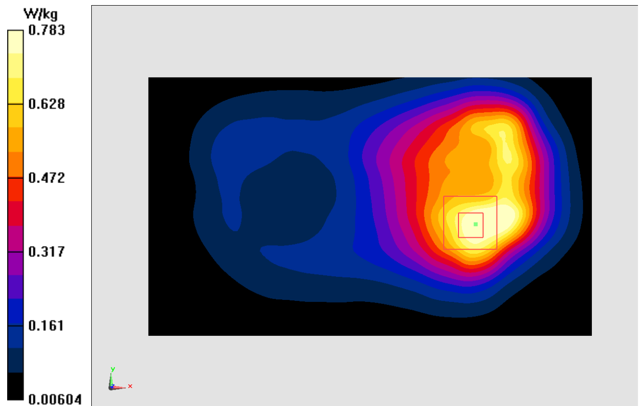
Fig.I.7 LTE Band2
