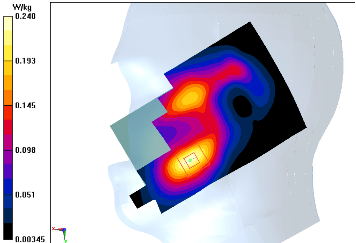
Fig.I.2 1900 MHz
