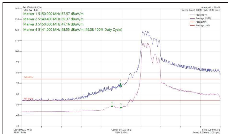
Figure 174 - 802.11ax HE80, RU 106-53, SDM, Core 0 + Core 1 - 5210 MHz Band Edge Frequency 5150 MHz
