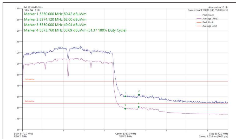
Figure 187 - 802.11ac VHT160, SISO, Core 0 - 5250 MHz Band Edge Frequency 5350 MHz
