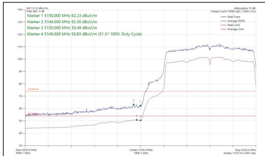
Figure 154 - 802.11ac VHT80, SISO, Core 1 - 5210 MHz Band Edge Frequency 5150 MHz
