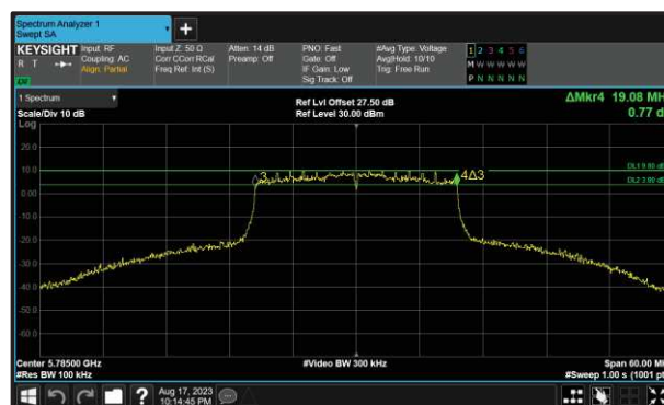
Figure 229 - 802.11ax HE20 SU Maximum 6 dB EBW
