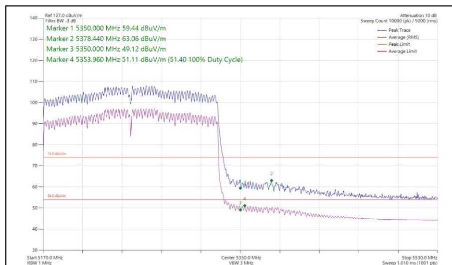
Figure 206 - 802.11ax HE160, SU, CDD, Core 0 + Core 1 - 5250 MHz Band Edge Frequency 5350 MHz
