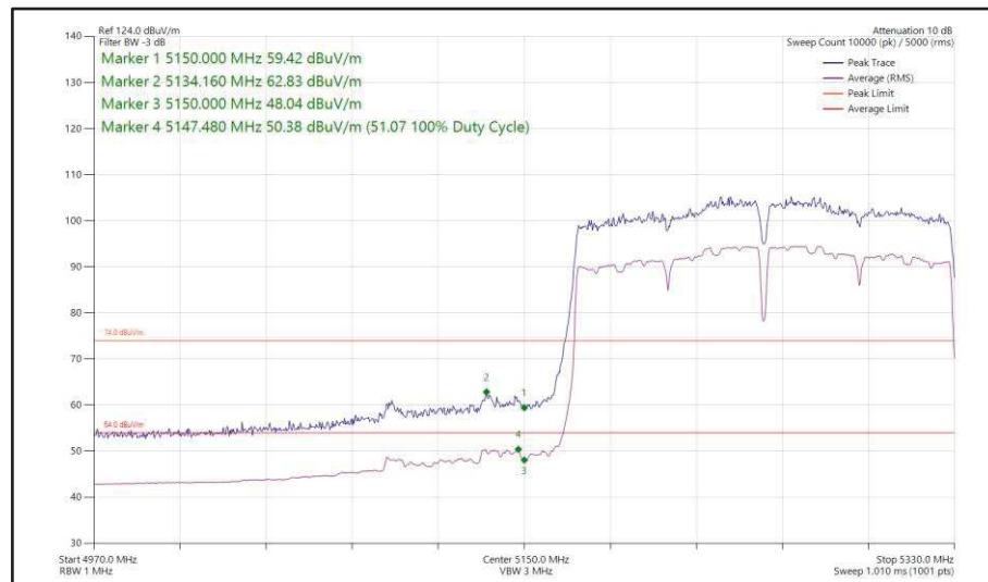
Figure 193 - 802.11ac VHT160, SISO, Core 1 - 5250 MHz Band Edge Frequency 5150 MHz
