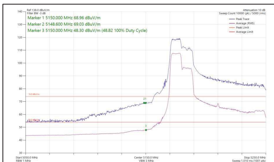
Figure 156 - 802.11ax HE80, RU 106-53, SISO, Core 1 - 5210 MHz Band Edge Frequency 5150 MHz
