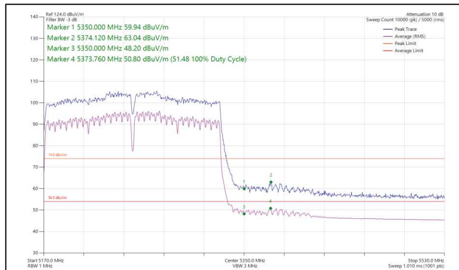
Figure 205 - 802.11ac VHT160, CDD, Core 0 + Core 1 - 5250 MHz Band Edge Frequency 5350 MHz
