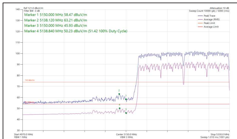
Figure 202 - 802.11ac VHT160, CDD, Core 0 + Core 1 - 5250 MHz Band Edge Frequency 5150 MHz
