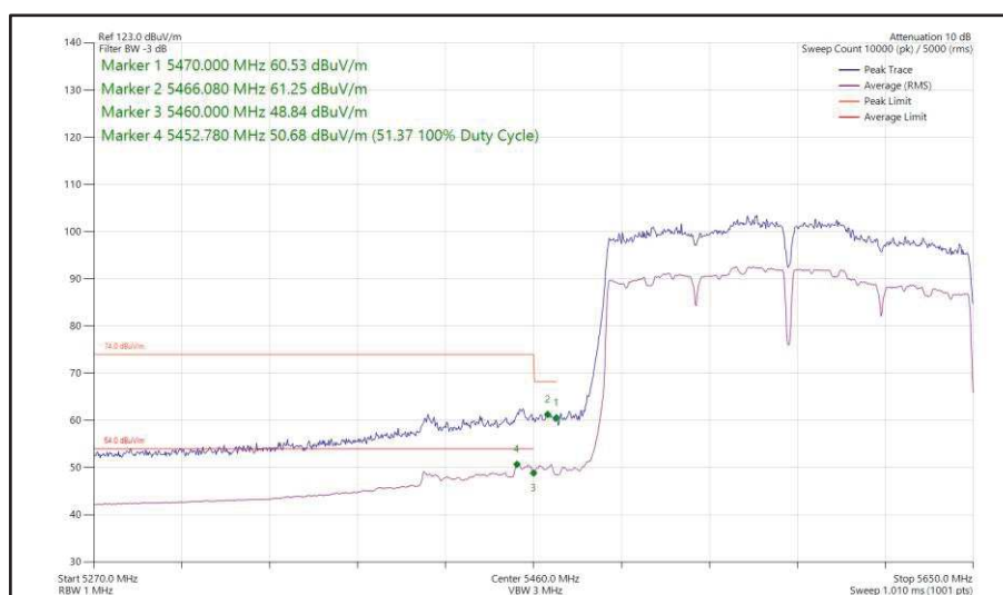
Figure 190 - 802.11ac VHT160, SISO, Core 0 - 5570 MHz Band Edge Frequency 5460 MHz
