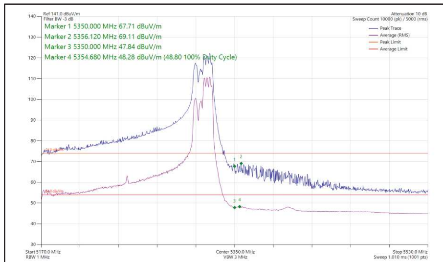
Figure 207 - 802.11ax HE160, RU 106-60, CDD, Core 0 + Core 1 - 5250 MHz Band Edge Frequency 5350 MHz
