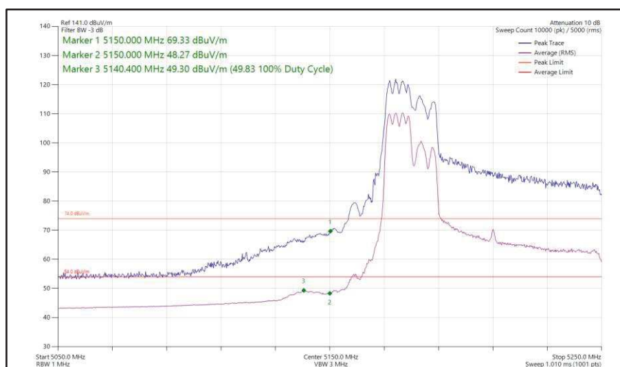
Figure 165 - 802.11ax HE80, RU 106-53, CDD, Core 0 + Core 1 - 5210 MHz Band Edge Frequency 5150 MHz
