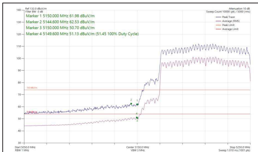
Figure 164 - 802.11ax HE80, SU, CDD, Core 0 + Core 1 - 5210 MHz Band Edge Frequency 5150 MHz
