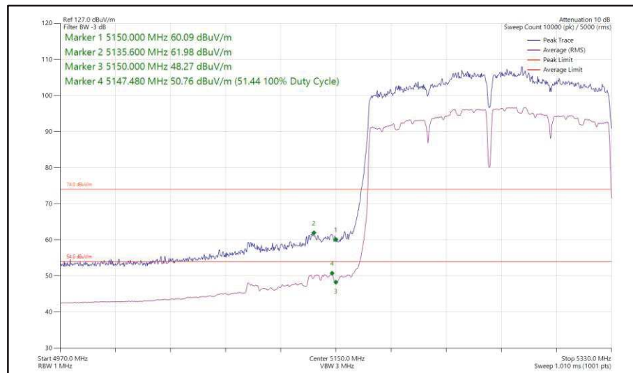
Figure 184 - 802.11ac VHT160, SISO, Core 0 - 5250 MHz Band Edge Frequency 5150 MHz
