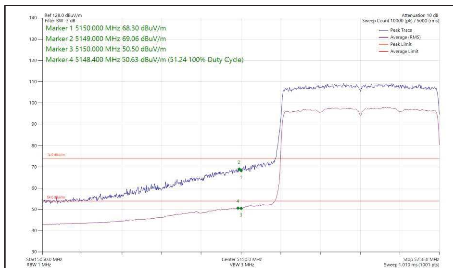
Figure 155 - 802.11ax HE80, SU, SISO, Core 1 - 5210 MHz Band Edge Frequency 5150 MHz
