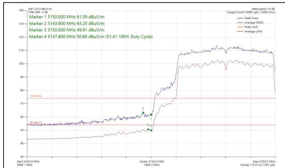
Figure 172 - 802.11ac VHT80, SDM, Core 0 + Core 1 - 5210 MHz Band Edge Frequency 5150 MHz
