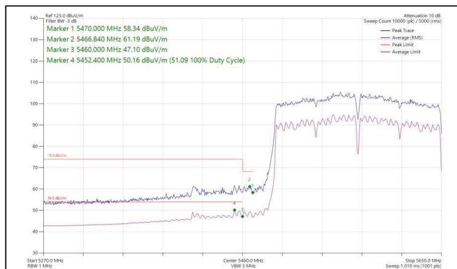
Figure 217 - 802.11ac VHT160, SDM, Core 0 + Core 1 - 5570 MHz Band Edge Frequency 5460 MHz
