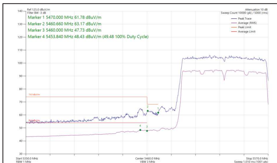
Figure 151 - 802.11ac VHT80, SISO, Core 0 - 5530 MHz Band Edge Frequency 5460 MHz
