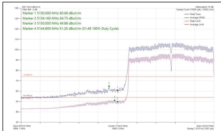
Figure 203 - 802.11ax HE160, SU, CDD, Core 0 + Core 1 - 5250 MHz Band Edge Frequency 5150 MHz
