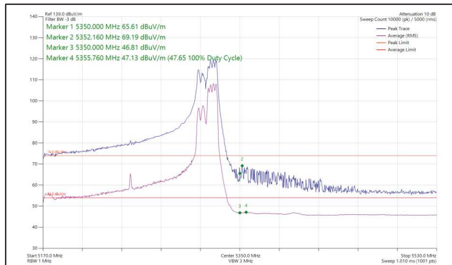
Figure 216 - 802.11ax HE160, RU 106-60, SDM, Core 0 + Core 1 - 5250 MHz Band Edge Frequency 5350 MHz
