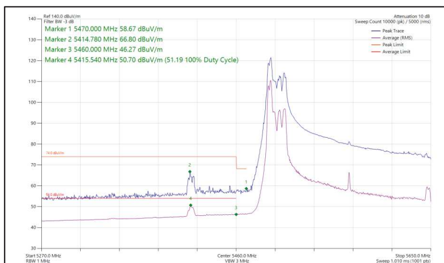
Figure 219 - 802.11ax HE160, RU 52-37, SDM, Core 0 + Core 1 - 5570 MHz Band Edge Frequency 5460 MHz
