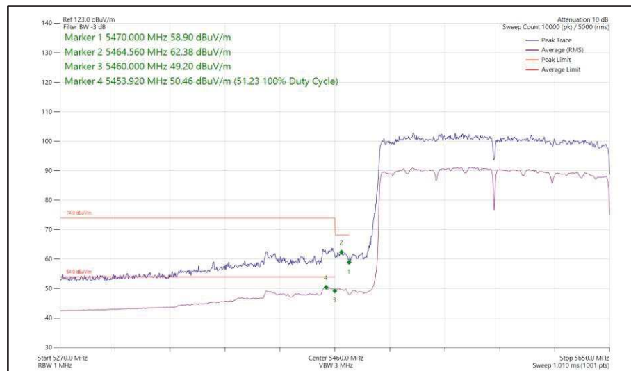
Figure 191 - 802.11ax HE160, SU, SISO, Core 0 - 5570 MHz Band Edge Frequency 5460 MHz
