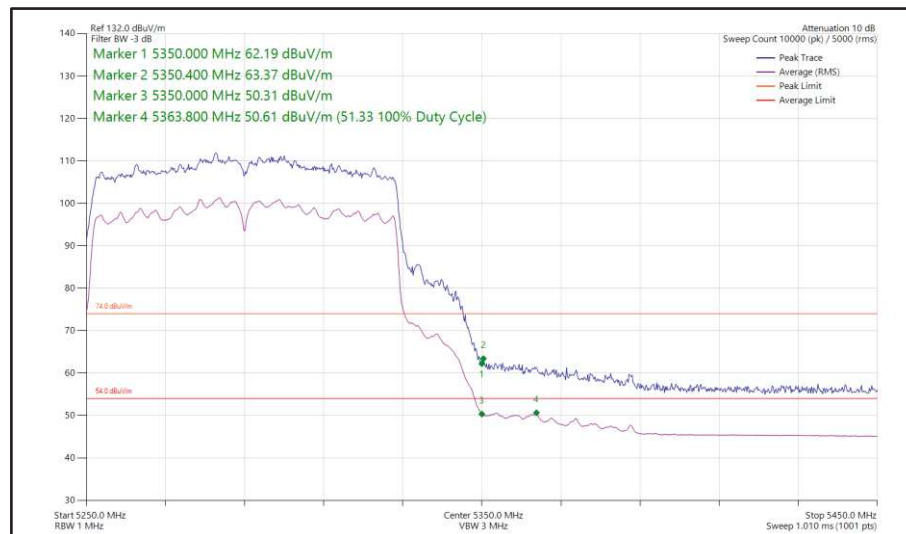
Figure 175 - 802.11ac VHT80, SDM, Core 0 + Core 1 - 5290 MHz Band Edge Frequency 5350 MHz
