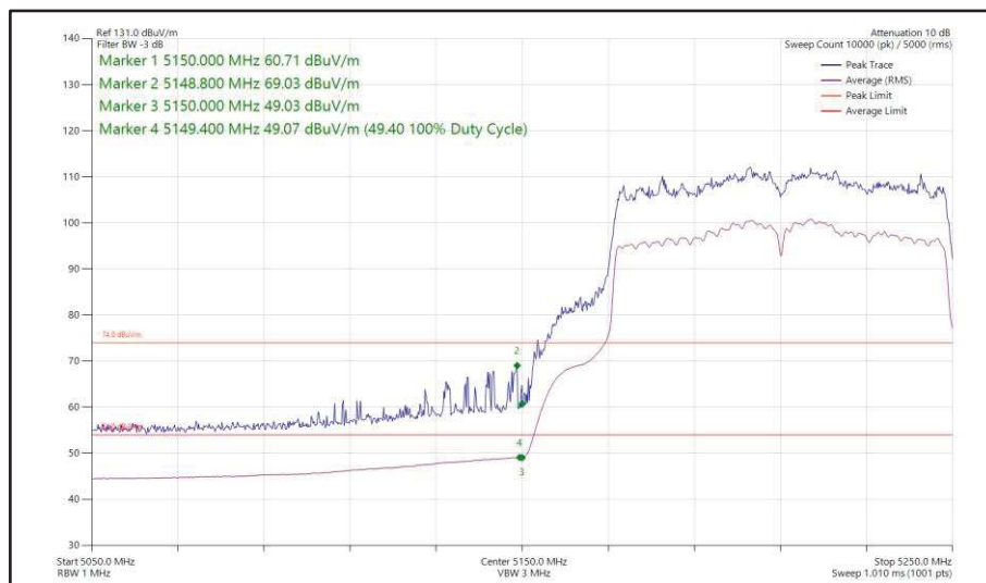
Figure 181 - 802.11ac VHT80, TxBF, Core 0 + Core 1 - 5210 MHz Band Edge Frequency 5150 MHz
