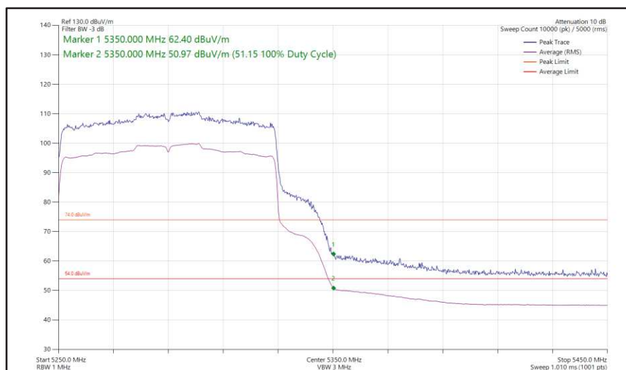
Figure 149 - 802.11ax HE80, SU, SISO, Core 0 - 5290 MHz Band Edge Frequency 5350 MHz
