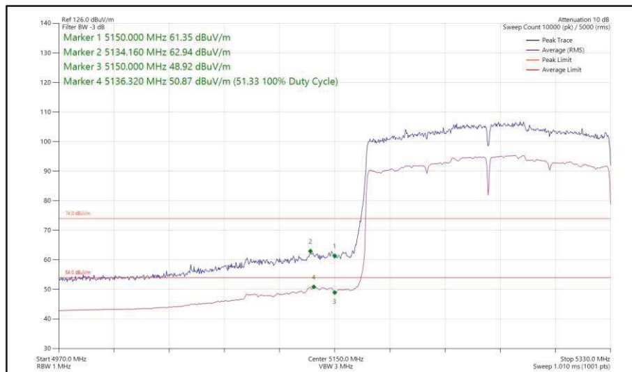
Figure 194 - 802.11ax HE160, SU, SISO, Core 1 - 5250 MHz Band Edge Frequency 5150 MHz
