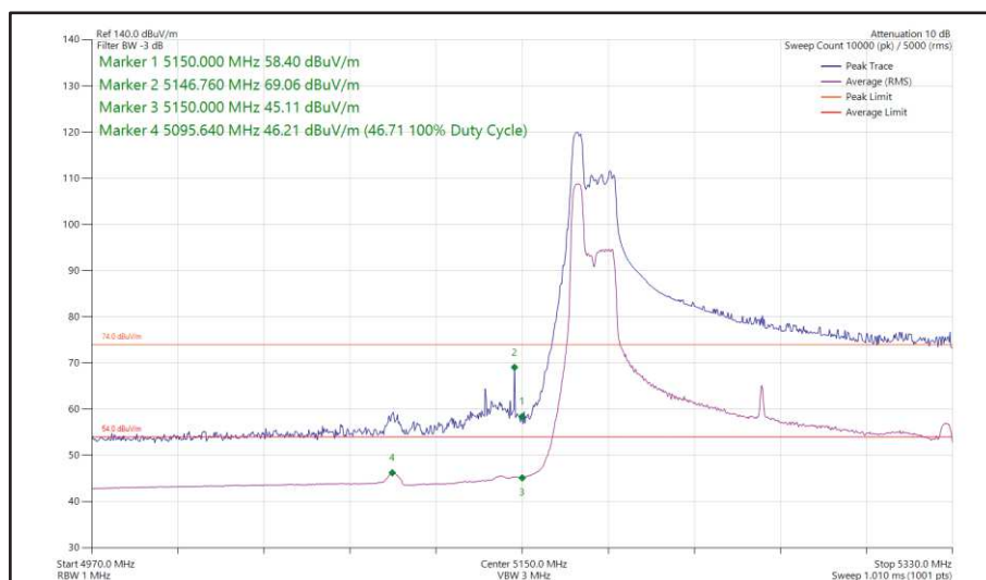
Figure 195 - 802.11ax HE160, RU 52-37, SISO, Core 1 - 5250 MHz Band Edge Frequency 5150 MHz
