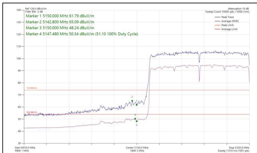
Figure 185 - 802.11ax HE160, SU, SISO, Core 0 - 5250 MHz Band Edge Frequency 5150 MHz
