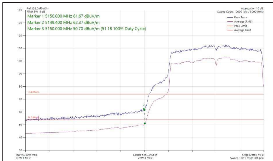
Figure 145 - 802.11ac VHT80, SISO, Core 0 - 5210 MHz Band Edge Frequency 5150 MHz
