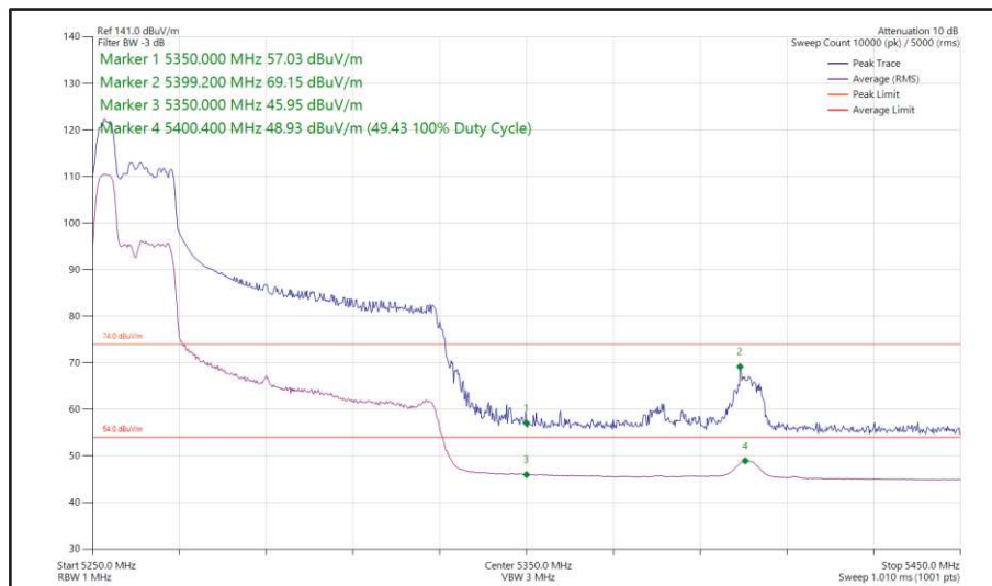
Figure 150 - 802.11ax HE80, RU 52-37, SISO, Core 0 - 5290 MHz Band Edge Frequency 5350 MHz
