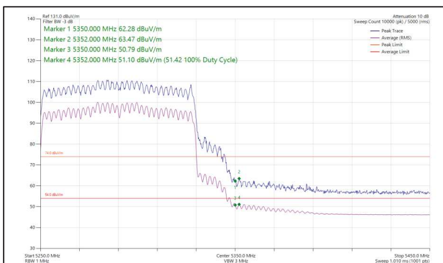
Figure 167 - 802.11ax HE80, SU, CDD, Core 0 + Core 1 - 5290 MHz Band Edge Frequency 5350 MHz
