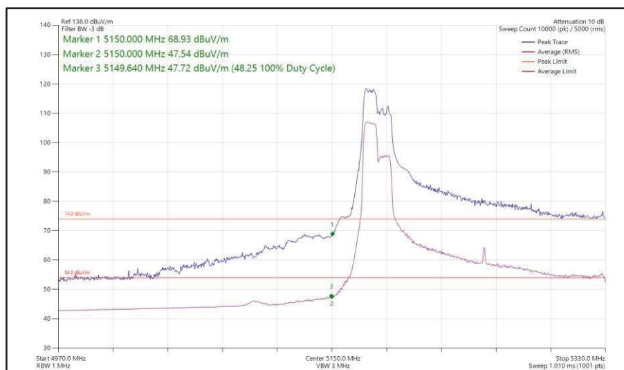
Figure 186 - 802.11ax HE160, RU 106-53, SISO, Core 0 - 5250 MHz Band Edge Frequency 5150 MHz
