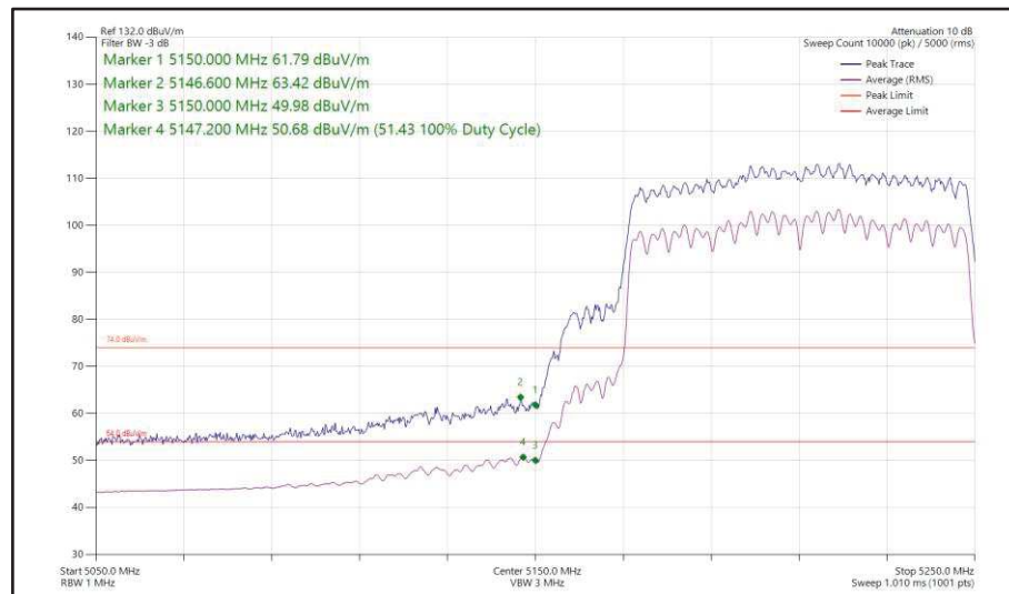
Figure 163 - 802.11ac VHT80, CDD, Core 0 + Core 1 - 5210 MHz Band Edge Frequency 5150 MHz
