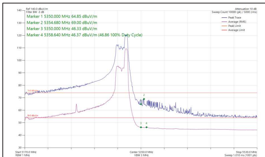
Figure 189 - 802.11ax HE160, RU 52-52, SISO, Core 0 - 5250 MHz Band Edge Frequency 5350 MHz
