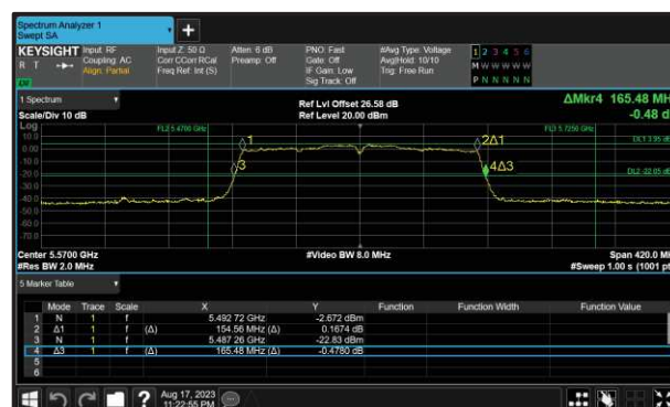
Figure 271 - 802.11ac VHT160 Maximum 99% OBW
