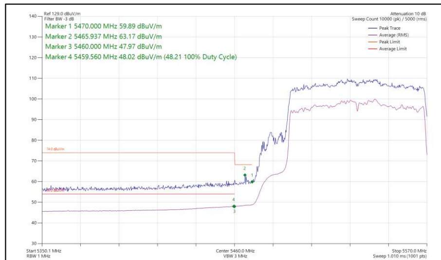
Figure 183 - 802.11ac VHT80, TxBF, Core 0 + Core 1 - 5530 MHz Band Edge Frequency 5460 MHz
