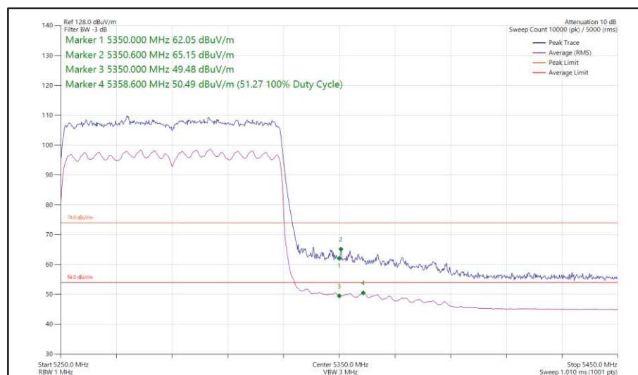
Figure 176 - 802.11ax HE80, SU, SDM, Core 0 + Core 1 - 5290 MHz Band Edge Frequency 5350 MHz
