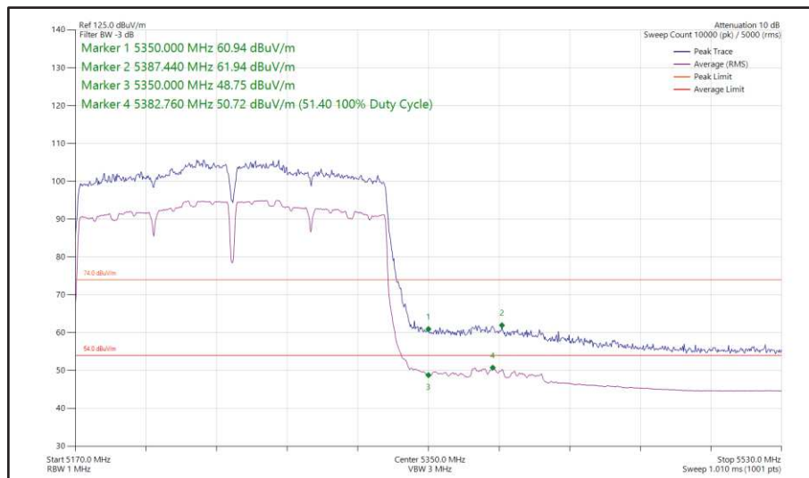
Figure 196 - 802.11ac VHT160, SISO, Core 1 - 5250 MHz Band Edge Frequency 5350 MHz
