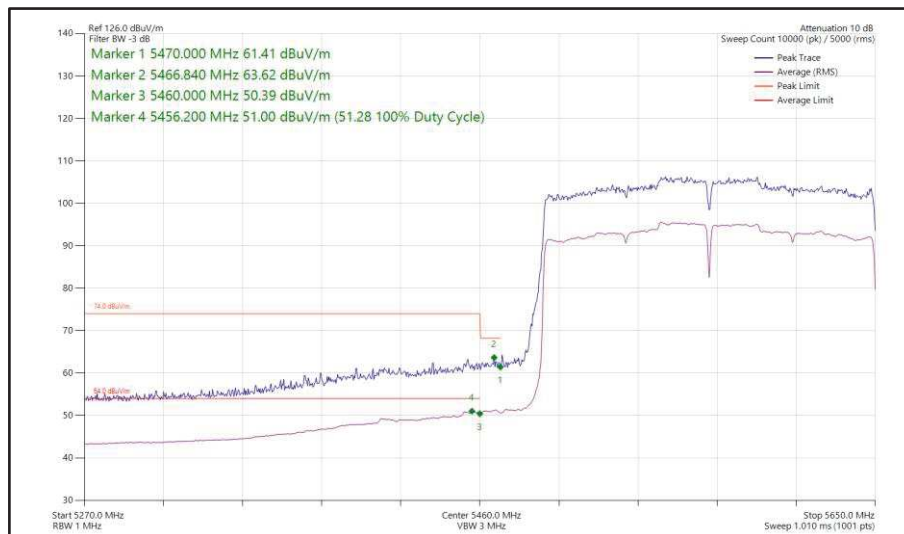
Figure 200 - 802.11ax HE160, SU, SISO, Core 1 - 5570 MHz Band Edge Frequency 5460 MHz
