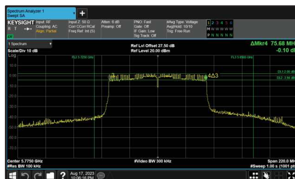
Figure 227 - 802.11ac VHT80 Maximum 6 dB EBW
