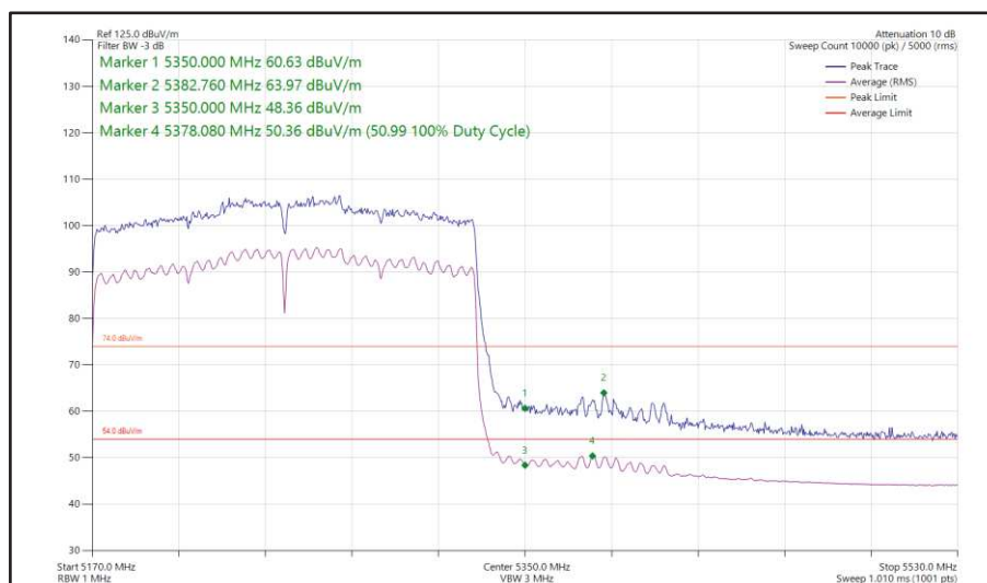
Figure 215 - 802.11ax HE160, SU, SDM, Core 0 + Core 1 - 5250 MHz Band Edge Frequency 5350 MHz
