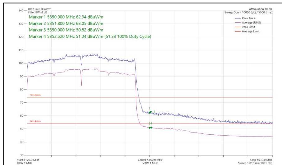
Figure 188 - 802.11ax HE160, SU, SISO, Core 0 - 5250 MHz Band Edge Frequency 5350 MHz
