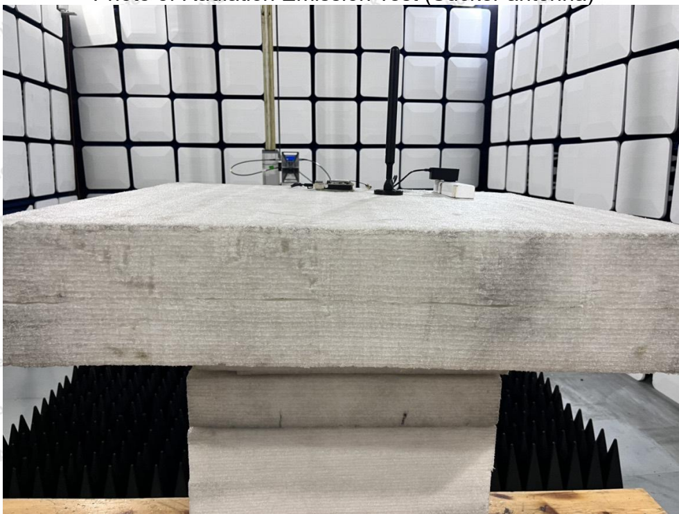
Photo of Radiation Emission Test (Sucker antenna)
