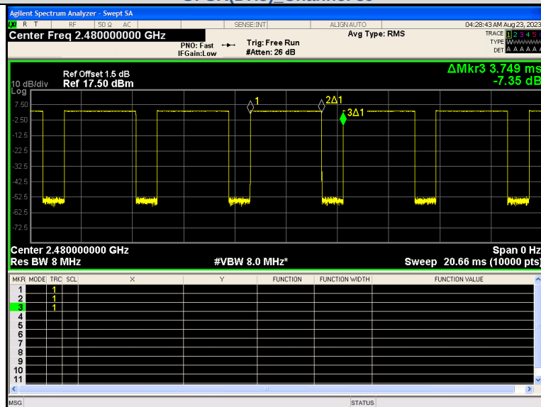
GFSK(DH5)_Channel 78
