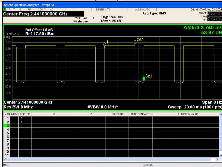
8DPSK(3-DH5) Channel 39
