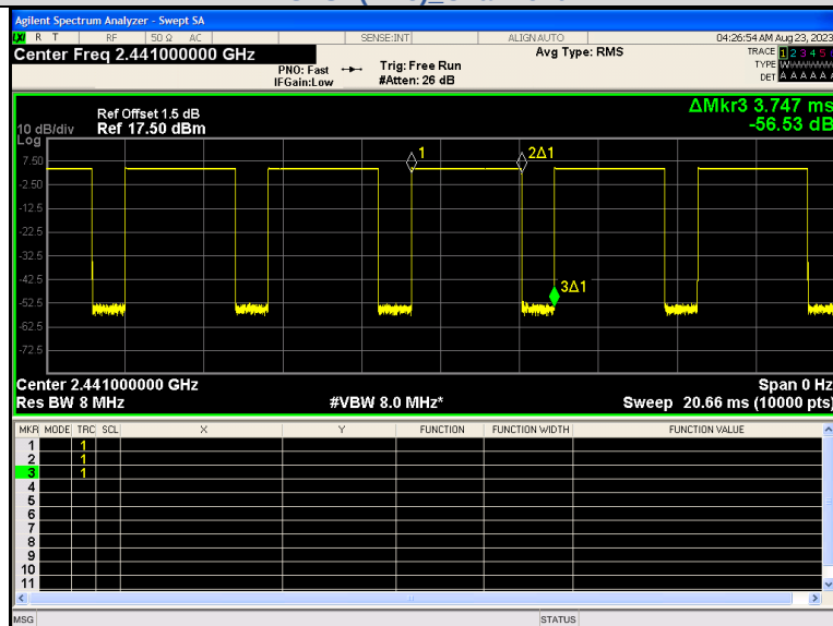
GFSK(DH5)_Channel 39
