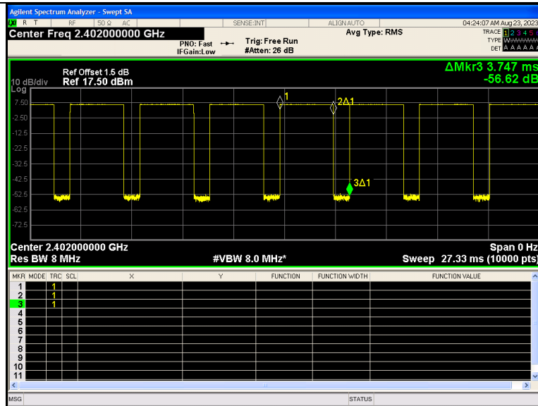
GFSK(DH5)_Channel 0
