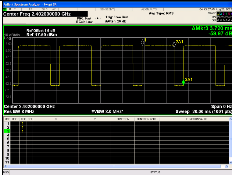
8DPSK(3-DH5) Channel 0
