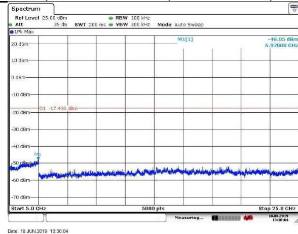
Spurious Emission (5GHz –25GHz)
