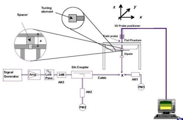
Fig 8.3.1 System Performance Check Setup
