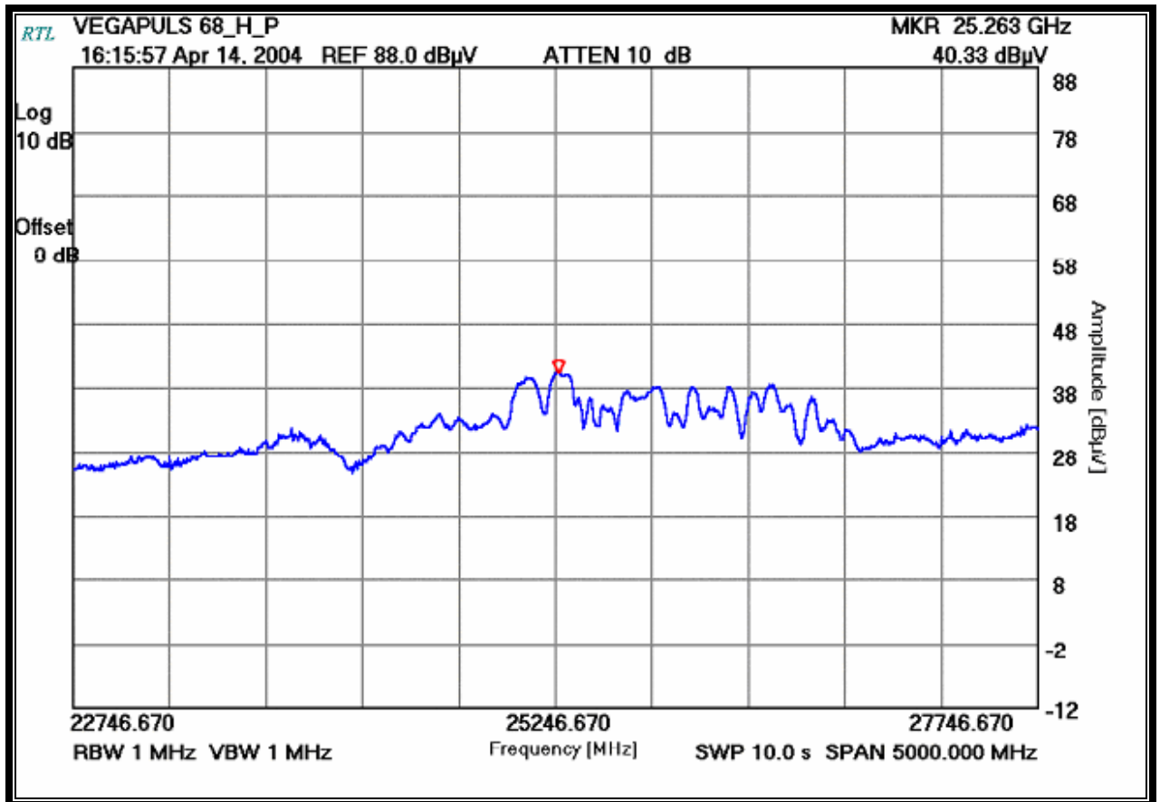
PLOT 6-2 EUT 19.5 DBI HORN ANTENNA 100% DUTY CYCLE PEAK MODE
