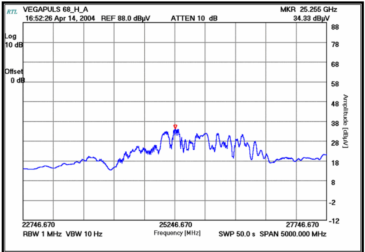
PLOT 6-3 EUT 19.5 DBI HORN ANTENNA 100% DUTY CYCLE AVERAGE MODE
